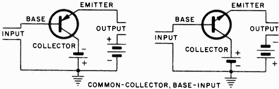
COMMON-COLLECTOR, BASE-INPUT
