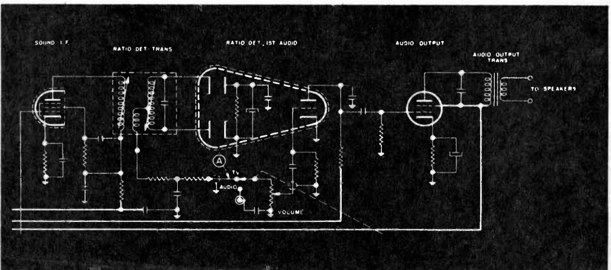
Circuit diagram (below) of typical TV sound.
