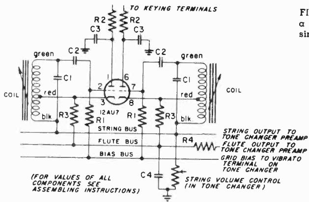
Two-note tone generator schematic is shown above.
