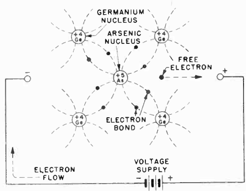
FIG. 2. When germanium is doped with a valence-5 material, an electron flow can take place as is the case in an ordinary electron conductor.
