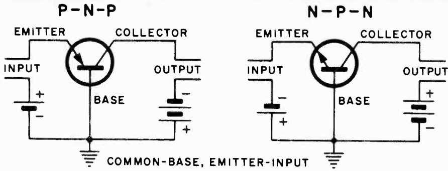
COMMON-BASE, EMITTER-INPUT
