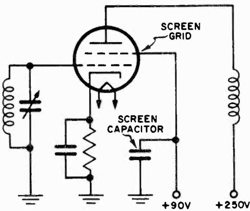
FIG. 7. Screen grid in the tetrode tube reduces interelectrode capacitance by a shielding effect.
