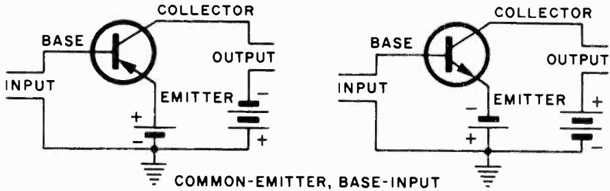
COMMON-EMITTER, BASE-INPUT
