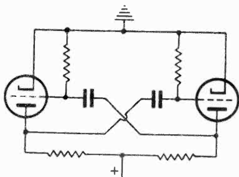
FIG. 5. The free-running multivibrator produces a wide range of frequencies in a single circuit, simply by varying the value of one component.
