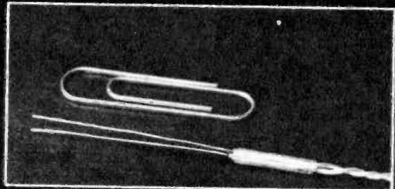
Detecting element (above) can be made by stripping the ends of a pair of wires, keeping them closely spaced.
