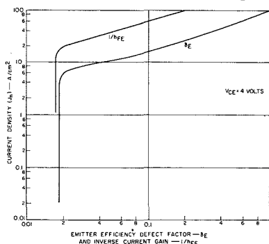
Fig. 7—Emitter-efficiency defect factor.
