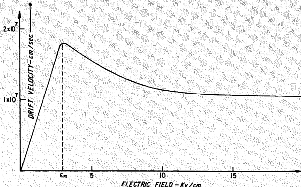
Fig. 6—Drift velocity of conduction electrons in GaAs as a function of electric field.
