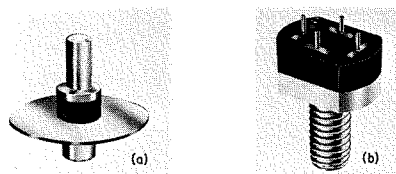
Fig. 2—Photograph of two transistor packages specifically designed for operation at uhf and microwave frequencies: a) coaxial package, b) stripline package.
