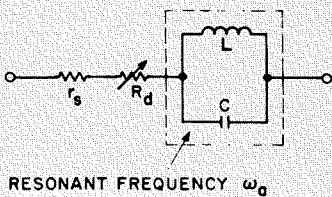
Fig. 5—Small-signal equivalent circuit of a Read avalanche diode.
