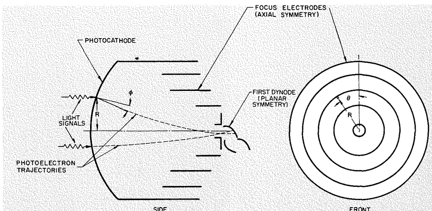
Fig. 2—Side and front views of the photocathode-to-first-dynode region showing parameters used in electron trajectory computations.
