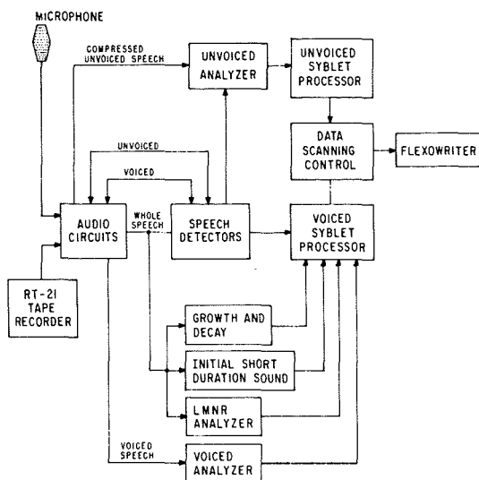
Fig. 1—Block diagram of speech analyzer.
