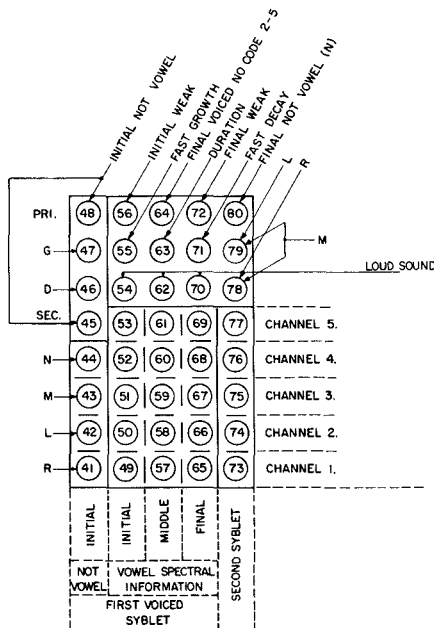
Fig. 2—40-bit digital display, voiced syblet processor.
