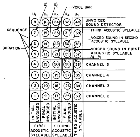
Fig. 3—40-bit digital display, unvoiced syblet processor.
