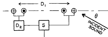
Fig. 2—Schematic arrangement of a higher-order unidirectional microphone; consisting of two first-order gradient microphones, a delay system ( D_2 ) and summing network ( S ).
