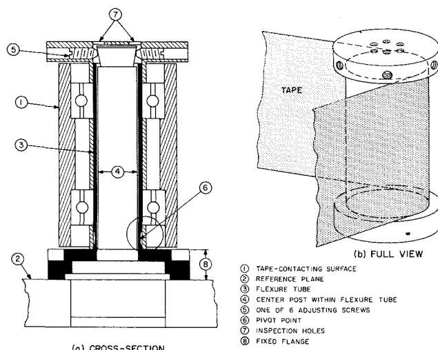
Fig. 2—Adjustable tape-guide roller.
