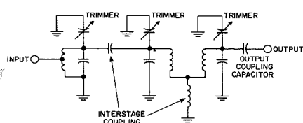
Fig. 5—Circuit diagram of the FD3100 pre-selector.
