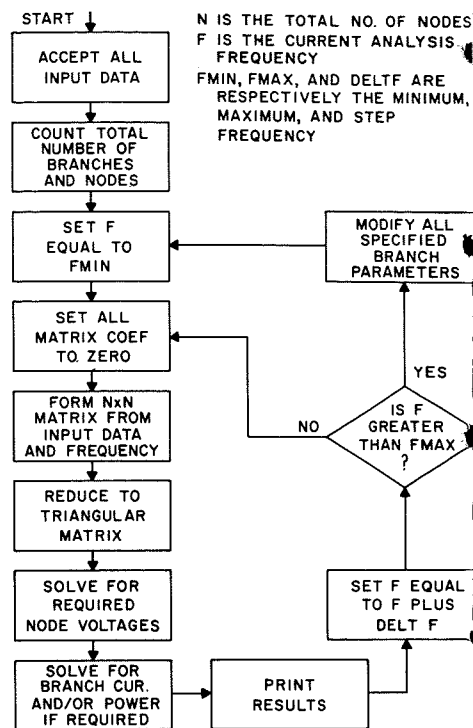
Fig. 4—Block diagram of steady-state circuit analysis program.
