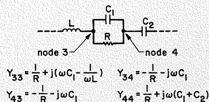
Fig. 2—This section of a circuit is shown with the elements of the corresponding Y-matrix.
