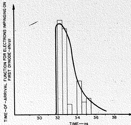
Fig. 7—Predicted time response characteristic for a photocathode illuminated by a beam of small diameter considering only low-energy photoelectron emission.
