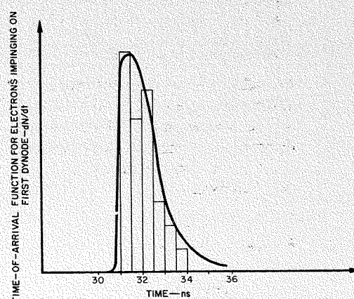
Fig. 8—Predicted time-response characteristic for a photocathode illuminated by a beam of small diameter focused on the axis of symmetry.
