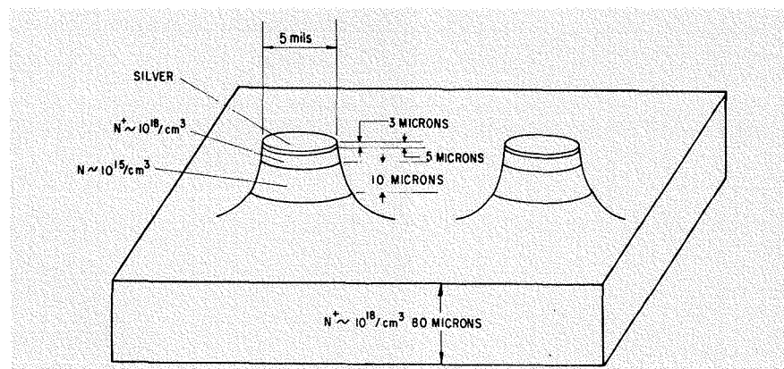
Fig. 8—Sketch of a two-mesa X-band cw transferred-electron oscillator. The mesas are chemically etched from an epitaxial wafer.
