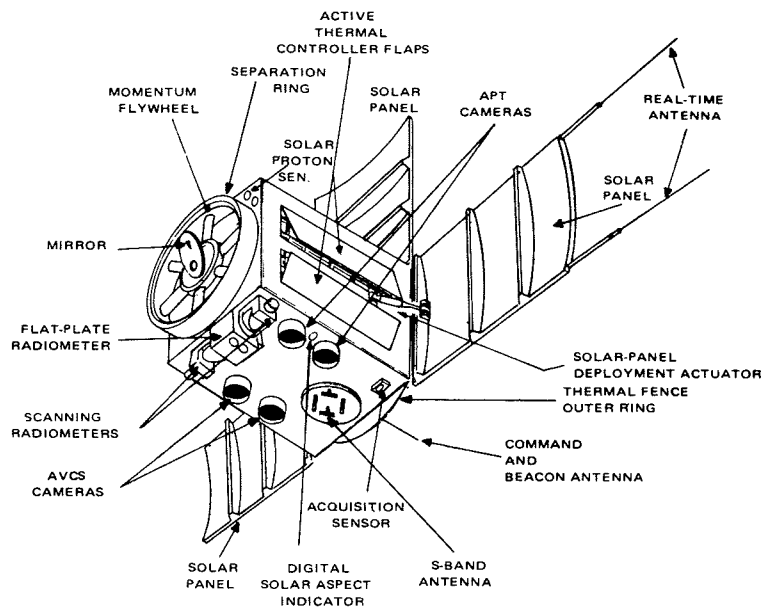
Fig. 7—The TIROS M/ITOS satellite in mission mode.
