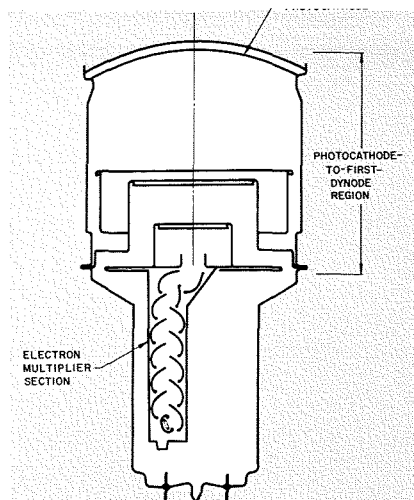
Fig. 1—Photomultiplier tube cross section.
