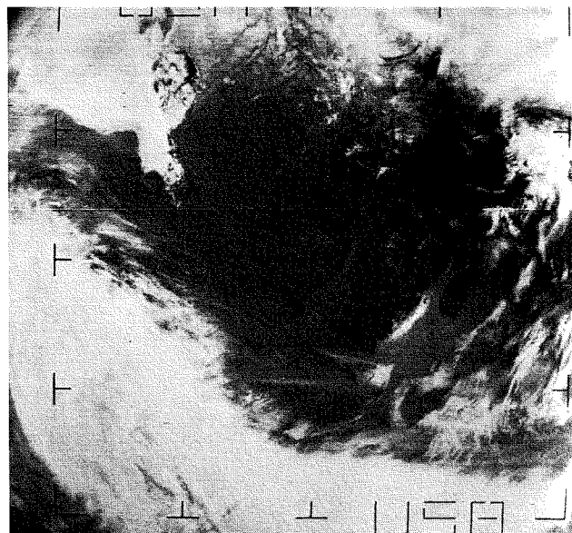
Fig. 4—The one-millionth picture taken by the TIROS series; picture shows the Hudson Bay area and Northern New England on May 27, 1968.
