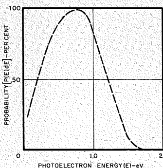
Fig. 5—Method of selecting three equally probable energies from the cumulative probability function.
