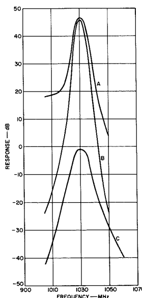
Fig. 6—Bandpass curves for a) FD3101 amplifier alone, c) FD3100 preselector alone, and b) FD2201.
