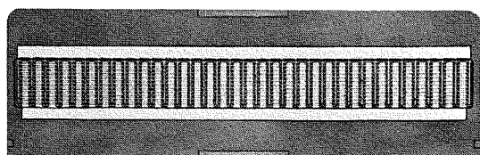
Fig. 1—Photograph showing the 408 emitters of the RCA Dev. No. TA2675 overlay transistor. The dimensions of each emitter are 0.1 mil x 1.4 mils.
