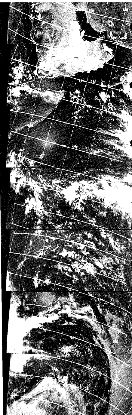
Fig. 3—Portion of an orbital sequence of ESSA 3 television photographs showing Saudi Arabia, Somaliland, and Indian Ocean. (Gridding added by digital computer at the U.S. National Environmental Satellite Center).
