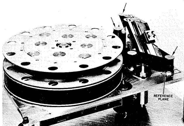
Fig. 1—Magnetic recorder showing tape-guide rollers (arrows).
