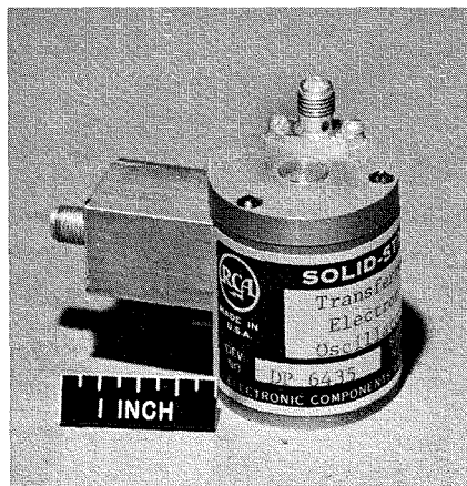
Fig. 9—Photograph of a pulsed 100-watt L-band transferred-electron oscillator.
