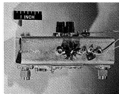
Fig. 3—Photograph of a 20-watt coaxial 700-MHz amplifier using three transistors in parallel.
