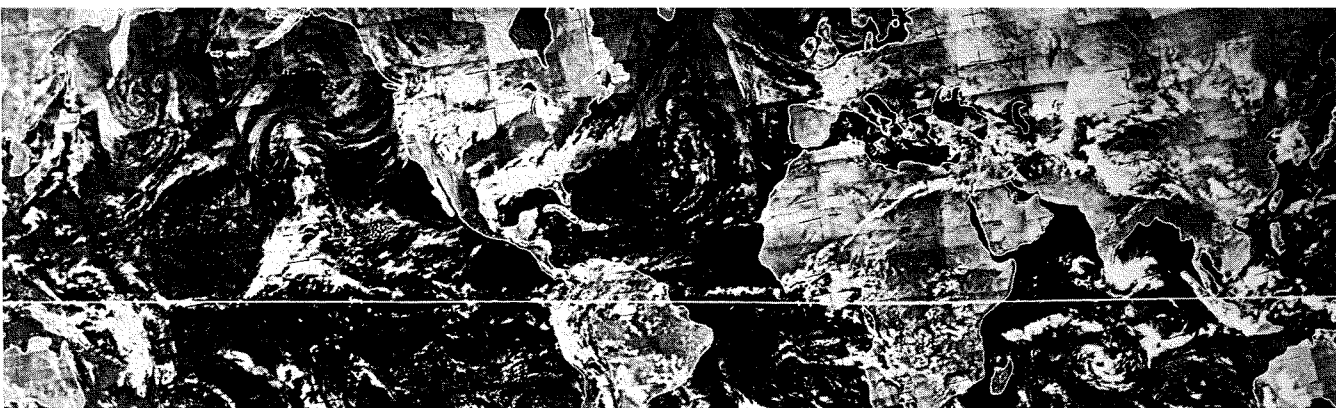
Fig. 2—First Complete view of the World's weather. This photomosaic is composed of 450 photographs taken by TIROS IX during its 12 orbits on February 13, 1965. (Courtesy of U.S. Environmental Science Services Administration.)
