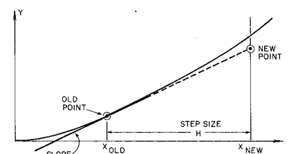
Fig. 4—Illustration of the basic principles in the numerical solution of differential equations.
