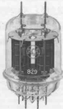
New P-P Beam Power RCA-829 takes 120 watts at the handy plate voltage of 500 volts. Goes all the way to 1 1/2 meters. Only 4 1/8" high and 2 1/4" in diameter.
