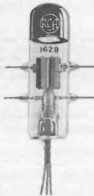
The new RCA-1628 transmitting triode takes maximum ratings as high as 500 Mc and reduced ratings up to 675 Mc.
