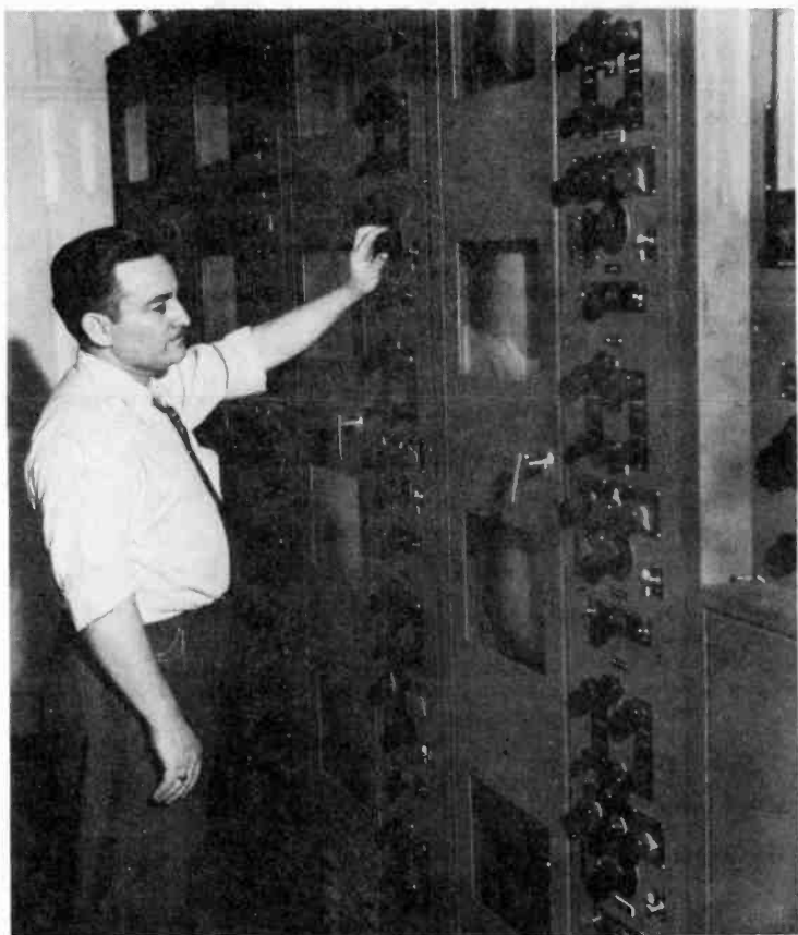
Final life tests are made on a sampling basis. 10BP4 kinescopes are operated day and night in these elaborate life test racks under simulated operating conditions more severe than might be encountered in the field.
