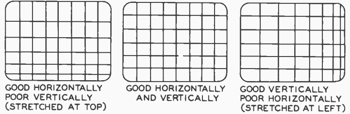
FIGURE 4. Horizontal and Vertical Lines instead of circles for Linearity Check.
