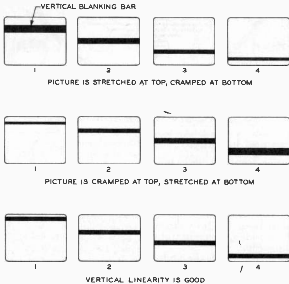
FIGURE 3. Checking Vertical Linearity with Vertical Blocking Bar.
