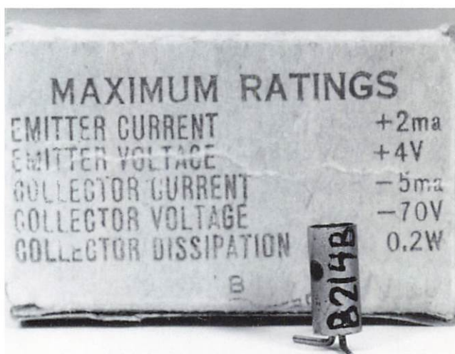
The transistor and maximum operating data.
