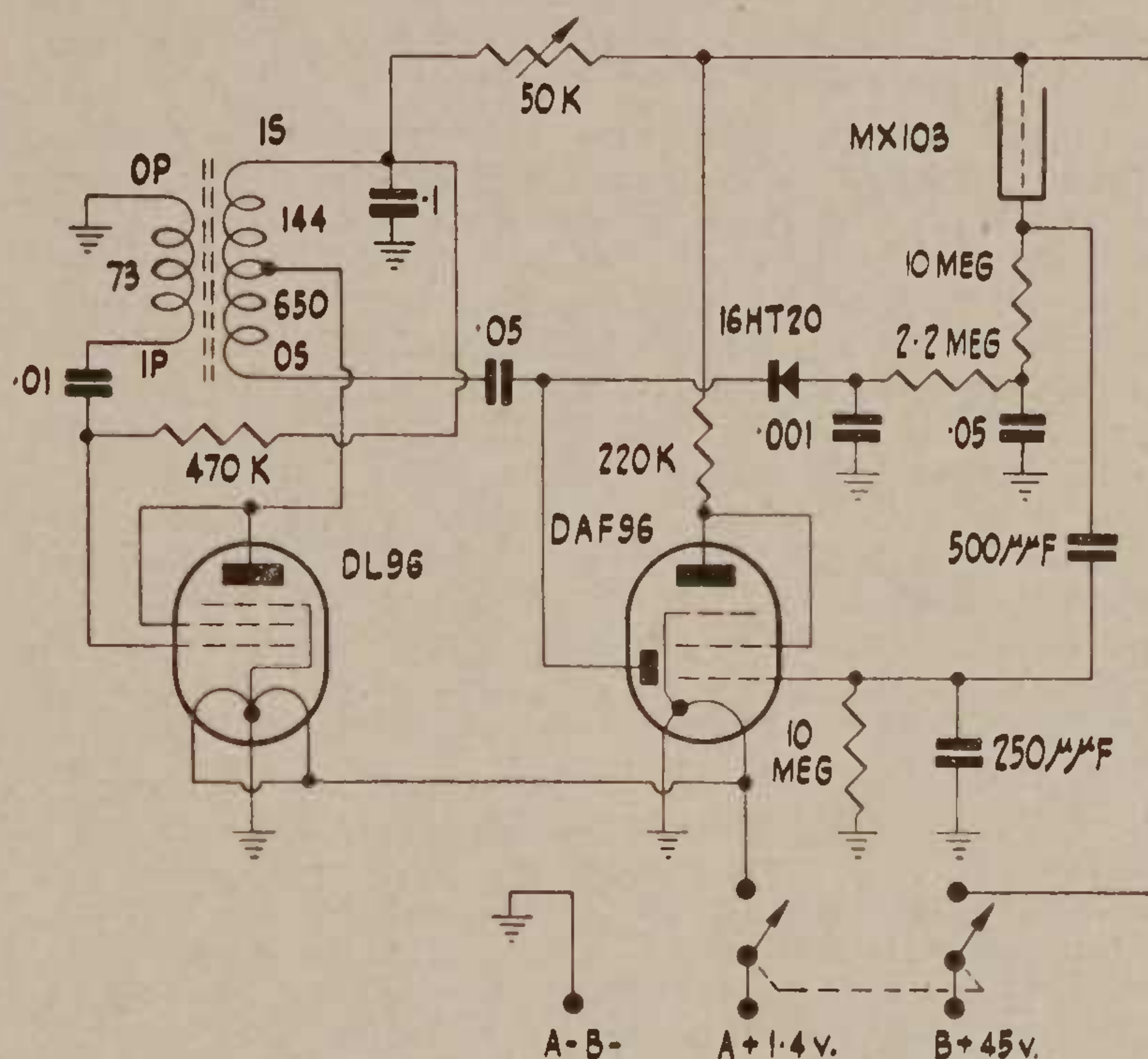
Circuit of the complete instrument. The transformer windings, which are made with 40-gauge enamelled wire, are described in the text. The core is a Ferro-cube one, type D25/17.5/11.5//11 n .
