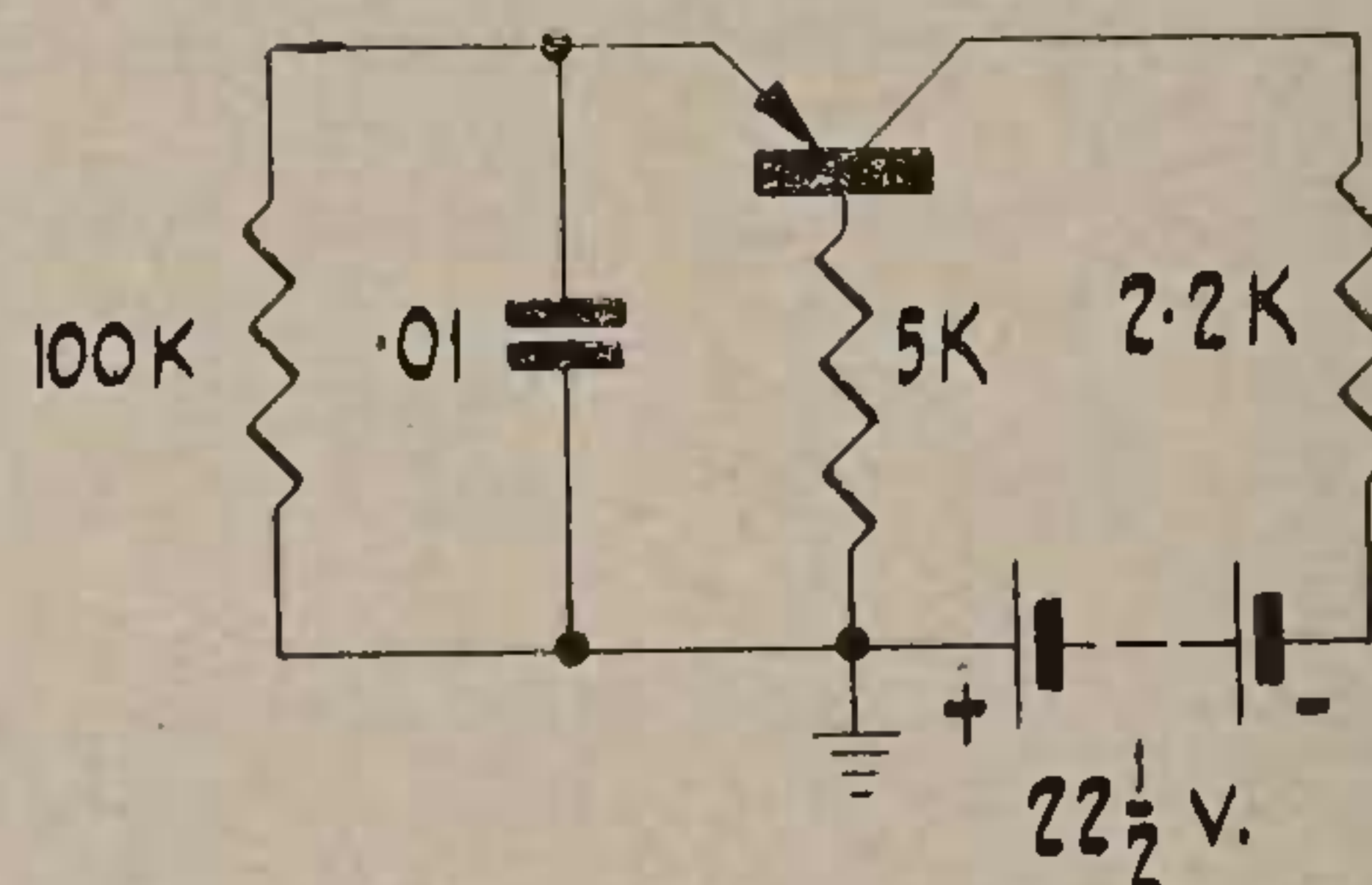
Fig. 3.—Circuit of a relaxation oscillator using a Philips OC51. This shows the standard symbol for a transistor. The heavy line is the base, the contact with the arrow head is the emitter, and the other is the collector. In this circuit, output can be taken either from the base or the collector, via a blocking condenser.
