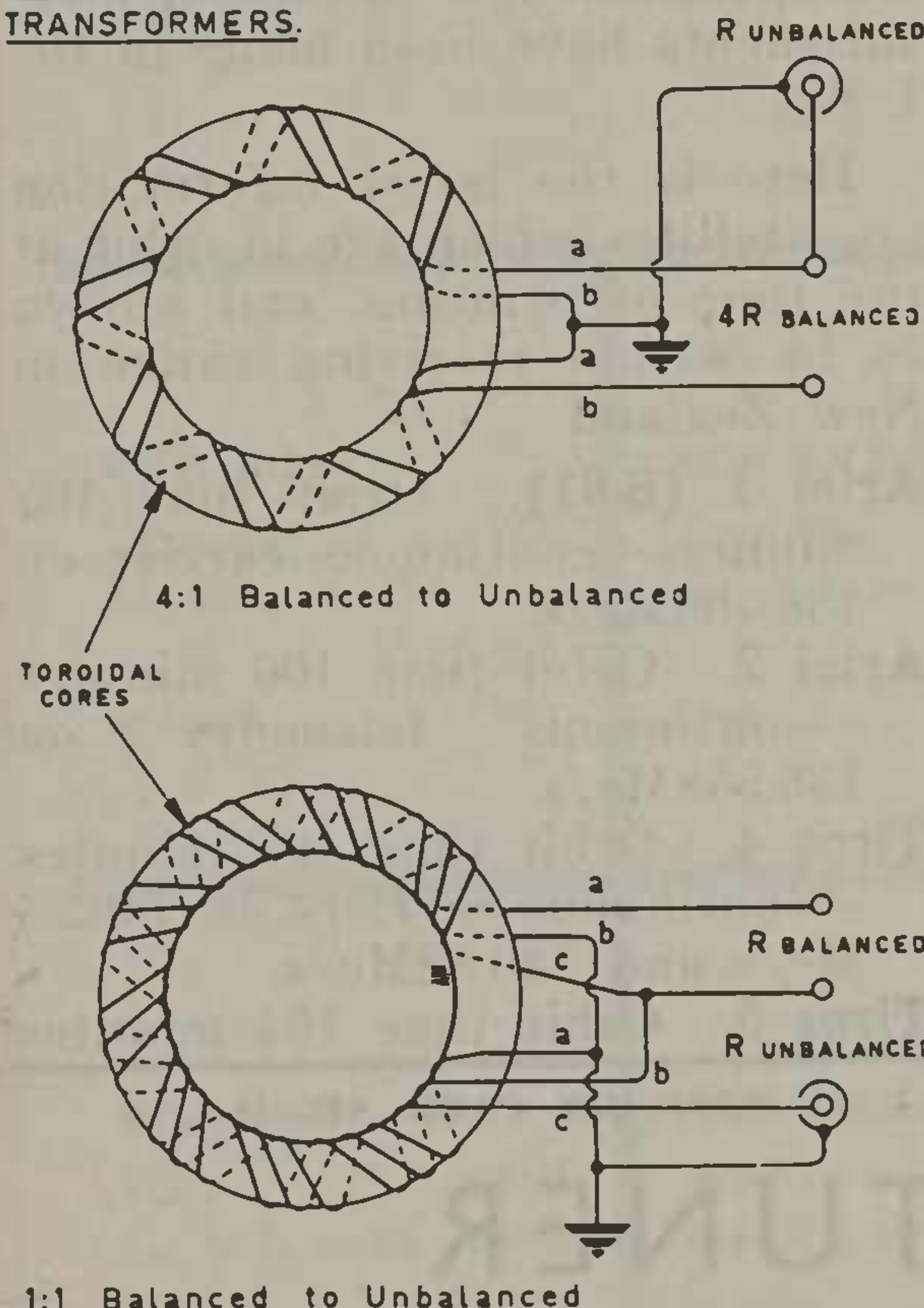
BROAD BAND TOROIDAL BALANCING TRANSFORMERS.
