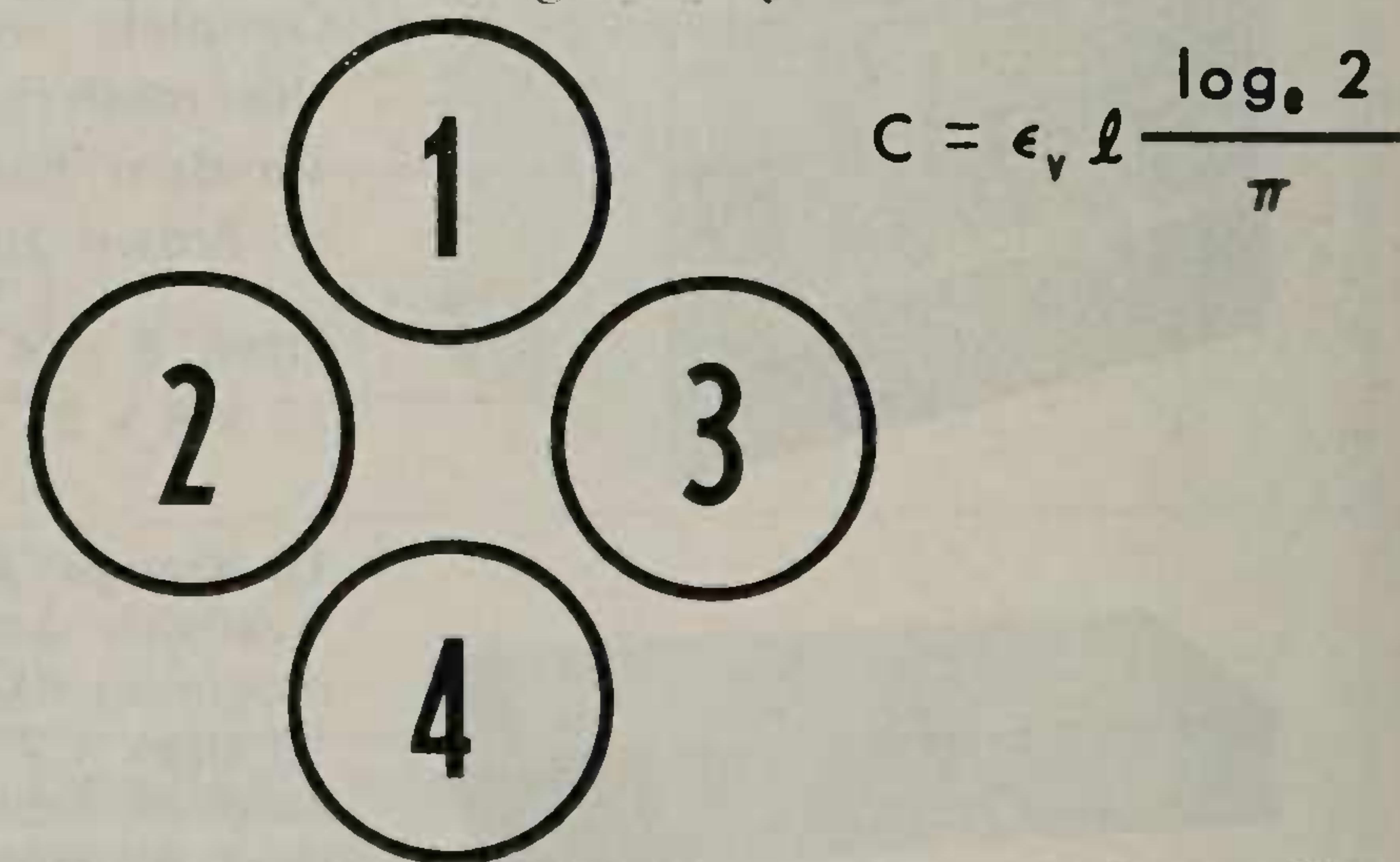
FIGURE 6. THOMPSON-LAMPARD COMPUTABLE CAPACITOR
