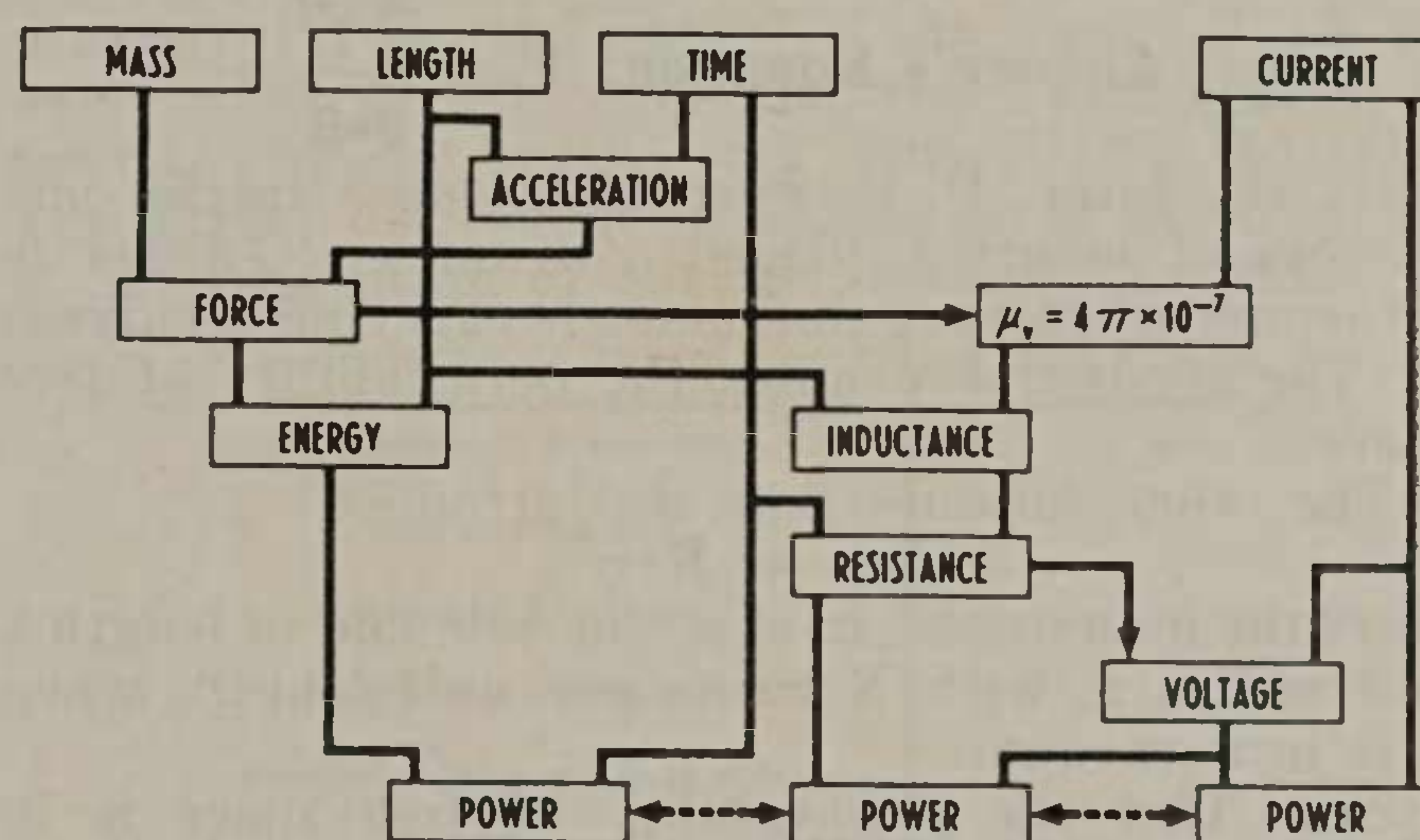
FIGURE 1. A DERIVATION OF POWER
