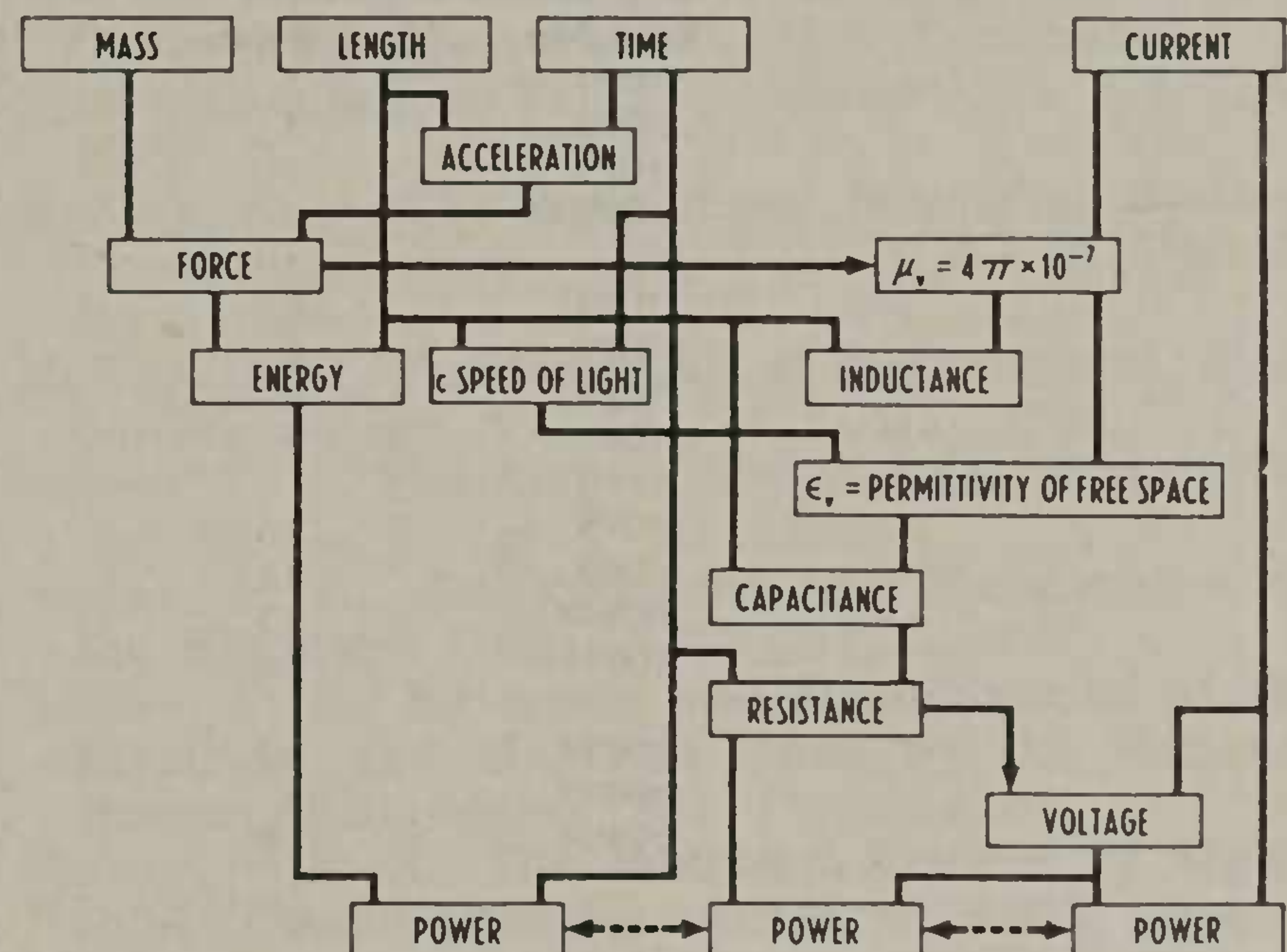
FIGURE 9. A DERIVATION OF UNITS USING CAPACITANCE
