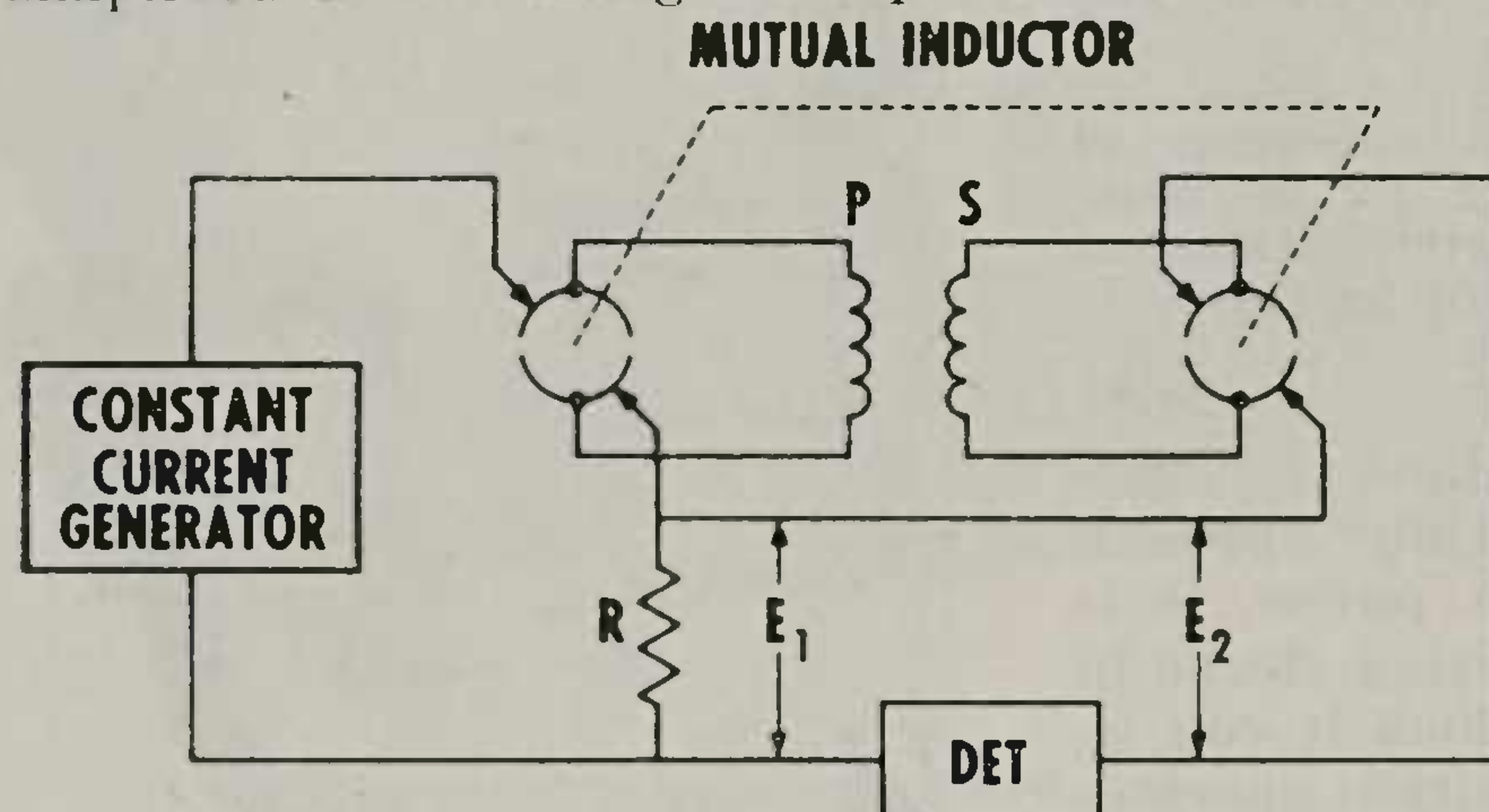
FIGURE 4. SIMPLIFIED SCHEMATIC OF WENNER METHOD OF DETERMINING RESISTANCE
