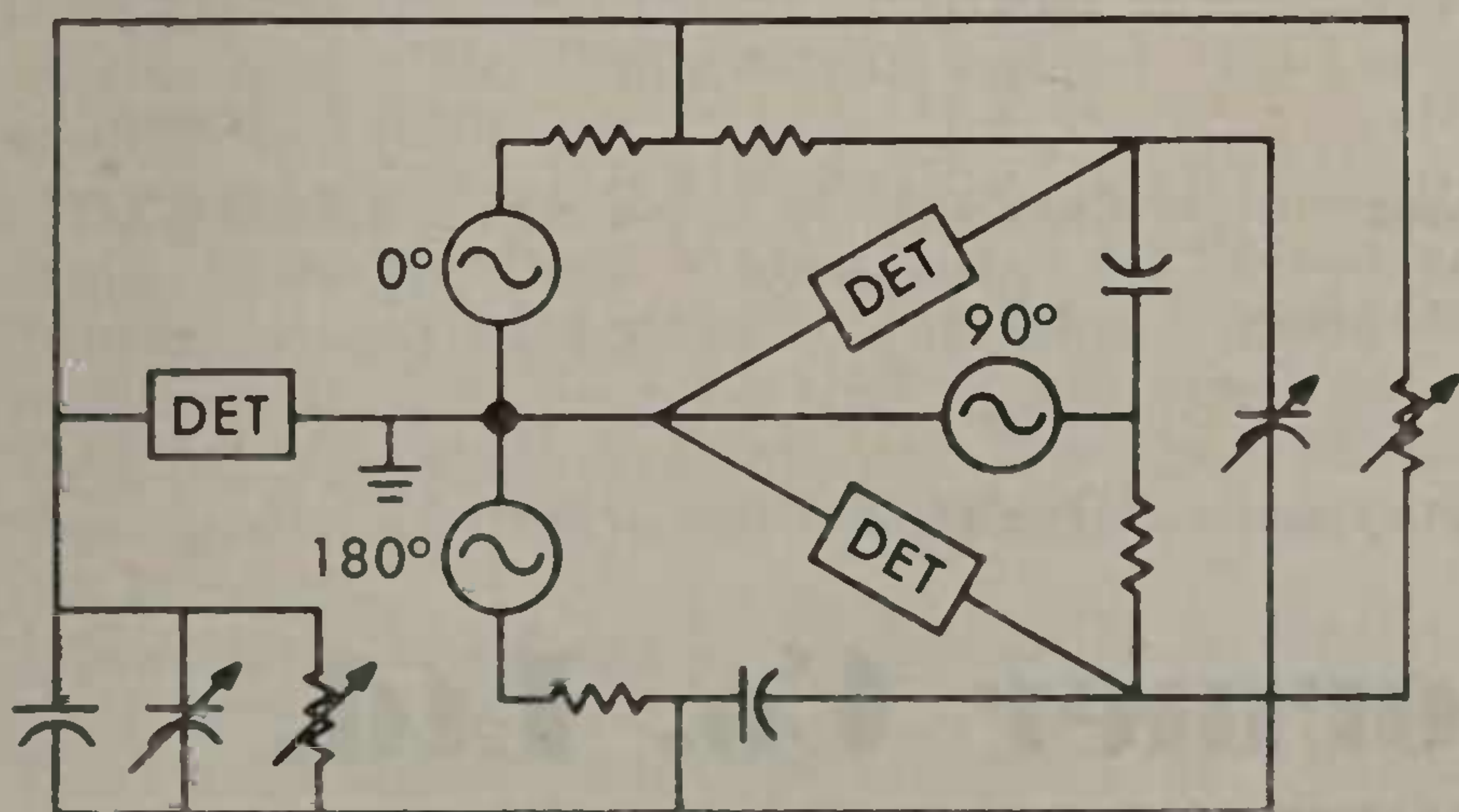
FIGURE 8. FREQUENCY-DEPENDENT BRIDGE SCHEMATIC
