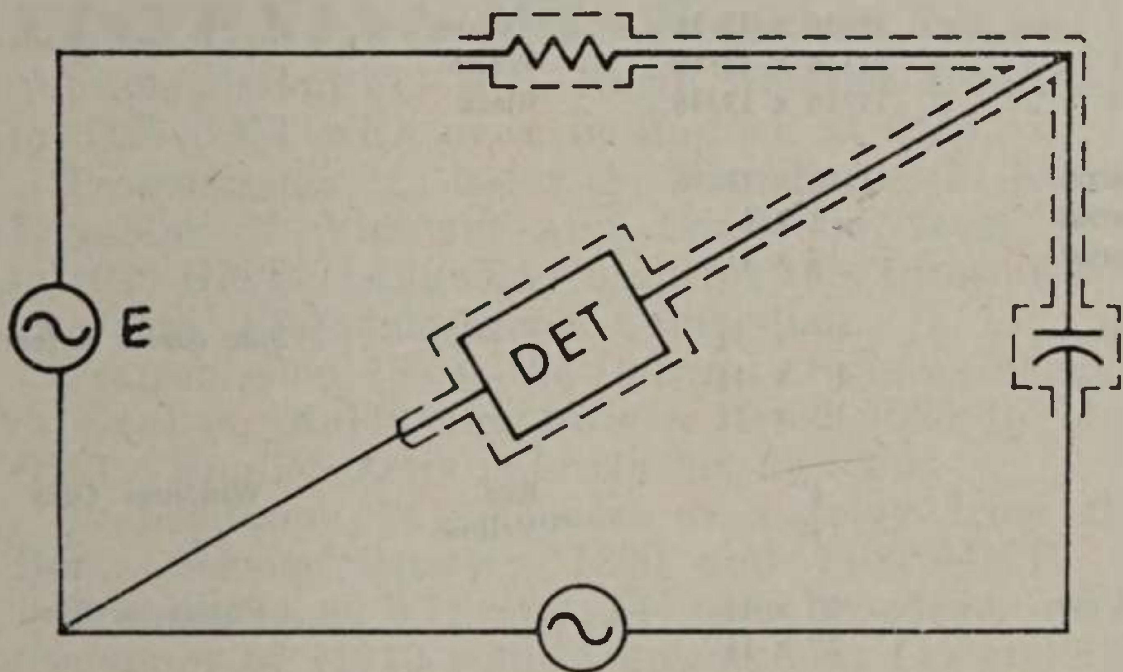
FIGURE 7. CAPACITIVE REACTANCE BRIDGE SCHEMATIC
