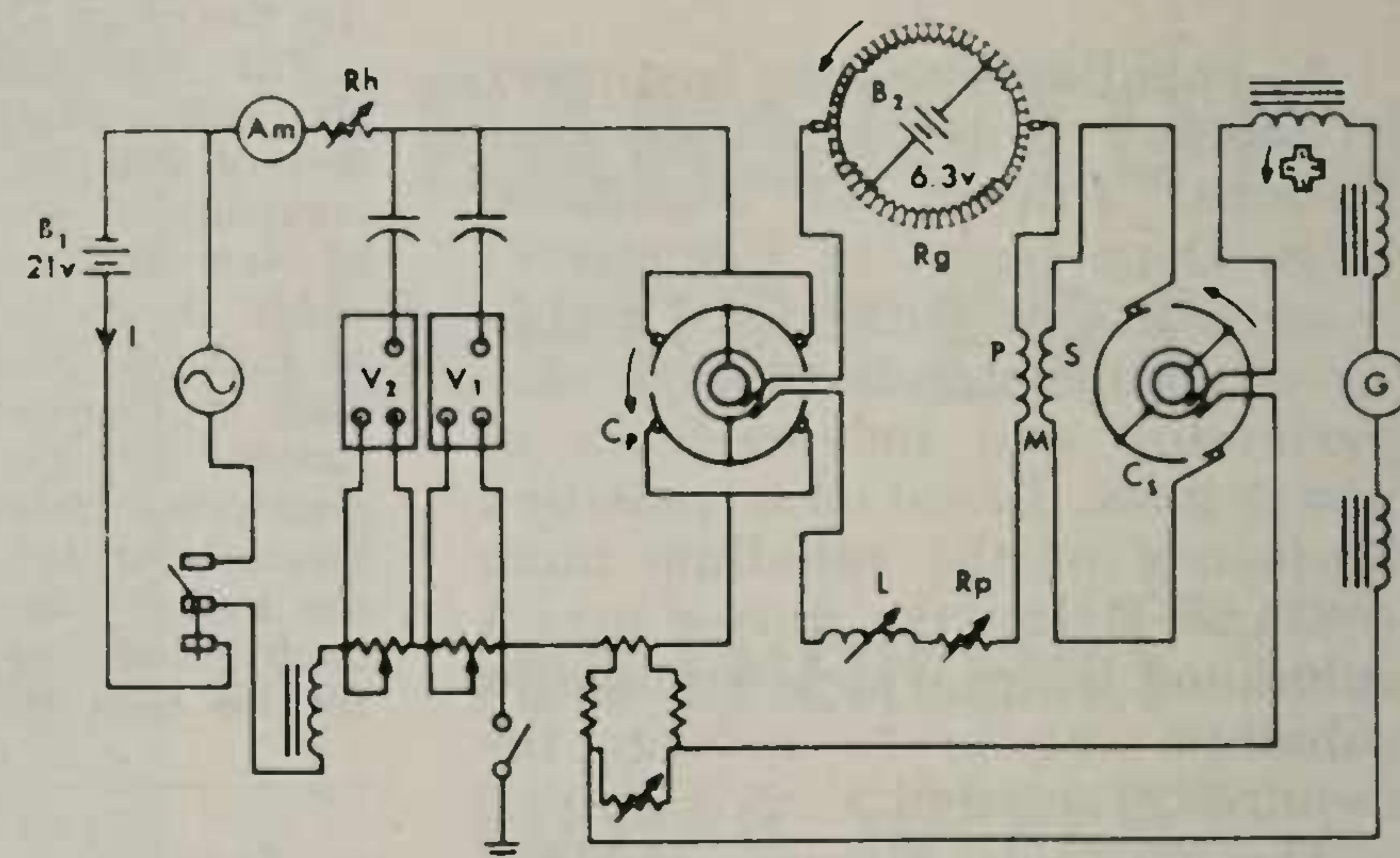
FIGURE 5. COMPLETE SCHEMATIC OF WENNER METHOD
