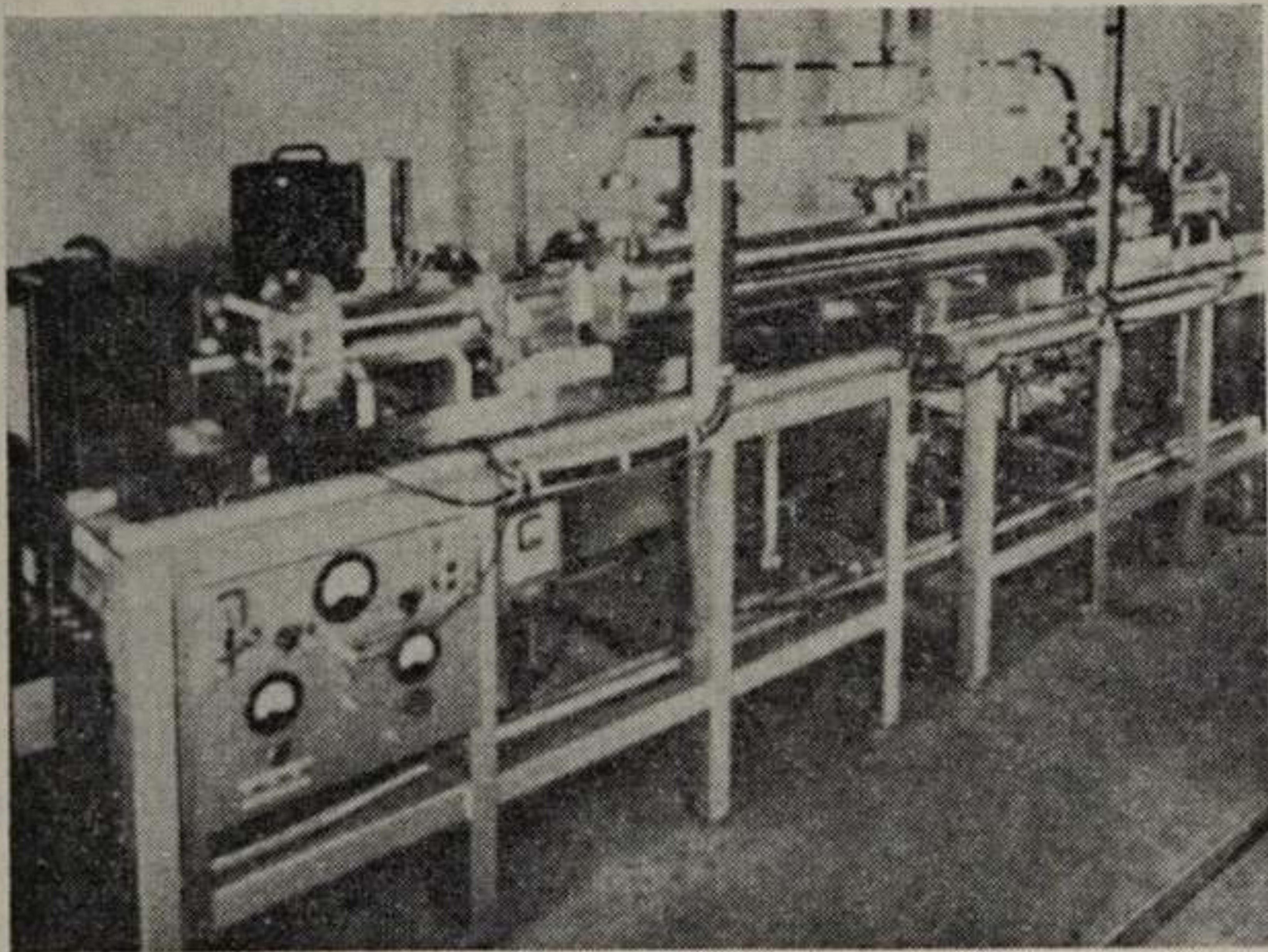
FIGURE 2. CESIUM BEAM FREQUENCY STANDARD (Photograph courtesy NBS)
