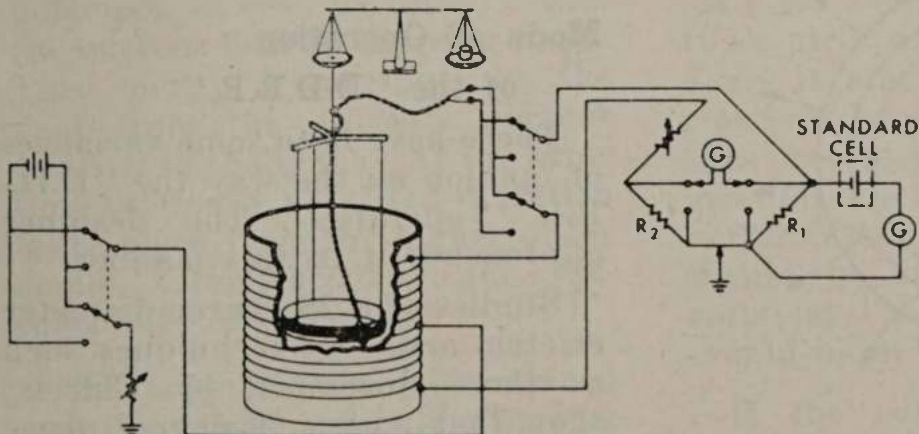
FIGURE 3. SCHEMATIC OF THE NBS CURRENT BALANCE
