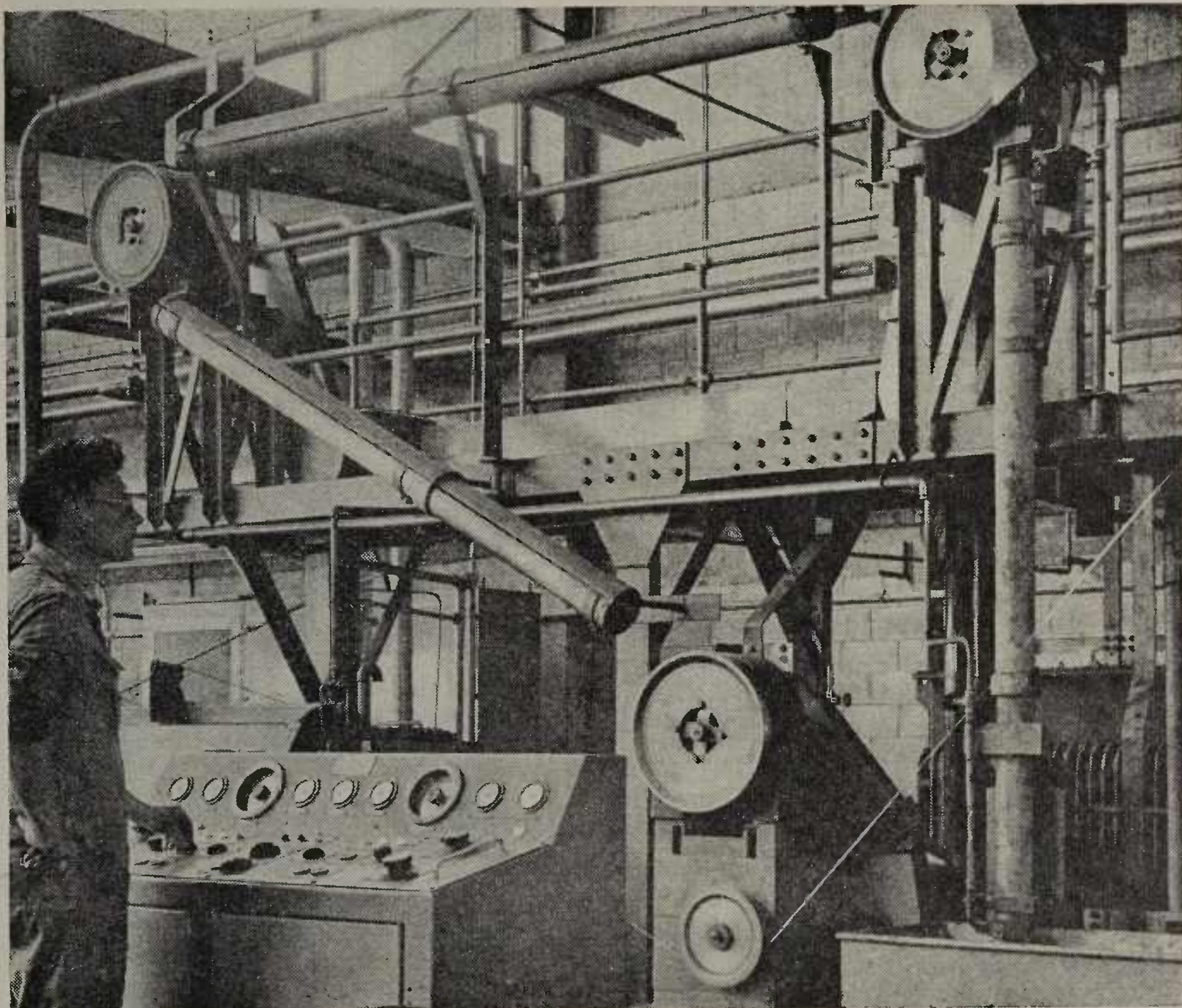
Initial wire-drawing process, where \frac{1}{4} -in. or \frac{5}{16} ths-in.-diameter copper rod is drawn down to 'feed wire'
