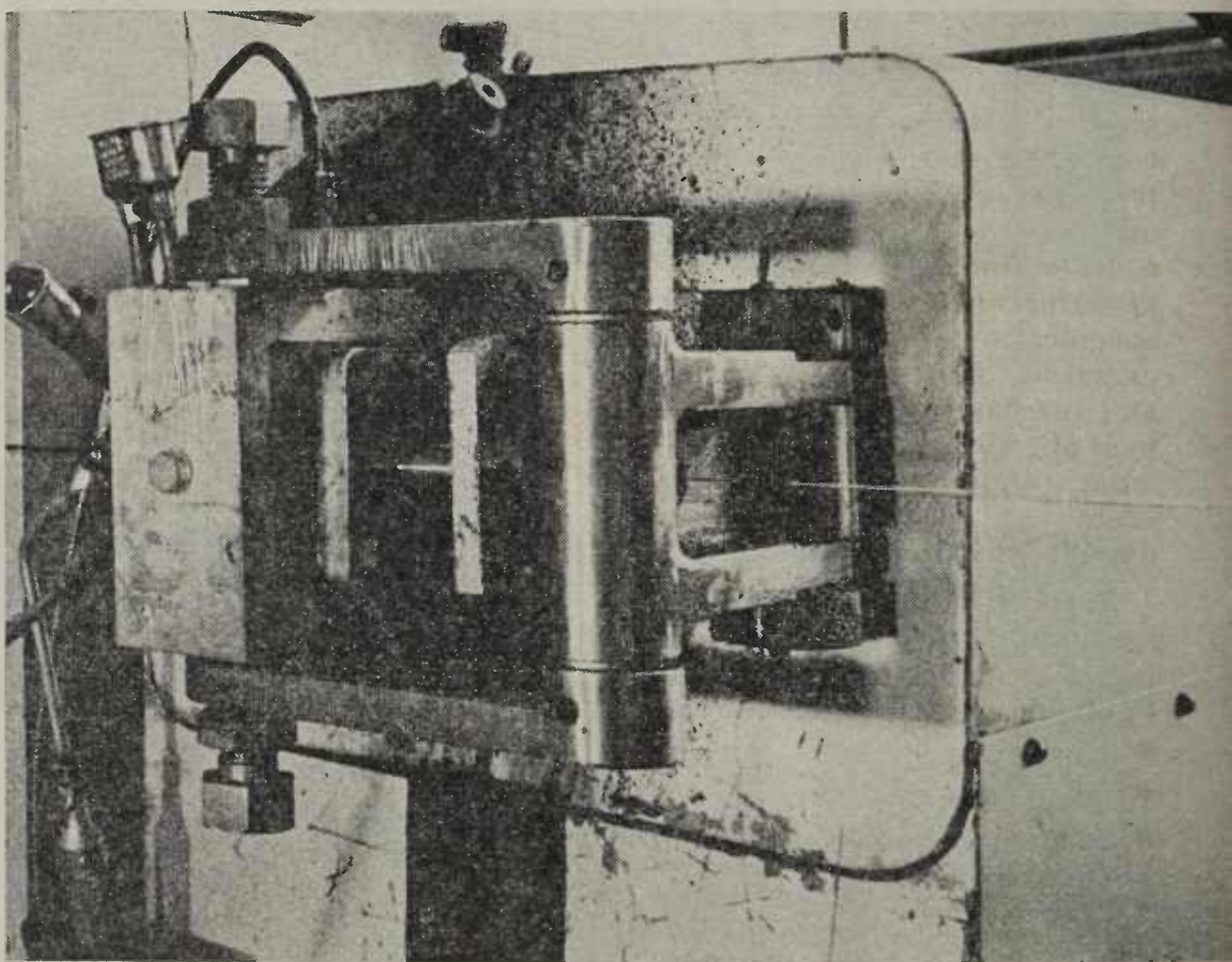
An insulating-type plastic extruder, showing the crosshead. Note the entry of the bare conductor at right of cross-head and its emergence as a plastic insulated conductor at the left
