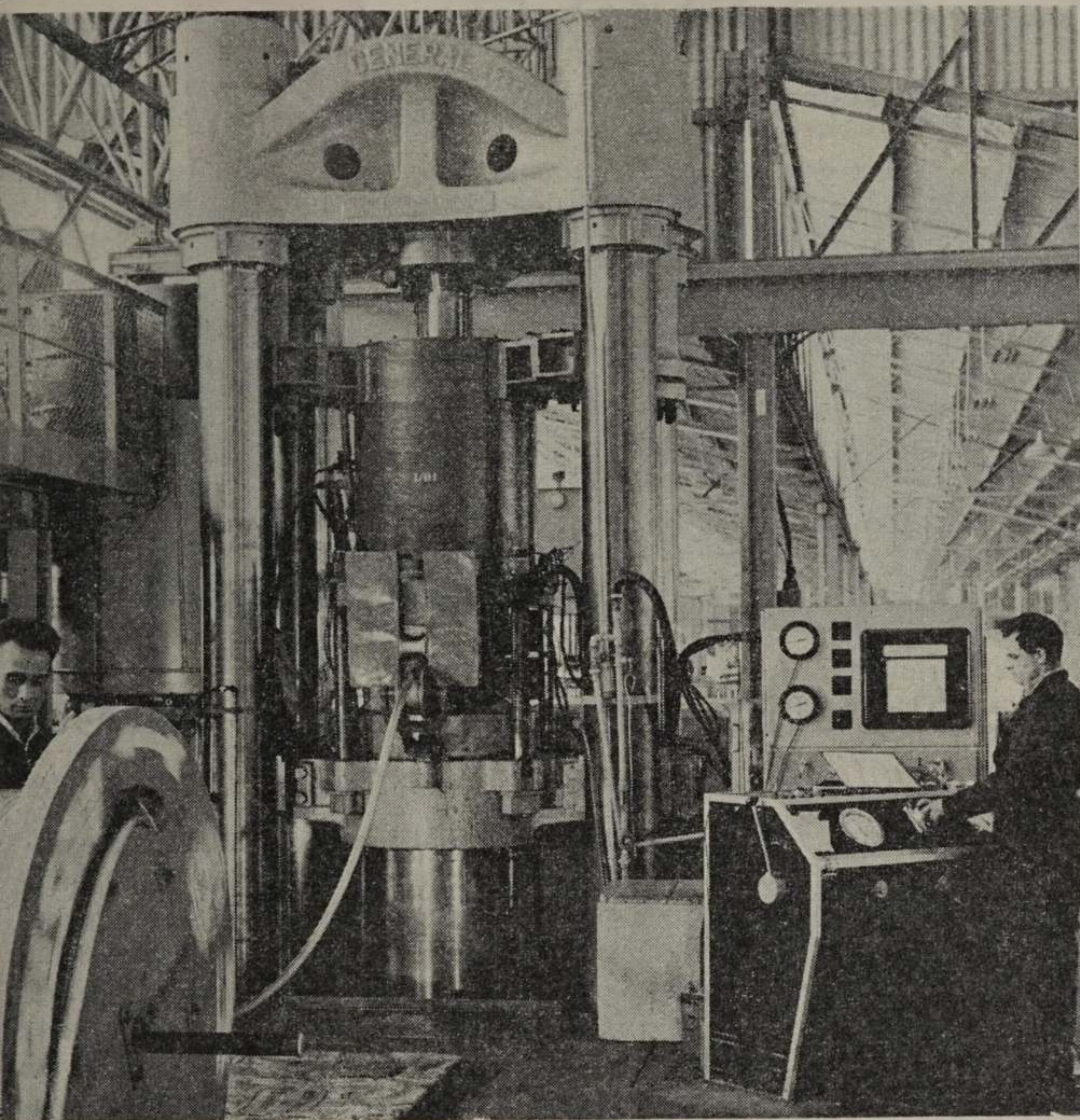
Left: A paper insulated cable being sheathed with lead through one of the large presses.
