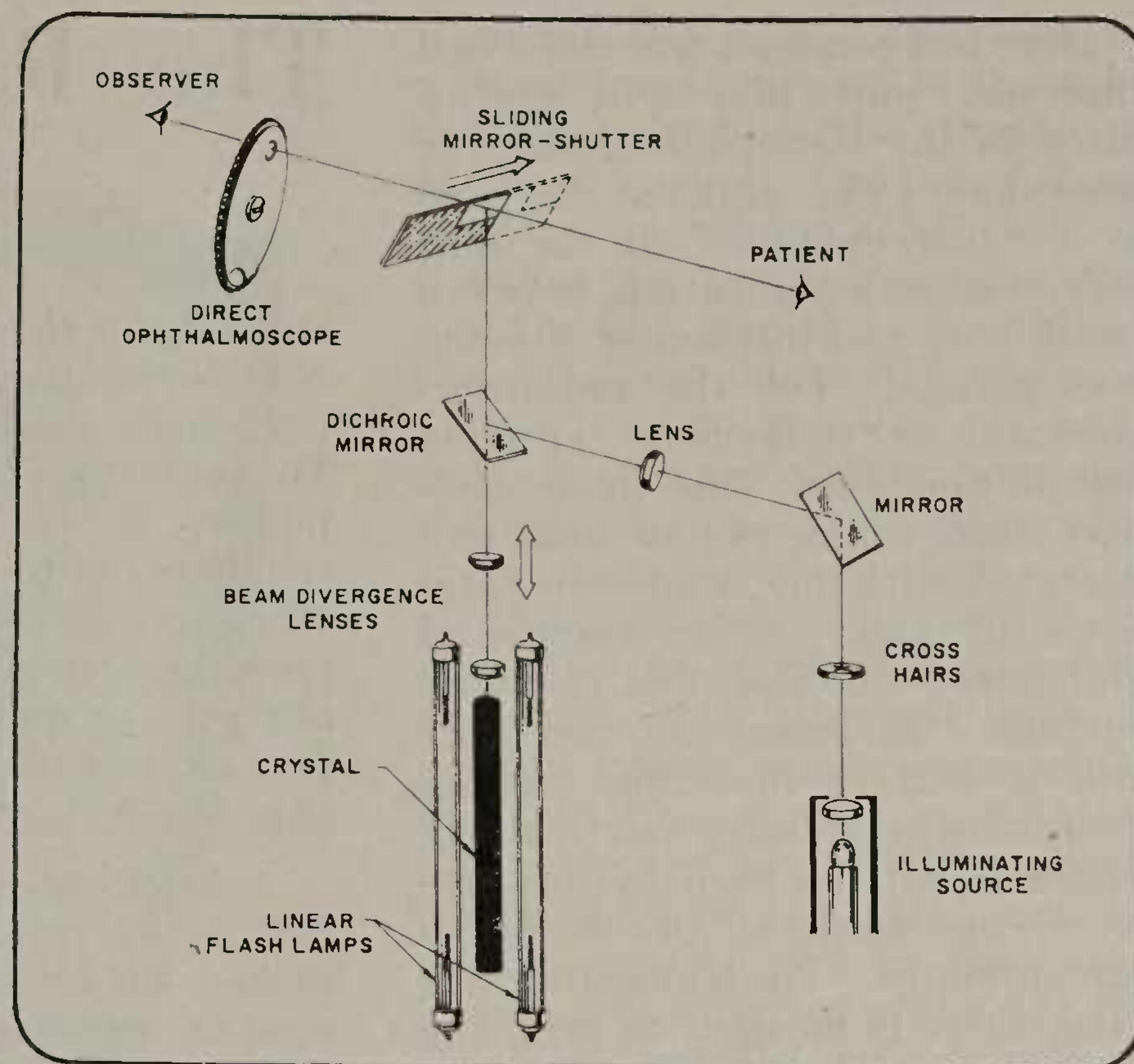
Fig. 2. Optical Layout
