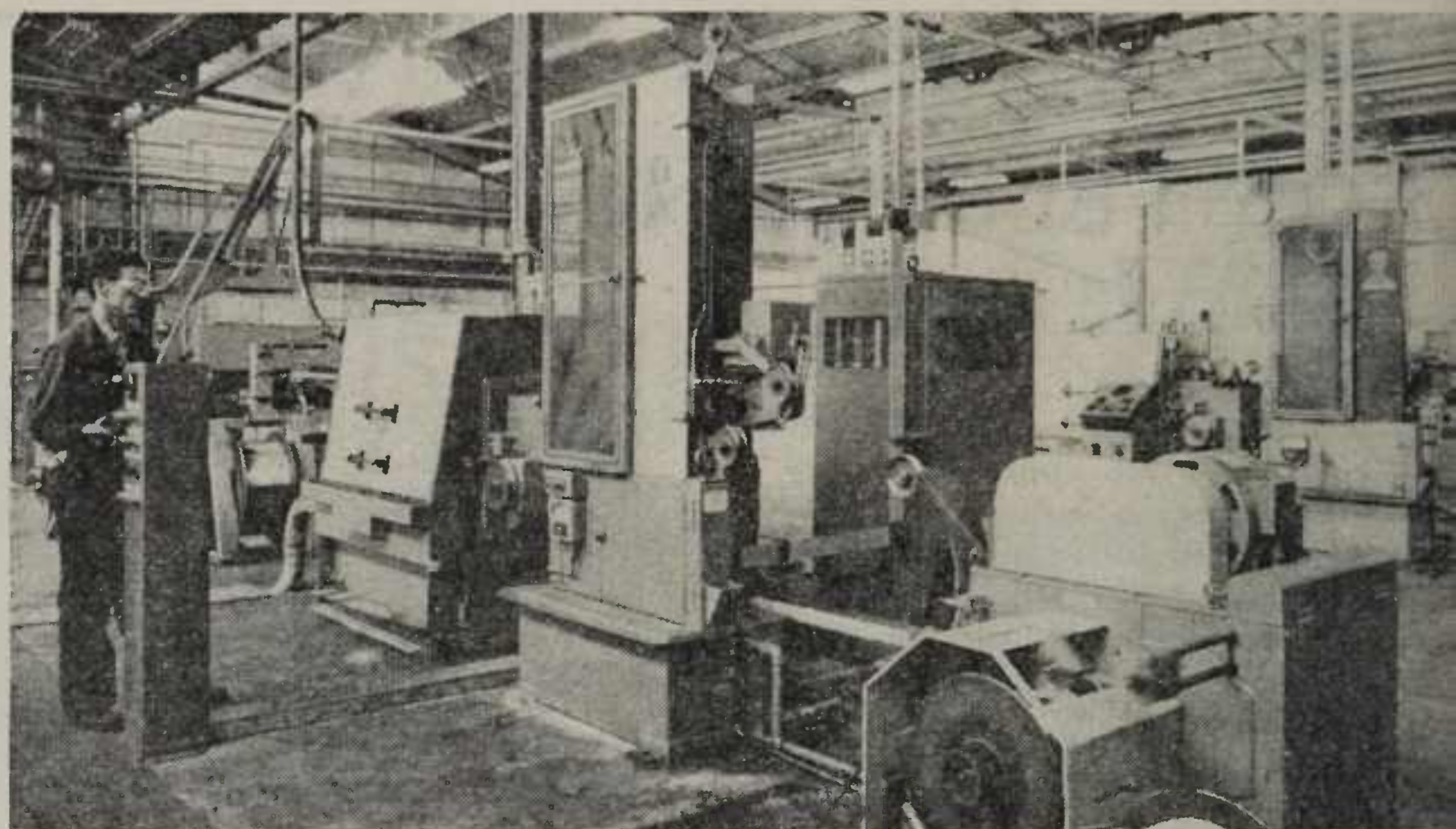
Second stage of wire drawing, where the 'feed wire' is drawn down to finished size and annealed
