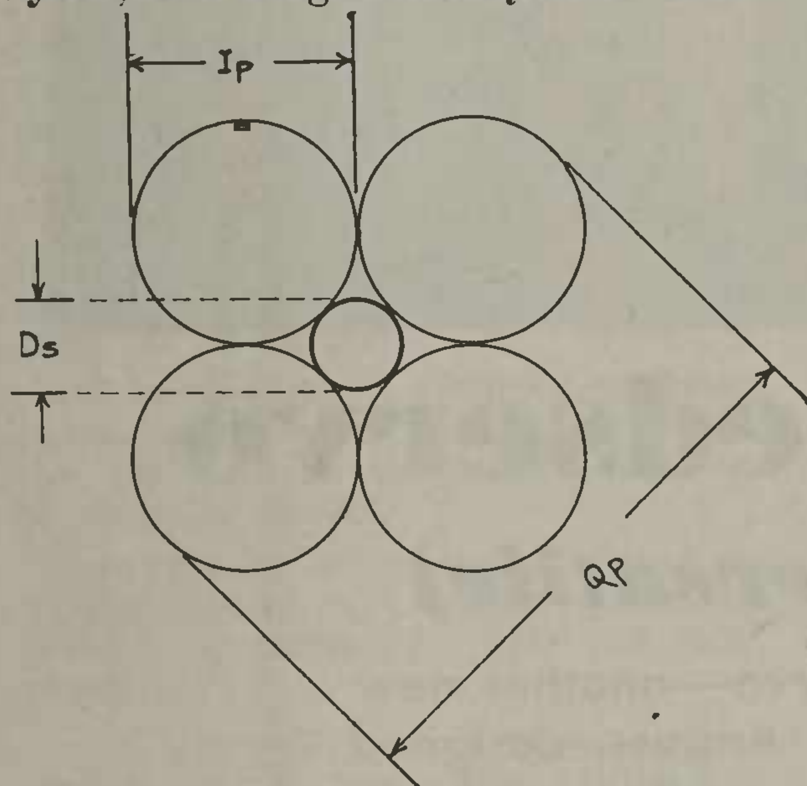
Quad formation showing four insulated conductors around a centre paper string.
