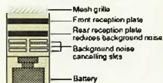
Back Electret (ECM2110) Side View
