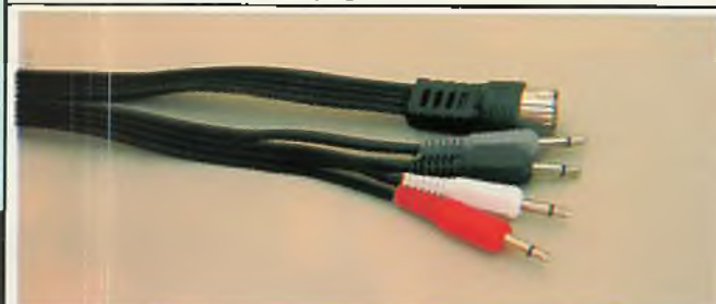
AL104 1.2 METRES $5.95 5 PIN DIN PLUG TO 4 X 3.5MM PLUGS Shielded cable with moulded plugs.
