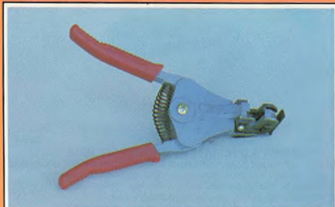
CS100 D.B. AUTOMATIC CABLE STRIPPERS Automatically grips, strips and ejects cable all in one movement. • Insulated handles with spring return • Suits Cable Diameter: 1 / 1.6 / 2 / 2.6 & 3.2mm • Length: 180mm (7") $29.95
