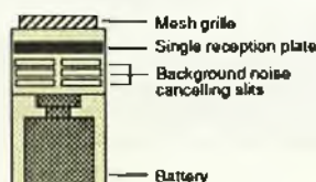
Normal Electret Side View
