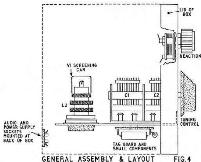
GENERAL ASSEMBLY & LAYOUT FIG. 4
