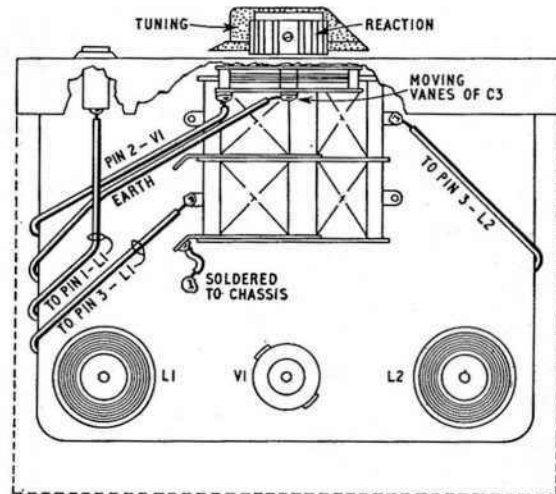
CHASSIS LAYOUT & WIRING ABOVE CHASSIS FIG. 2
