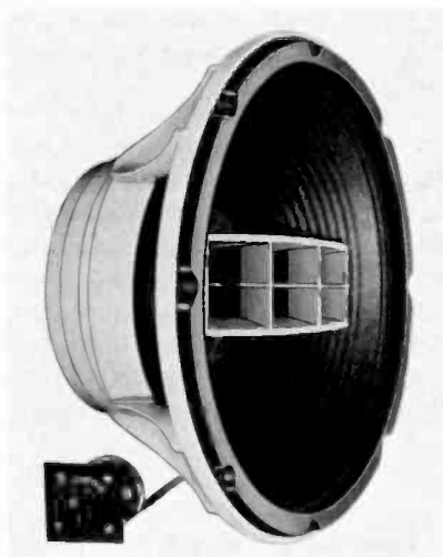
(B) 12" coaxial-type.
