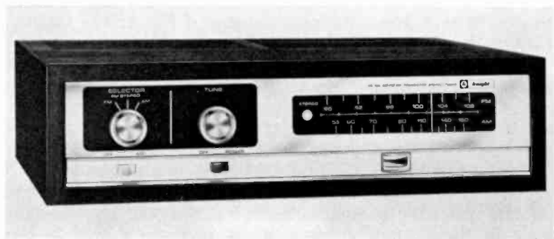
Fig. 2-3. Knight-Kit® stereo FM-AM tuner. Receives single-channel AM or FM, and multiplex (2 channel) FM broadcasts.
