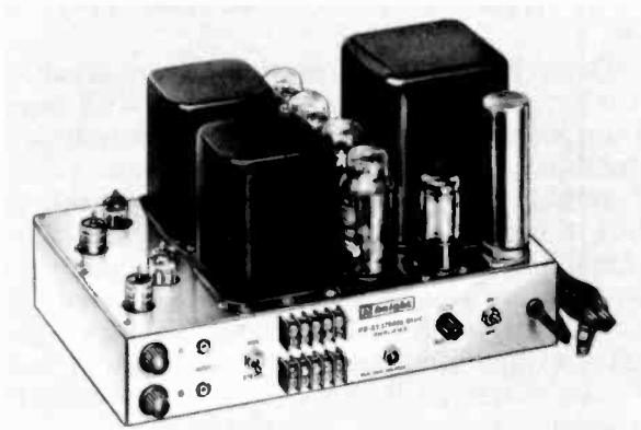
Fig. 3-2. Stereo basic amplifier used in systems with separate preamplifiers.
