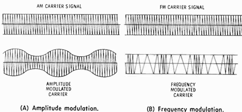
Fig. 2-2. Two methods of modulating an RF carrier signal.
