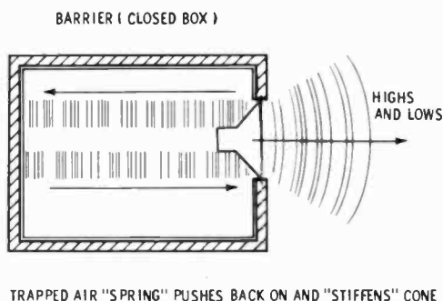
Fig. 3-13. A barrier-type speaker enclosure.
