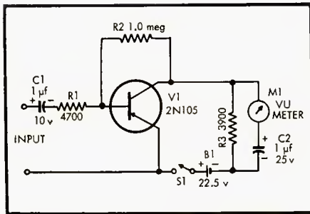
Fig. 2. The simple transistor amplifier which converts the VU meter from an insensitive instrument to one that responds full scale on five microamperes signal current.
