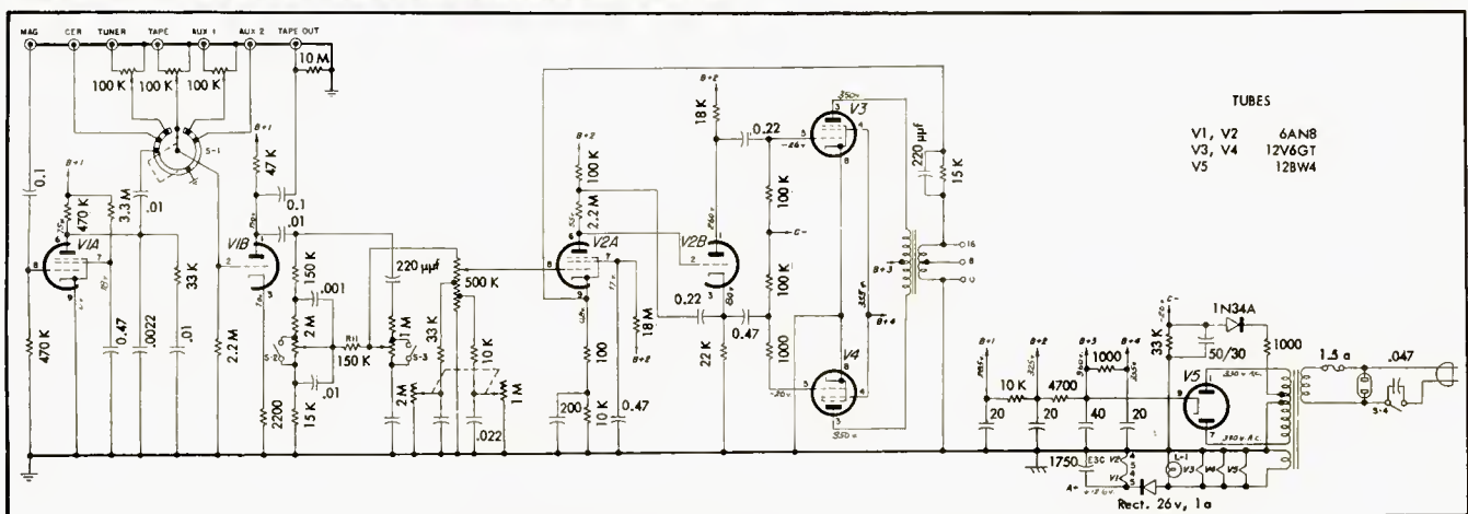
Fig. 3. Complete schematic of the Sonatone HFA-150.
