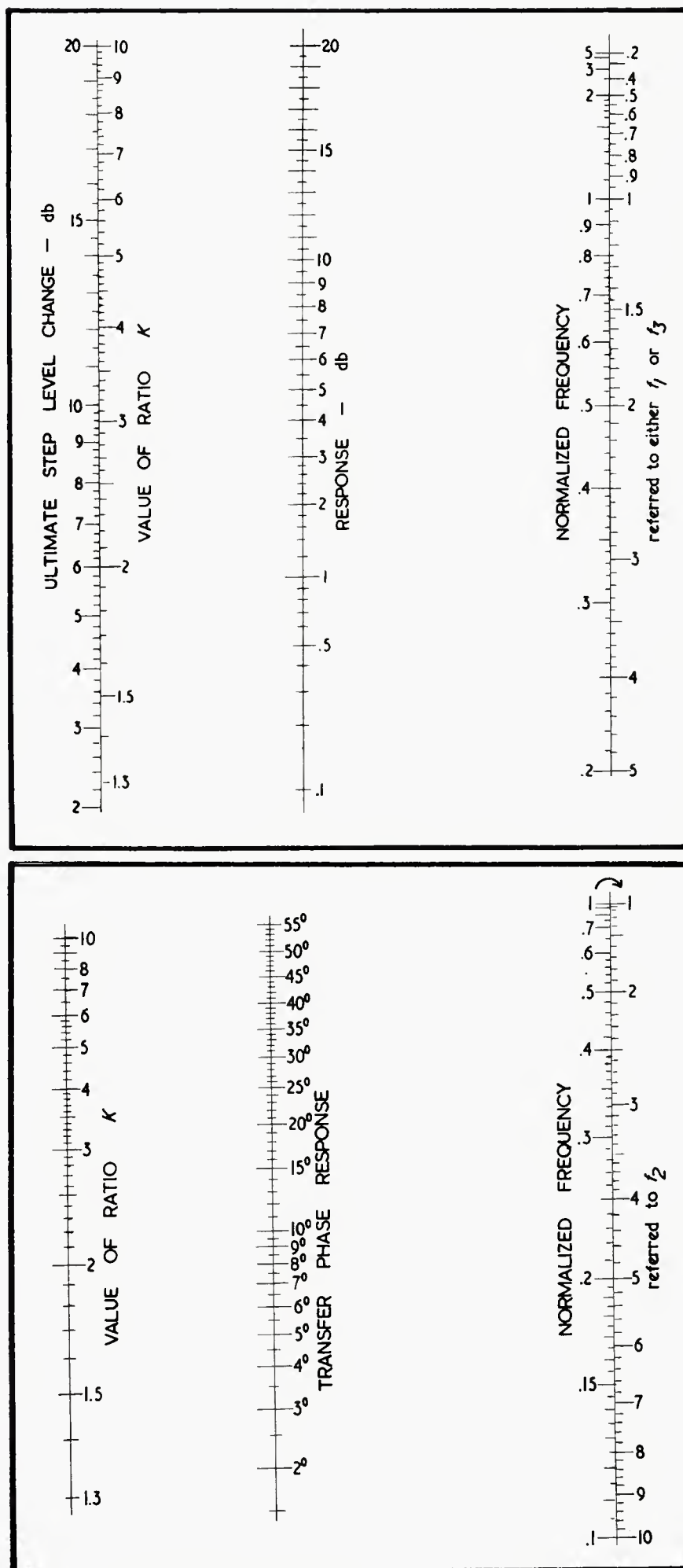
Fig. 3. Nomogram for quick computation of step response attenuation characteristic, normalized to either f_1 or f_3 .
