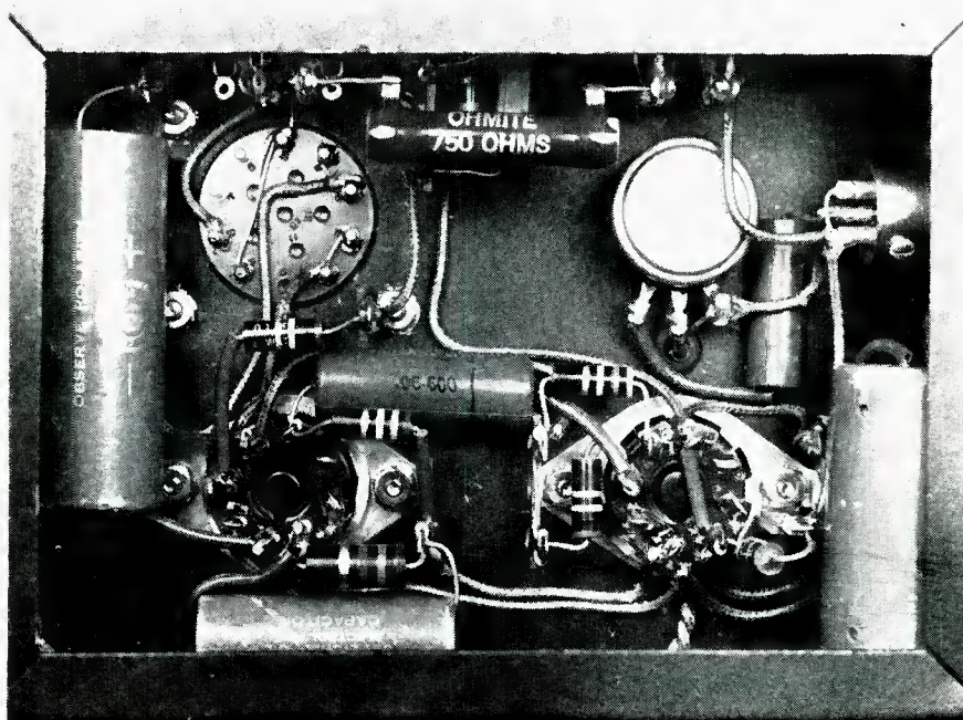
Fig. 4. Arrangement of components in the amplifier.
