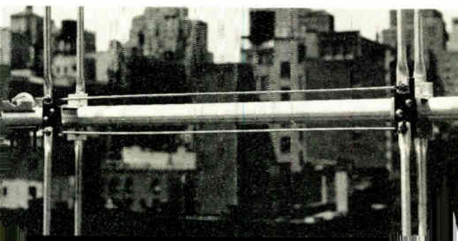
Closeup views showing details of the dipole mountings and connections of the Taco antenna, left, and the LaPointe antenna at the right
