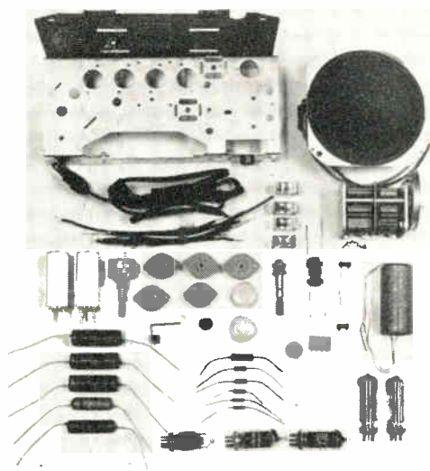
Here are all the components and hardware For an AC-DC table-model AM receiver
