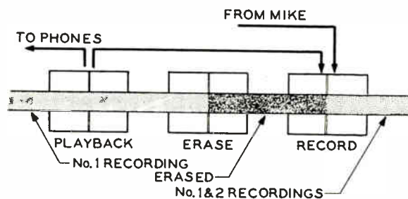
Fig. 1. Diagram showing the successive stages of S-O-S recording
