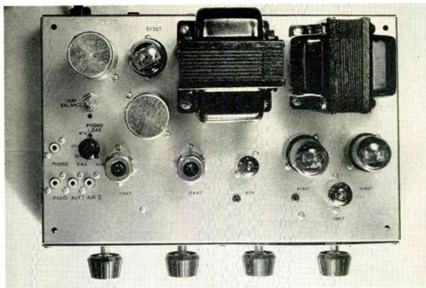
Fig. 2. Top view of the combination preamp and amplifier chassis. Dimensions are 12 ins. wide, 6\frac{3}{4} high, and 8\frac{3}{4} deep behind the front panel
