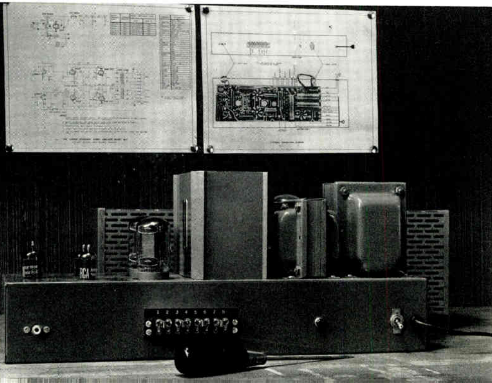
Fig. 1. The UTC Linear Standard amplifier kit was chosen as the first in this series of projects because it requires only the use of a screwdriver. Rated at 20 watts, it can be fed from any tuner, tape recorder, or crystal phonograph pickup, or from the preamplifier used with a magnetic pickup. A novice who has never tackled a job like this before can complete this amplifier, without hurrying, in less than one hour's time
