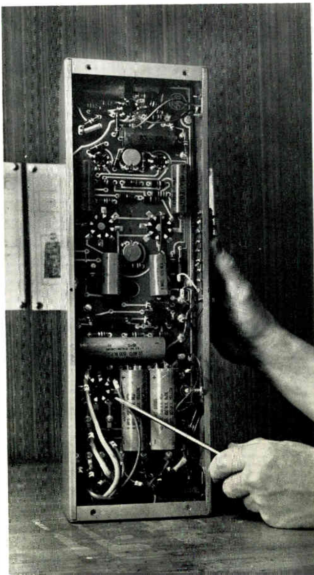
Fig. 3 above. Under side of the mounting plate. Fig. 5, below. In this view, all the wires have been connected to the terminals
