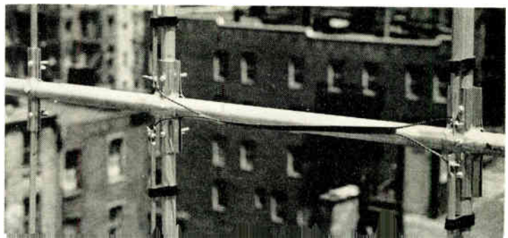
Closeup views showing details of the dipole mountings and connections of the Taco antenna, left, and the LaPointe antenna at the right
