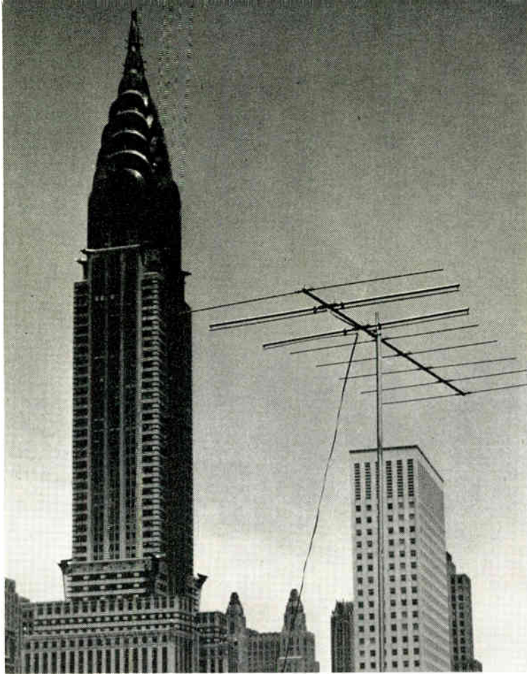
The La Pointe Yagi is delivered as shown at the right, requiring only a few minutes to open up and clamp the rods in place. It is shown at the left mounted on a simple mast of three 5-ft. telescoping steel tubes. Maximum pickup is towards background
