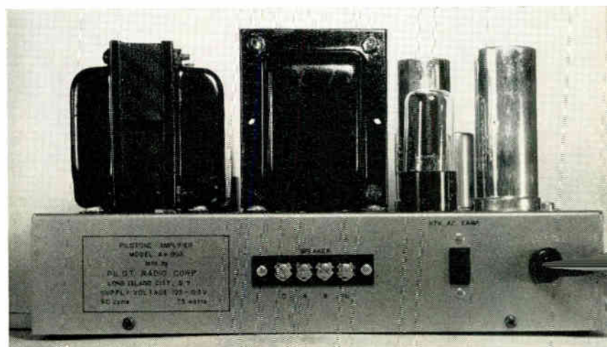
Fig. 3, above: Closeup of the input connections and the chassis adjustments. Fig. 4, below: Rear view showing speaker terminals and outlet
