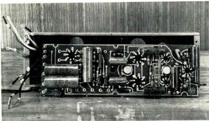
Fig. 3 above. Under side of the mounting plate. Fig. 5, below. In this view, all the wires have been connected to the terminals
