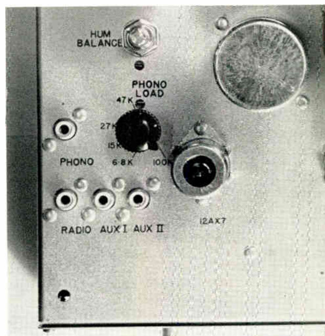
Fig. 3, above: Closeup of the input connections and the chassis adjustments. Fig. 4, below: Rear view showing speaker terminals and outlet
