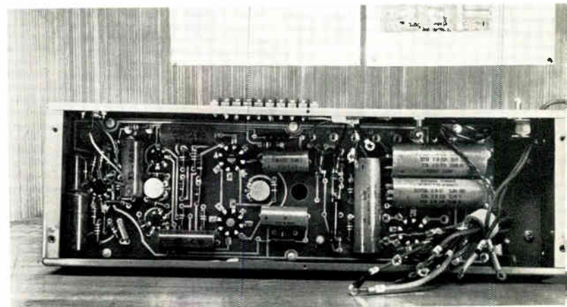
Fig. 4. Appearance of the chassis before the lugs on the numbered wires have been connected to the respective terminals
