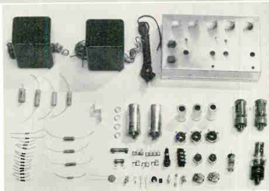
These two illustrations show all the components and parts for a Fisher FM-AM tuner and preamp above, and for a 25-watt power amplifier below. One tube is missing in the upper picture. Reproduced to the same scale as the picture on the opposite page, this explains graphically the difference in price between a conventional AC-DC radio and a hi-fi FM-AM tuner and preamp, with a high-quality power amplifier
