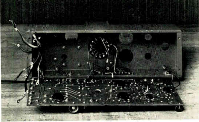
Fig. 2. Top of the mounting plate, with the tubes removed. Part of the printed-circuit wiring is carried on this side
