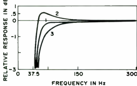
Fig. 5. Curve 1 is the target for Q_T = .38 ; Q_L = 10 ; curve 2 is for an h which is 10% too large; curve 3 is for an h which is 10% too small.
