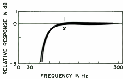
Fig. 3. 1 is the actual HD17B response and 2 is the target response.
