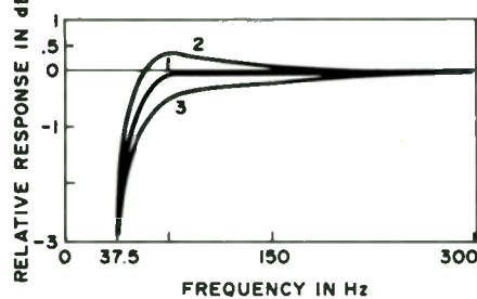
Fig. 4. Curve 1 is the target for Q_T = .38 , Q_L = 10 ; curve 2 is for a Q_T which is 5.25% too large; curve 3 is for a Q_T which is 5.25% too small.
