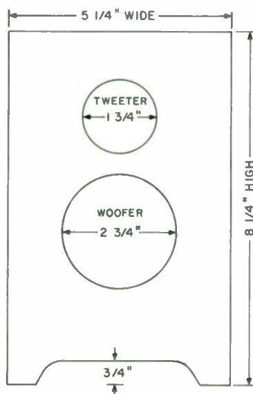
Fig. 3B. Front and bottom dimensions of the diffuser ported box. The trim on the grille is \frac{1}{8} " half round wood. The box is constructed of \frac{1}{2} " particle board. The diffuser blocks on the bottom are 1"x3" stock.
