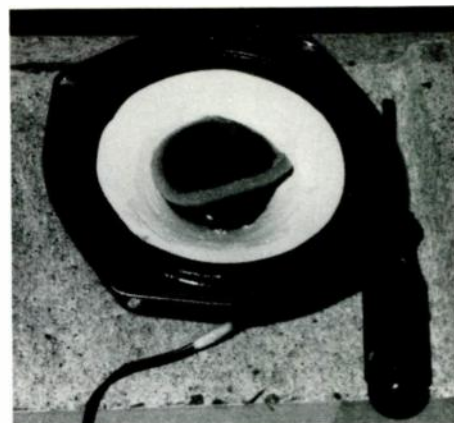
Photo 2. Preparing the speaker for use in the enclosure involves cones and whizzer alteration.
