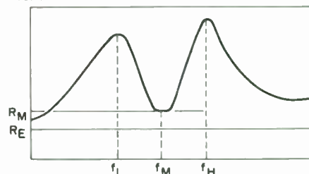
Fig. 1. Shape of impedance curve for a vented box system.
