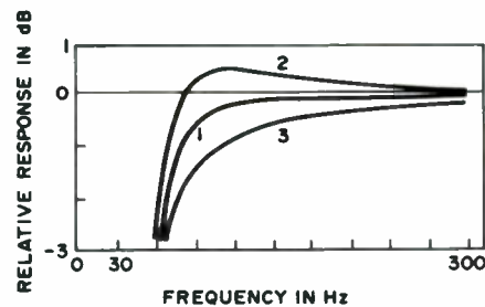
Fig. 9. Curve 1 is the target response for Q_L = 7 ; Q_T = .20 . Curve 2 results from a +10% error in Q_T and curve 3 results from a -10% in the same parameter.
