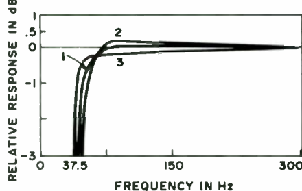
Fig. 6. Curve 1 is the target for Q_T = 10 ; Q_T = .38 ; curve 2 is for an \alpha which is 20% too large; curve 3 is for an \alpha which is 20% too small.
