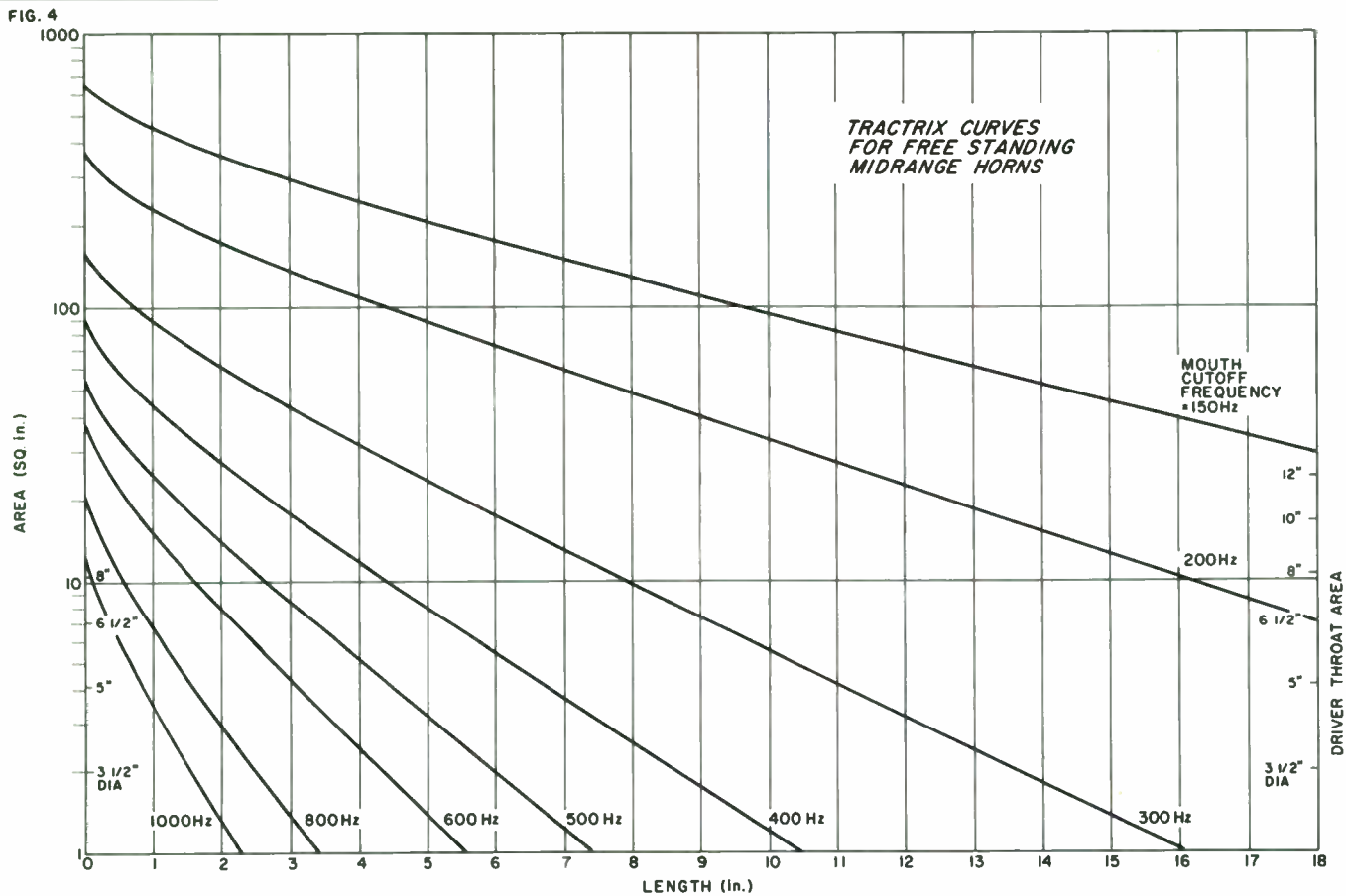
Fig. 4. Tractrix area expansion for midrange horns (free standing) with low frequency cutoffs from 150Hz to 1kHz.
