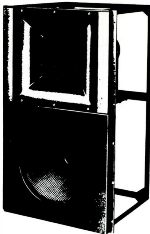
Fig. 7. Spherical-wave midrange horn with direct radiator woofer used in Germany in the early 1950's.
