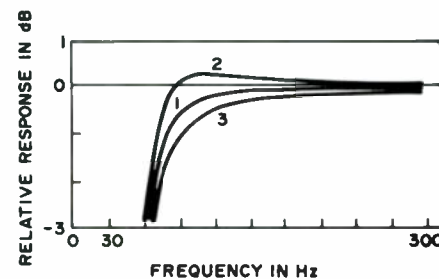
Fig. 10. Curve 1 is the target response for Q_L = 7 , Q_T = .20 . Curve 2 results from a +10% error in h and curve 3 from a -10% error in the same parameter.
