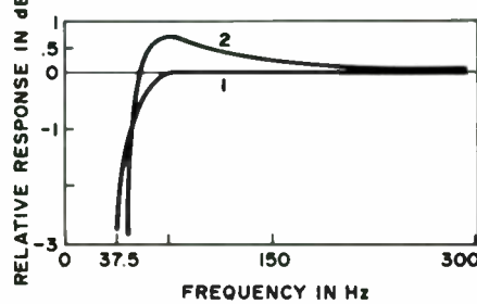
Fig. 7. Curve 1 is the target for Q_T = .38 , Q_L = 10 ; curve 2 is the response when h is 10% too large and \alpha is 20% too large.
