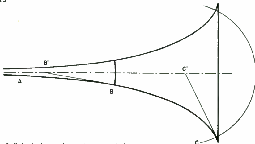
Fig. 3. Spherical wavefronts in a tractrix horn.
