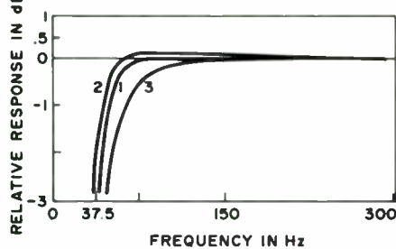
Fig. 8. Curve 1 is the on target response with Q_T = .38 , Q_L = 10 ; curve 2 is for Q_L = 15 ; curve 3 is for Q_L = 3 .
