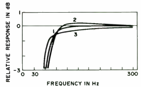
Fig. 11. Curve 1 is the target response for Q_L = 7 , Q_T = .20 . Curve 2 results from a +20% error in \alpha and curve 3 from a -20% error in the same parameter.
