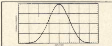
Figure 1. White noise voltage distribution.
