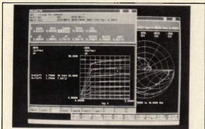
Figure 5. Xtract is used for large-signal and linear model extraction.
