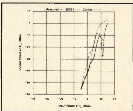
Figure 2(d). Comparison of data at fourth harmonic.
