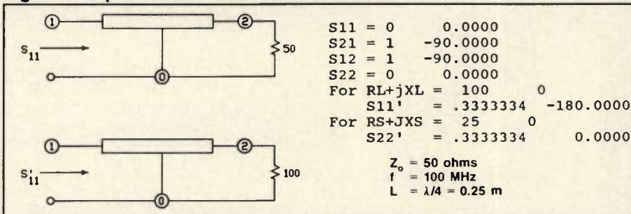
Figure 4. S-parameters for a transmission line.
