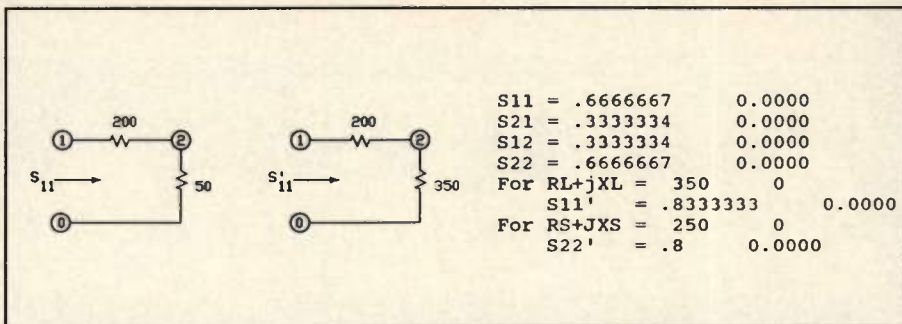
Figure 3. S-parameters for a series resistor.
