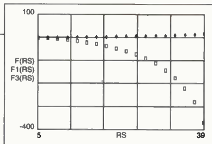
Figure 2. Sensitivities of R_S with respect to X_1 for pi (cross), mixed pi (square) and mixed tee (diamond) networks. R_L = 50 , Q = 5 .
