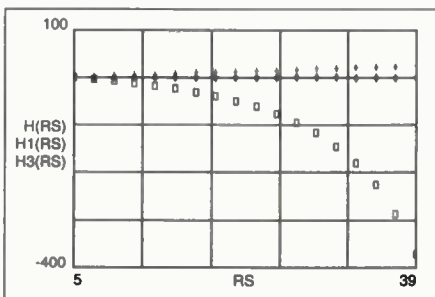
Figure 6. Sensitivities of R_S with respect to X_3 for pi (cross), mixed pi (square) and mixed tee (diamond) networks. R_L = 50 , Q = 5 .
