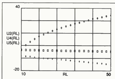
Figure 11. Sensitivities of R_L with respect to X_2 for standard tee (cross), series enhanced-Q L (square) and shunt enhanced-Q L (diamond) networks. R_S = 5 , Q = 5 .
