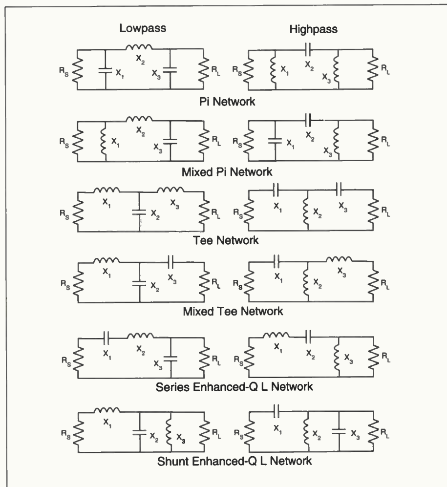
Figure 1. Narrowband matching network topologies.
