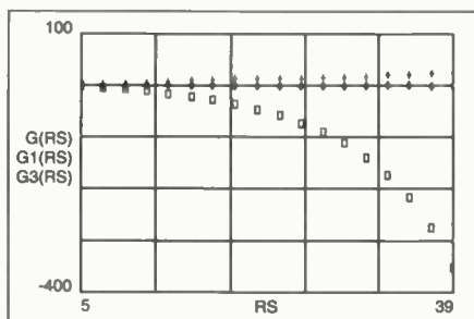
Figure 4. Sensitivities of R_S with respect to X_2 for pi (cross), mixed pi (square) and mixed tee (diamond) networks. R_L = 50 , Q = 5 .
