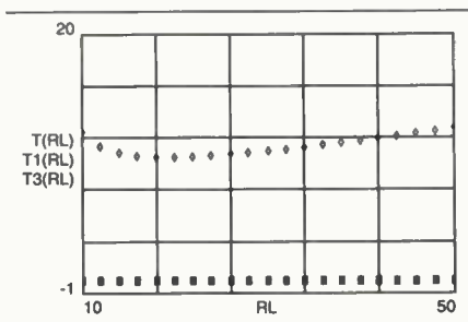
Figure 8. Sensitivities of R_L with respect to X_1 for pi (cross), mixed pi (square) and mixed tee (diamond) networks. R_S = 5 , Q = 5 .
