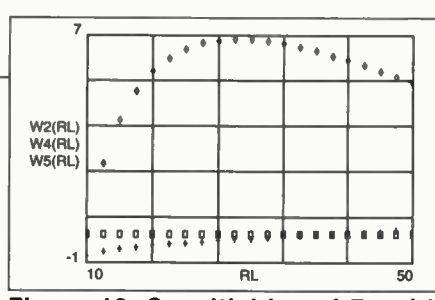
Figure 13. Sensitivities of R_L with respect to X_3 for standard tee (cross), series enhanced-Q L (square) and shunt enhanced-Q L (diamond) networks. R_S = 5 , Q = 5 .
