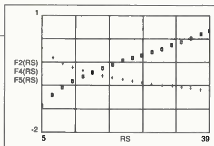
Figure 3. Sensitivities of R_S with respect to X_1 for standard tee (cross), series enhanced-Q L (square) and shunt enhanced-Q L (diamond) networks. R_L = 50 , Q = 5 .
