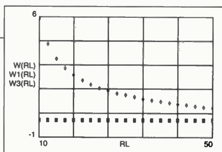
Figure 12. Sensitivities of R_L with respect to X_3 for pi (cross), mixed pi (square) and mixed tee (diamond) networks. R_S = 5 , Q = 5 .
