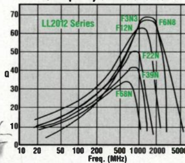
Q-Frequency Characteristics
