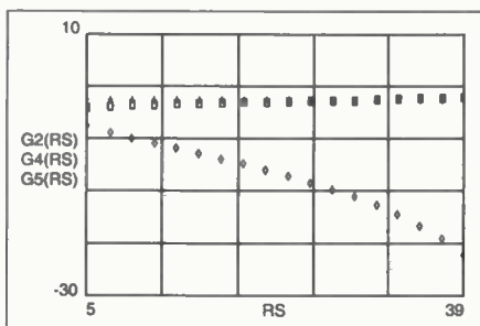
Figure 5. Sensitivities of R_S with respect to X_2 for standard tee (cross), series enhanced-Q L (square) and shunt enhanced-Q L (diamond) networks. R_L = 50 , Q = 5 .
