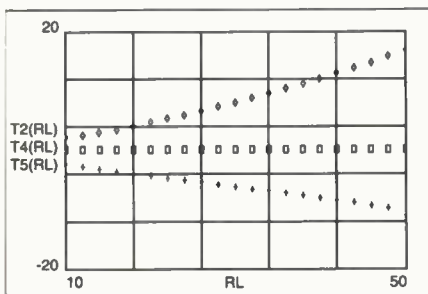
Figure 9. Sensitivities of R_L with respect to X_1 for standard tee (cross), series enhanced-Q L (square) and shunt enhanced-Q L (diamond) networks. R_S = 5 , Q = 5 .
