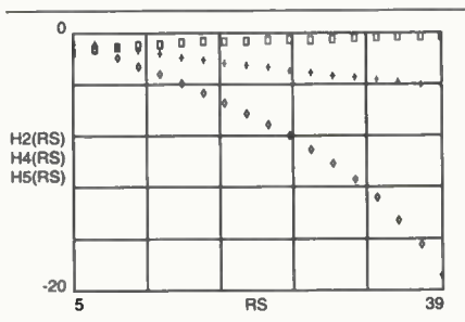
Figure 7. Sensitivities of R_S with respect to X_3 for standard tee (cross), series enhanced-Q L (square) and shunt enhanced-Q (diamond) networks. R_L = 50 , Q = 5 .
