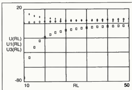
Figure 10. Sensitivities of R_L with respect to X_2 for pi (cross), mixed pi (square) and mixed tee (diamond) networks. R_S = 5 , Q = 5 .
