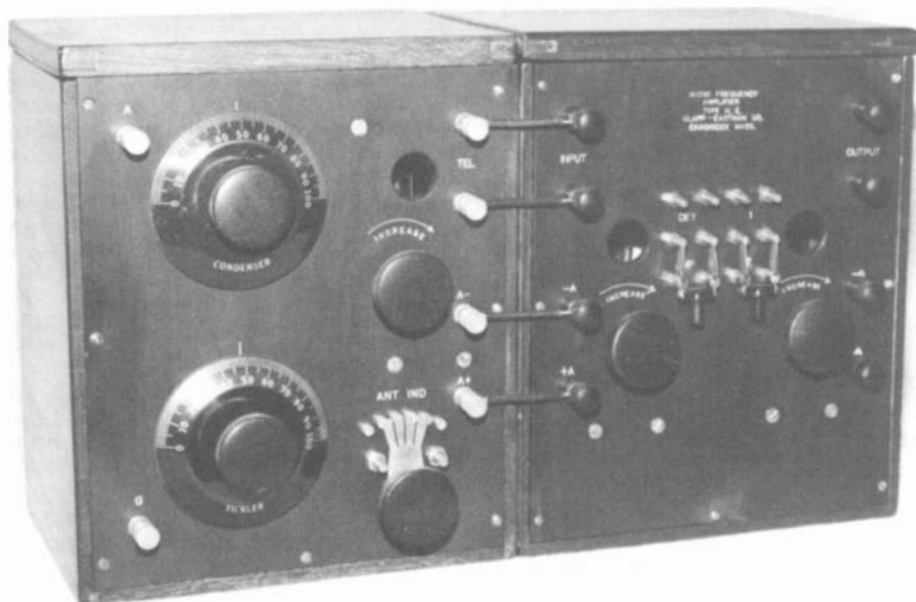
Figure 1. The Clapp Eastham HR (left) and the HZ (right).
