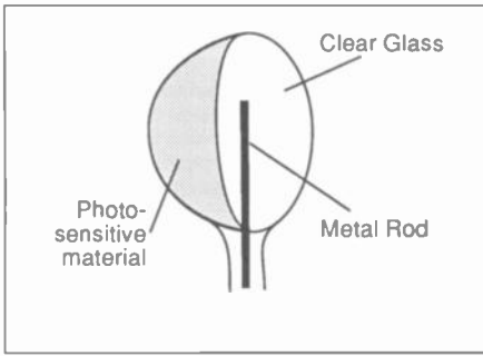
Figure 2. A photocell used in a 1930 mechanical TV.
