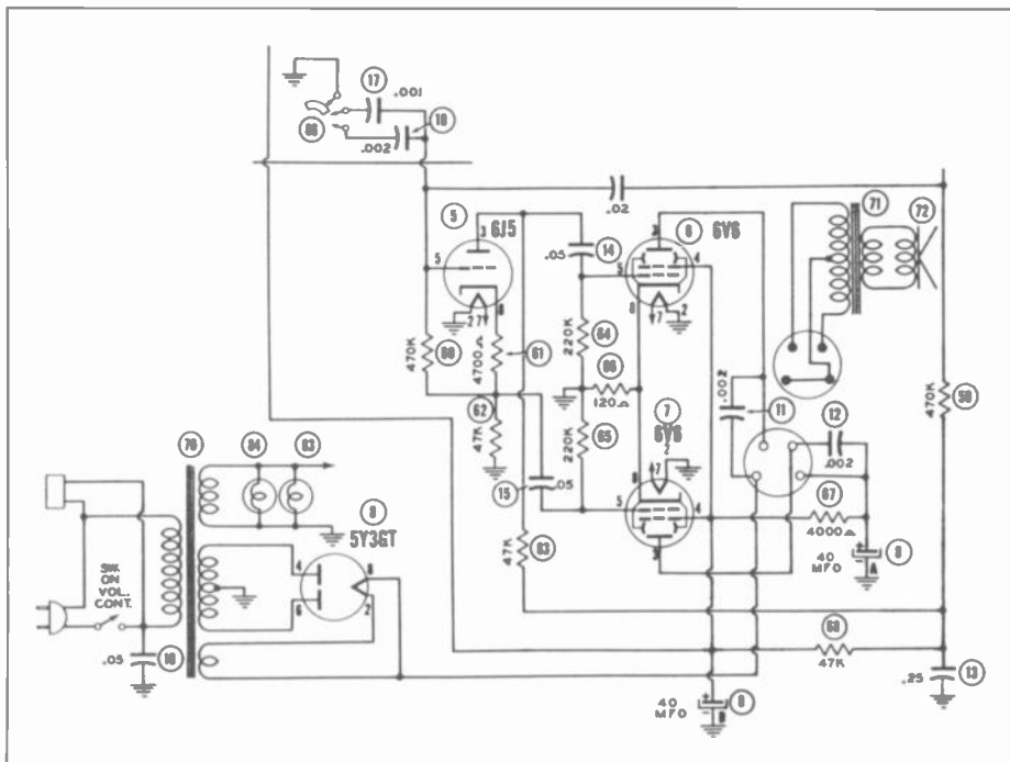
Power supply and audio circuit of a typical large AC radio.
