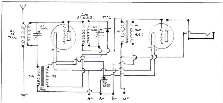
Figure 5. Schematic diagram of the Nyacoflex Model R2. (Courtesy of Scott MacWilliam).
