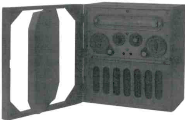
RADIOLA 26 - The Radio Corporation of America offered this two-dial Superhet portable in 1925. It used six UV199 tubes. Note the radio direction finding antenna in the door to the left. This "portable" was a hefty 35 pounds with batteries. (Larry Cannon - Fresno, CA)
