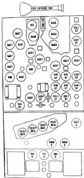
Figure 5. The location diagram of the 43 tubes used in the G.E. 901 projection television.
