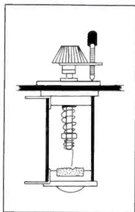
Figure 4. Cross section of the Nyacoflex crystal detector. (Drawn by Scott MacWilliam).
