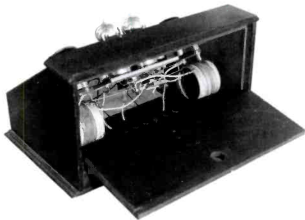
Figure 3. The Nyacoflex Model R2 with the rear access panel pulled down to expose the two-tube chassis.
