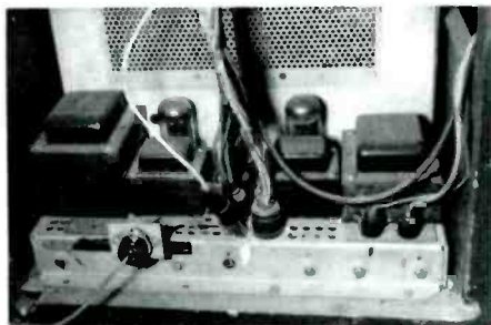
Figure 4. High voltage power supply for the G.E. Model 901 projection television receiver.
