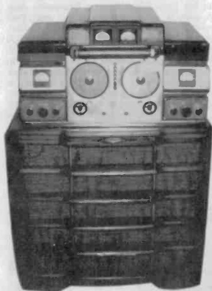
HALLCRAFTERS MODEL DD-1 – This late 1930s, single control, Dual-Diversity receiver has two complete RF, IF and second detector stages with a common local oscillator and audio stage. The radio selects the strongest signal to reduce shortwave fading. The power supply and audio amplifier are contained in a separate chassis. The set has 26 tubes and 3 "S" meters. (Joel Levine – Greenlawn, NY)
