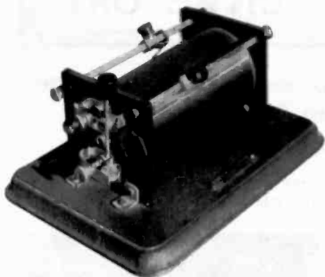
STAR CRYSTAL SET — This catwhisker and galena crystal receiver was manufactured by the Star Mfg. Company of Turtle Creek, Penn. It has a 1922 red and gold seal of approval from Radio News . Tuning is done by the double slide contacts on the red-enameled wire coil. (Dave Crocker — Mashpee, MA)
