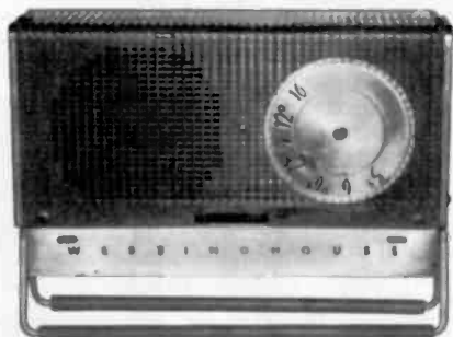
WESTINGHOUSE MODEL H-493-P4 — This Art Deco portable uses subminiature tubes—Types 1V6, 1AH4, 1AJ5 and 1AG4. Measurements are 6-inches long, 3 3 / 4 -inches high not including the handle, and 1 3 / 4 -inches deep. (Francis Buren — Postville, IA)
