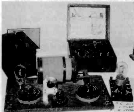
This A.C. Gilbert display in the Tuska seminar on Saturday consists of a board-type crystal set, a boxed crystal set, and a 1-tube Audion detector stand.
