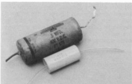
Figure 11. Modern capacitors with plastic film dielectric are much smaller than the old paper dielectric capacitors.
