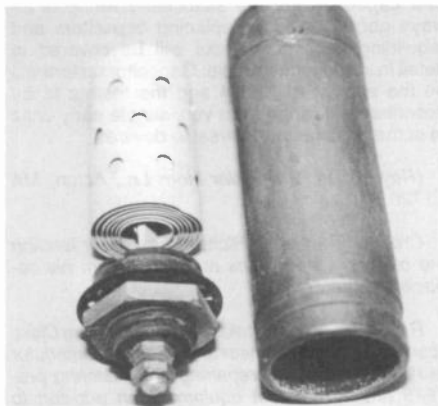
Figure 8. A copper, can-type, wet electrolytic capacitor from a Philco radio.
