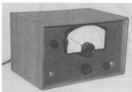
Figure 7. A 2-band version of the 1-tube superheterodyne, using plug-in coils.
