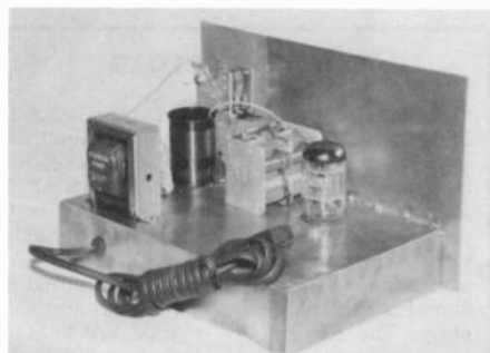
Figure 6. The Multivalue Receiver No. 3 superheterodyne, using a Type 6AS11 Compactron.
