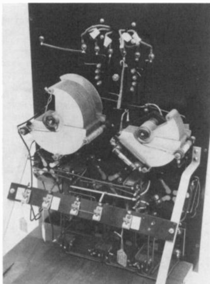
Figure 6. Interior view of the Universal Receiving Set.
