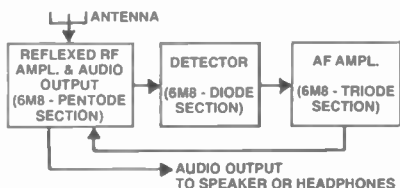
Figure 4. Simplified block diagram of the "Modern" Multivalue Receiver #1.
