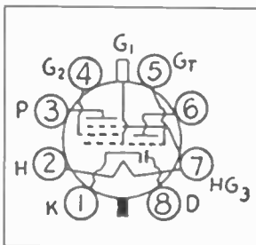
Figure 1. The base diagram for the Type 6M8GT tube.
