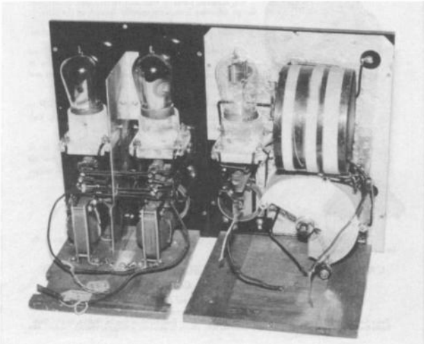
Figure 4. Interior view of the SC-10 receiver and the Type S amplifier.
