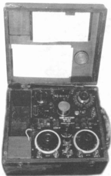
MARK III SHORTWAVE SET – This 1918 World War I crystal receiver was manufactured by Johnson and Phillips Ltd., of London. It was used in the trenches by the military. Operation is by a perikon type detector. (Jim Taylor – Bournemouth, England)
