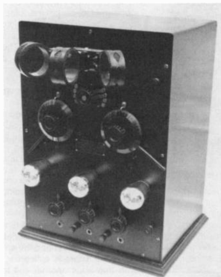
Figure 5. Front view of the Universal Receiving Set.
