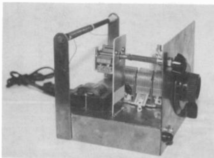
Figure 2. A side view of my first attempt to use the 6M8GT in an TRF circuit. The set actually worked!
