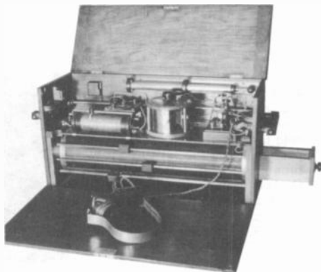
Figure 2. The 1910 crystal receiver with a secret past.
