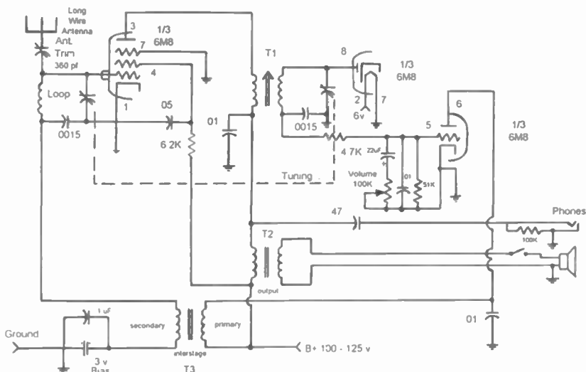
Figure 3. A schematic diagram of the "Modern" Multivalue Receiver No. 1. This TRF set employs reflex circuitry. In this reflex circuit, the desired signal is selected with the tuning capacitor and coupled to the grid (via the grid cap) of the RF amplifier — the pentode section of the Type 6M8 tube. The amplified RF signal (pin 3) is coupled to the detector via the RF transformer (T1). The detected AF signal is sent to the grid (pin 5) of the triode section where it is amplified. The amplified AF signal is fed back to the grid of the pentode section through the audio interstage transformer (T3). Now the pentode section functions as an AF amplifier. The amplified AF signal (pin 3) is fed to either the speaker via the audio output transformer (T2) or via the 0.47 mF capacitor to the headset.
