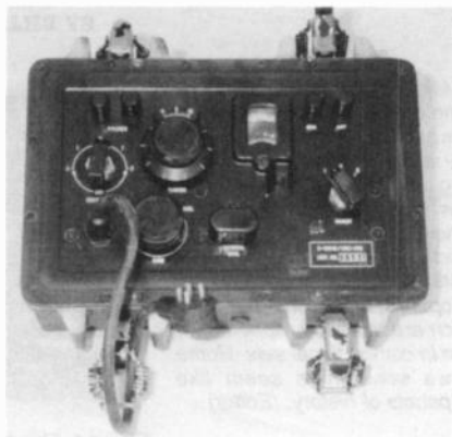
The R1004-A/GRC-109 receiver showing the power cable and crystal socket near the bottom center of the front panel.
