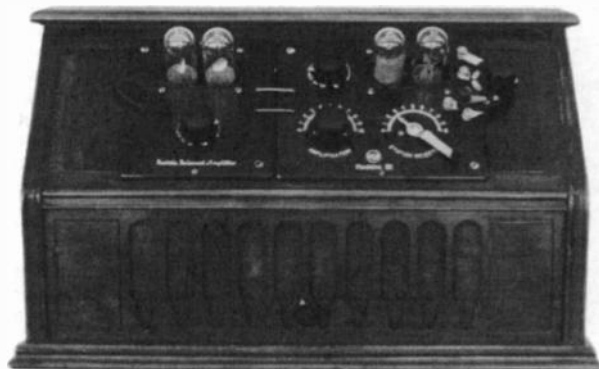
RCA RADIOLA III – This Radiola III is set in an original ACRE Deluxe cabinet, which includes the 2-tube RCA balanced amplifier and built-in speaker below. The radio operates on (4) Type WD-11 tubes, but could use Type UX-199 or Type 230 tubes with WD-11 adapters. When these substitute tubes are used, the knob at the bottom of the grille controls the filament current. (Ross Mason – Mason City, IA)
