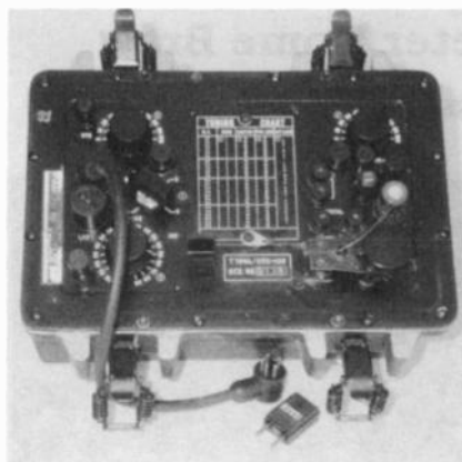
The T784A/GRC-109 transmitter has the controls and tuning chart on the front panel. The power cable extends from the front panels. A typical crystal is in front of the unit. A built-in key is mounted on the bottom right corner of the unit.
