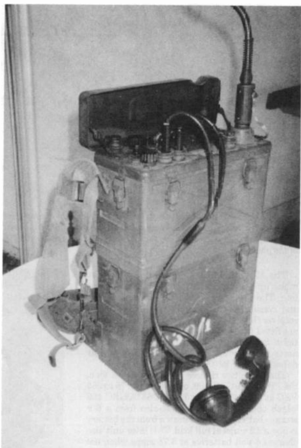
The SCR-300-A is shown with the antenna attached, the handset plugged into the set, and the battery box on the bottom. Carrying straps for backpack operation are attached.
