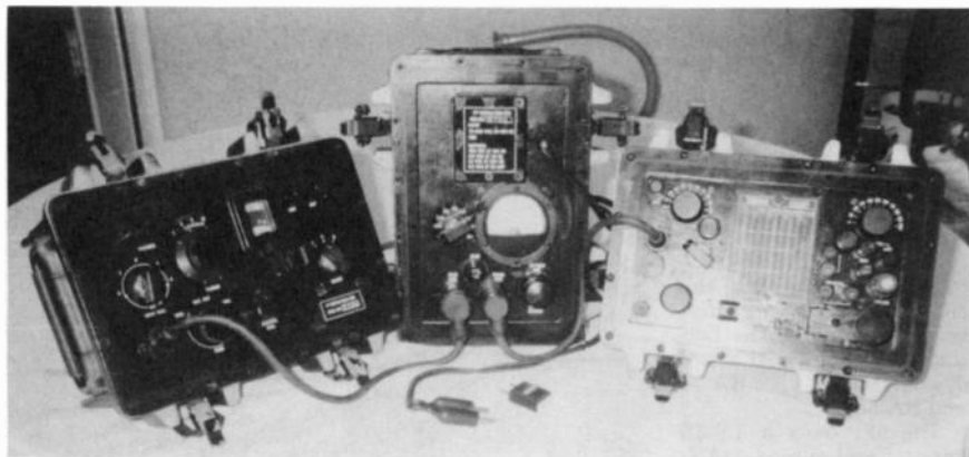
The AN/GRC-109 components, left to right: receiver, power supply for AC operation, and transmitter. An antenna and headphones would complete this installation. AC power can range from 40 to 400 cycles at voltages from 70 v to 240 v. Note the large, round, 2-pin power plug (as used in Europe) on the power cord in the photograph.
