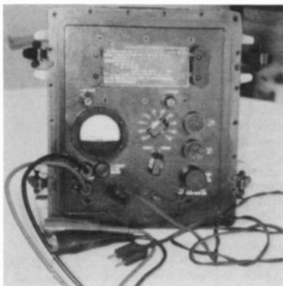
The AN/GRC-109 power supply for 6 Vdc or AC operation. This unit is larger than the AC-only power supply. Note the AC cord and battery cables. This unit can operate from 6 Vdc input or can be used to charge a 6-volt battery when not operating the radio sets.
