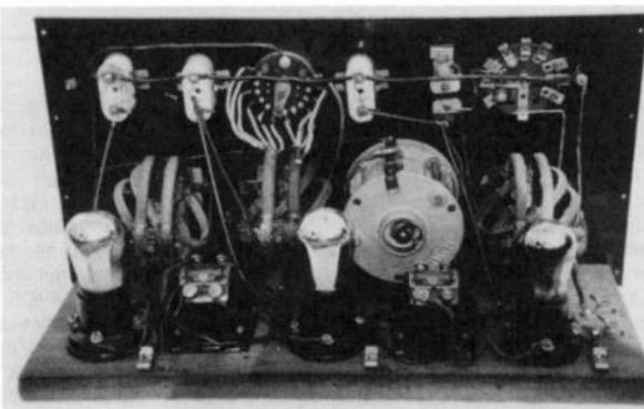
Figure 2. A rear view reveals the neat construction and layout, as well as the author's fine restoration.
