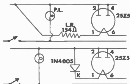
Figure 2. These "Before" (top) and "After" (bottom) schematic diagrams show the use of a solid-state rectifier as a resistance line cord substitute.
