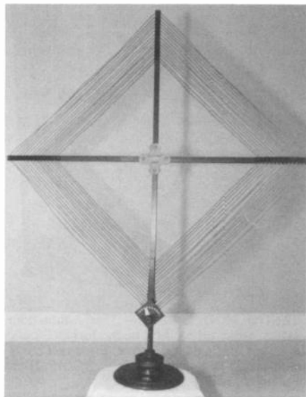
Figure 1. Korach Loop Antenna manufactured by the Hermanson Manufacturing Company.
