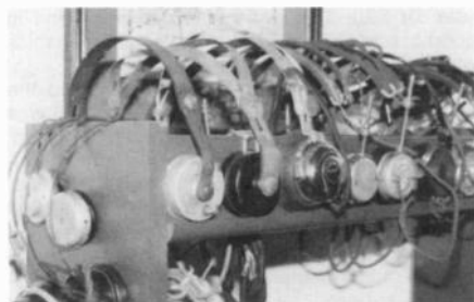
Figure 2. This close-up view of a rack shows some construction details.
