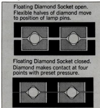
Floating diamond four point contact socket
