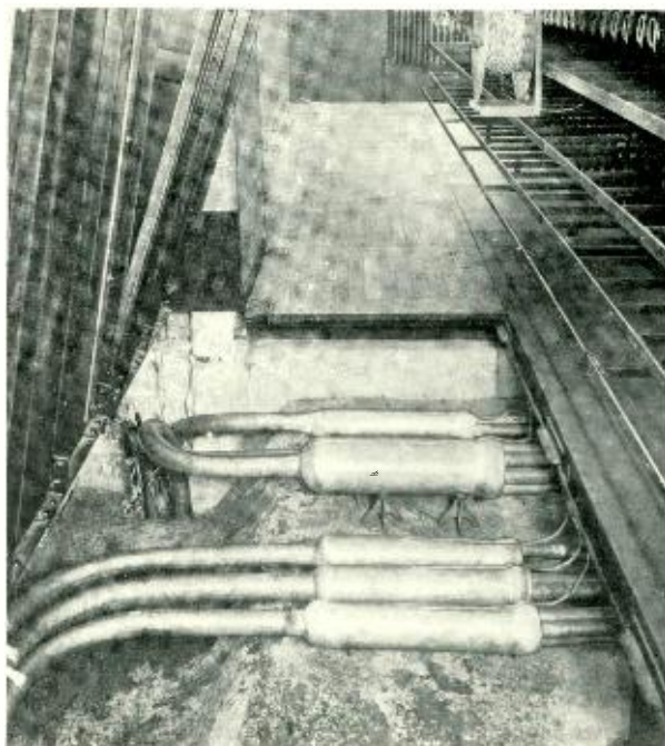
Fig. 6—The fourth cable from the bottom shows an 1800-pair cable spliced to nine 200-pair cables for distribution to the main frame
