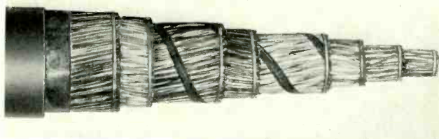
Fig. 1—A short length of 1200-pair cable showing layered construction
