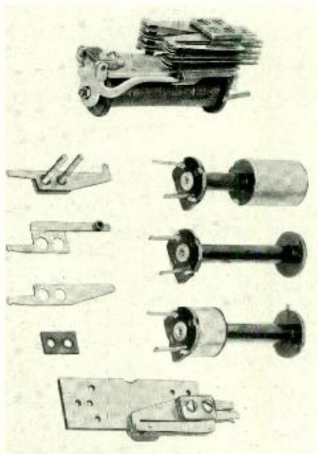
Fig. 1—The elements from which an indefinite number of step-by-step relays may be built up are here shown both individually and assembled into a typical relay
