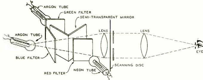
One semi-transparent mirror reflects red light from the neon tube; one reflects green light from one argon tube; and through both mirrors passes blue light from the other argon tube
