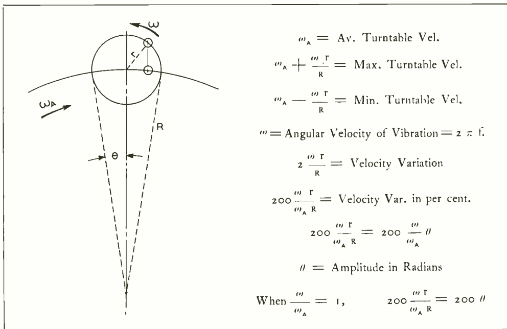
Fig. 9—Method of converting stroboscope micrometer reading to per cent velocity variation. The curve of large radius represents the rim of the turntable, and the curve of small radius represents the familiar diagram of harmonic motion. At the projection of the end of the small circle's radius is a groove on the turntable rim. The quantity read on the micrometer is 2r ,—the maximum motion of a groove
