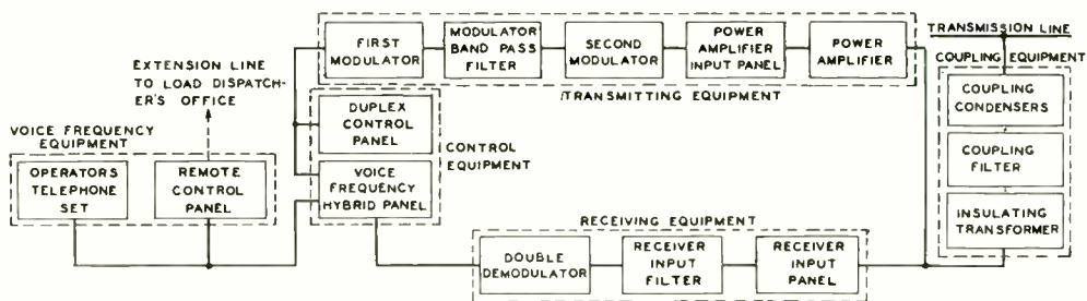
Fig 2—Block schematic of the carrier system
