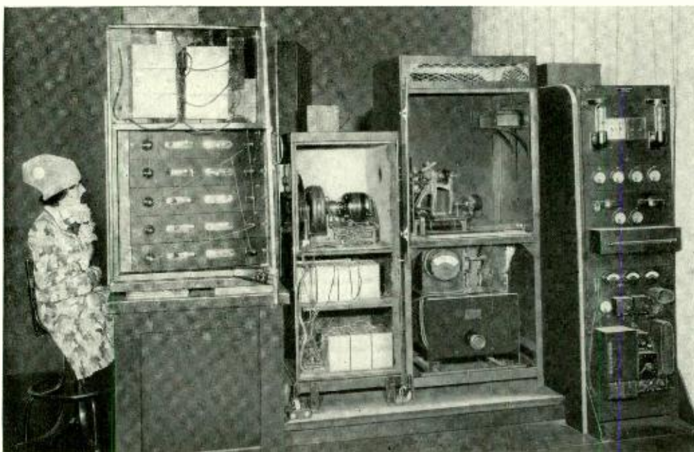
Side view of sending apparatus with doors of cabinets opened. With the exception of the photoelectric cabinet at the left, the apparatus is identical with that used for the original demonstration of monochromatic television
