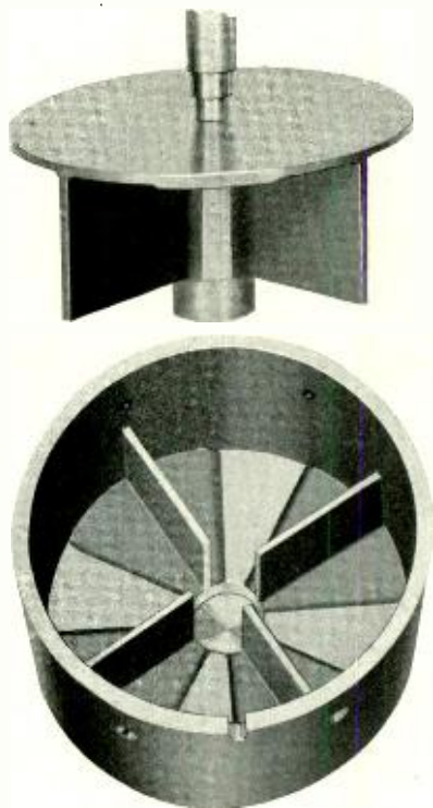
Fig. 5—The oil-damping connection between gear and turntable shaft. Above, oil cup; below, vane-bearing end of turntable shaft
