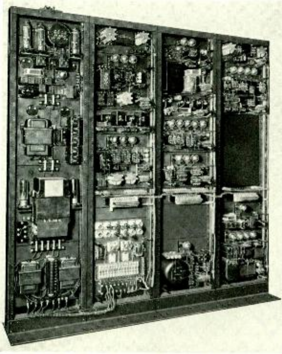
Fig. 5—Terminal equipment—rear view
