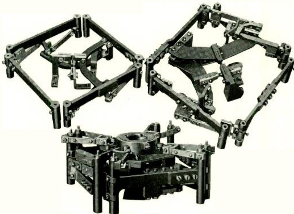
Fig. 8—Steps in the development of the linkage, showing its successively more rugged construction
