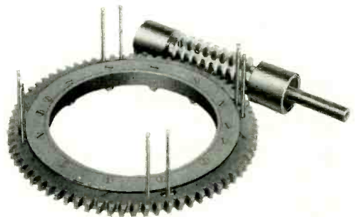
Fig. 3—The reduction gearing: a worm and a four-layer worm-wheel
