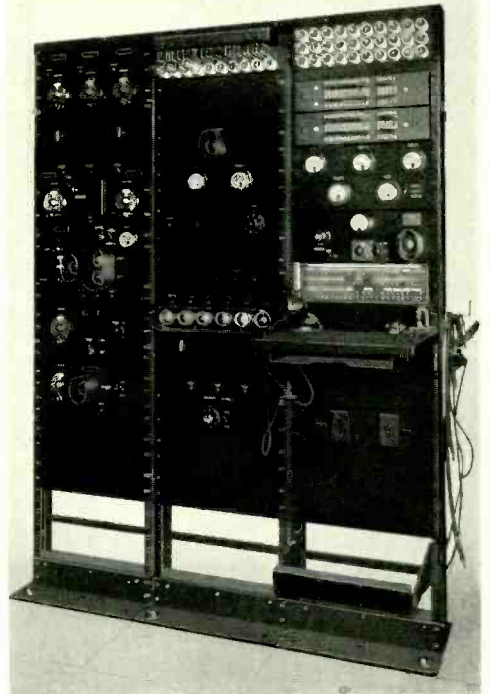
One of the short-wave receivers at Netcong. The monitoring operator's position is at the right-hand panel
