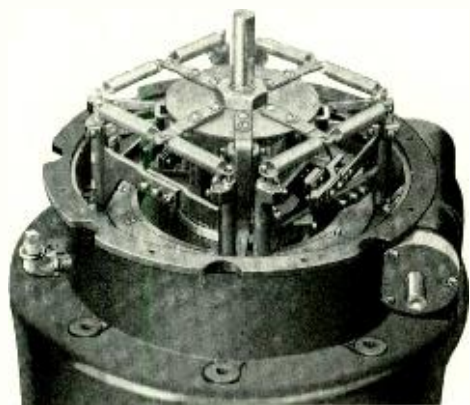
Fig. 4—The spring connection between gear and turntable shaft
