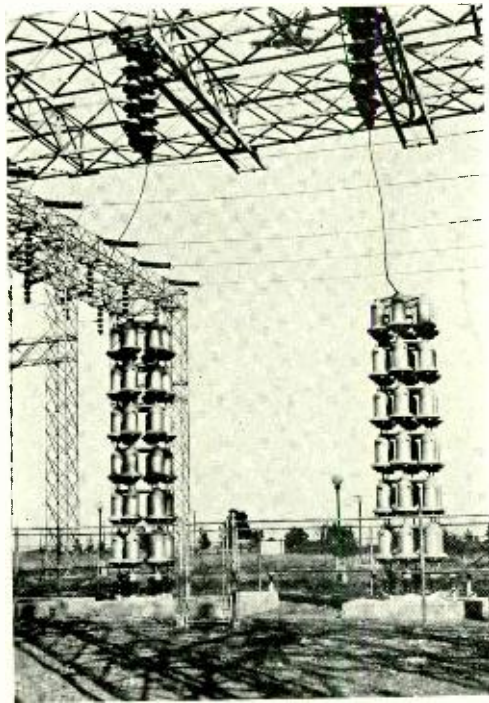
Fig. 4—Coupling condensers for 220,000 volt lines
