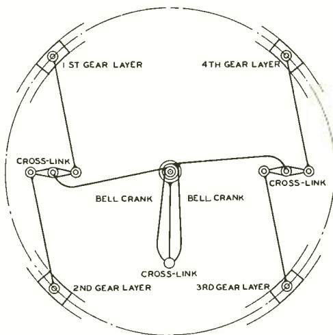
Fig. 7—Schematic diagram of linkage. The bell-cranks are pivoted at the center of the mechanism but are not attached to the shaft. The third cross-link, between the ends of the bell-cranks, is perpendicular to the plane of the diagram. From its center extends the only member which has a rigid connection at the center of the mechanism, to the collar which drives the oil cup
