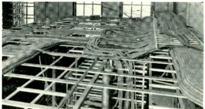
Switchboard cables at Lansing; this view shows how the smaller and more flexible cables may cross each other in several planes
