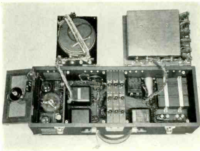
Interior of 3-B measuring set
