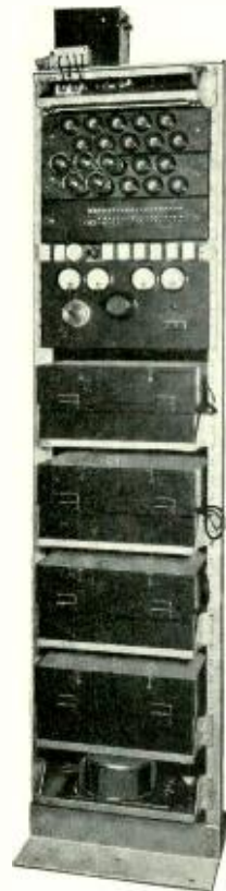
Fig. 3—The 200-milliamperere, 130-volt plant. At the top is the Tungar rectifier; next come the resistance lamps and fuses. The relays are for automatic charging and voltage control. In the four lower boxes are the storage cells
