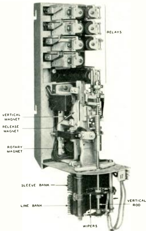
Fig. 1—On this photograph of a regular connector we indicated the essential operating elements
