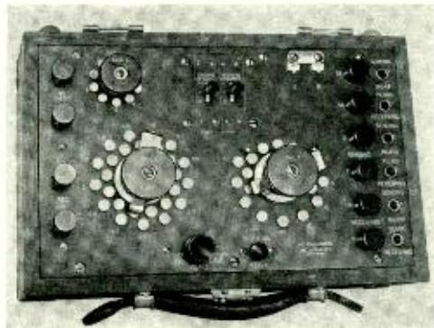
1-C measuring set, of acoustic balance type
