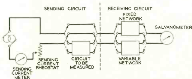
Fig. 2—Meter-indicating type of transmission measuring circuit
