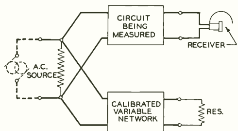
Fig. 1—Acoustic balance type of transmission measuring circuit
