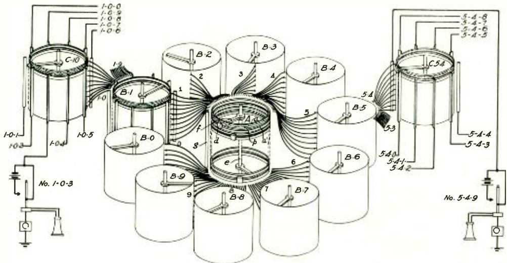
Fig. 3—A patent granted to J. W. McDonough discloses features more nearly allied to the trend taken by later development
