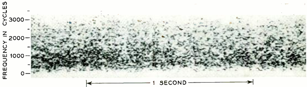
Fig. 5—Spectrogram of fluctuation noise alone
