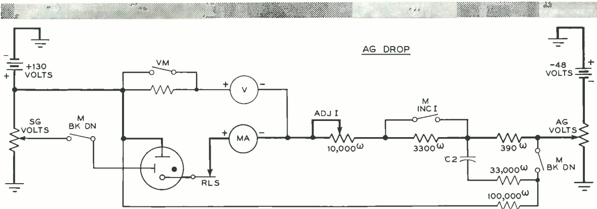
Fig. 4—Test circuit with key in "DROP" position
