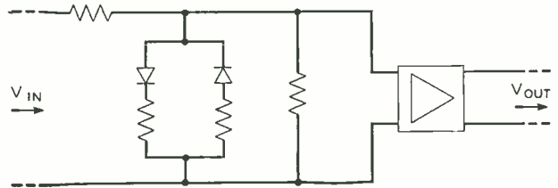
Fig. 2—This simplified schematic shows the essential elements of the compressor. It contains, besides the shunt and series resistors, two varistors oppositely poled and bridged across the circuit
