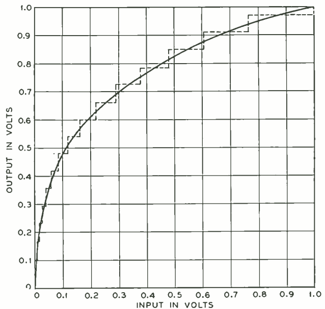
Fig. 3—Compressor characteristics, solid line, in terms of its input and output voltage. The dashed lines show quanta. For low values of input voltage, a variation in the input produces a relatively large change in the output, but for larger values of input, a change in input produces comparatively little change in output
