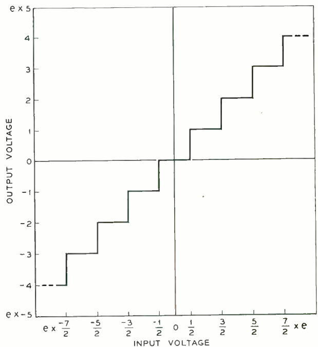
Fig. 1—Staircase characteristic representing quantization
