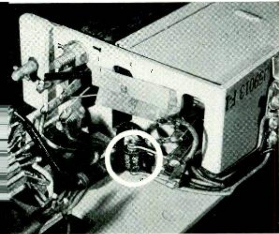
Fig. 1—A central-office trunk circuit of the 555 PBX showing a 400B germanium varistor used to reduce the potential on the cord sleeve when the plug is removed from the jack
