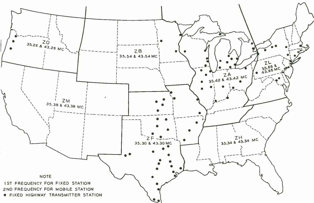
Fig. 1—Land stations and zones for the highway mobile radio-telephone system
