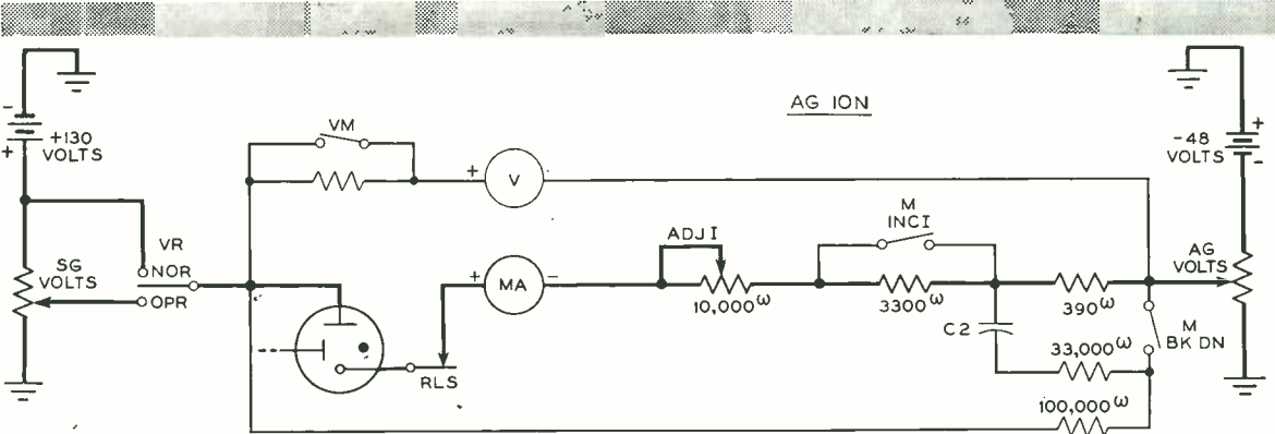
Fig. 3—Test circuit with key in "ION" position
