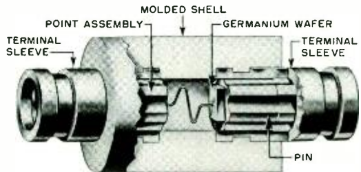
Fig. 2—Cut-away view of a 400 type varistor
