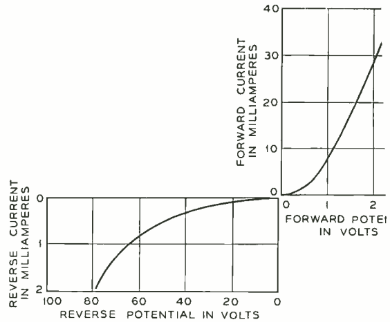
Fig. 3—Voltage-current characteristic of the 400A varistor
