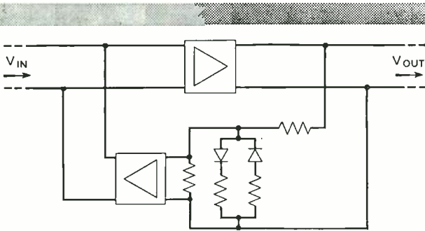
Fig. 4—Simplified schematic of the expander circuit
