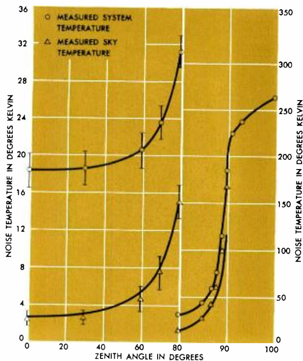
System and sky noise vary according to zenith angles. Theoretical calculations agree closely with those obtained from actual sky measurements.
