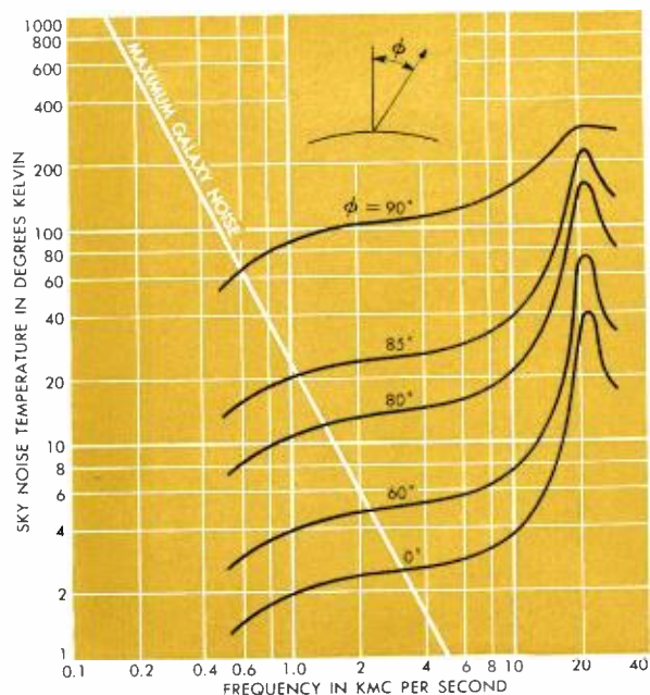
Galaxy noise decreases with increasing frequency; noise emanating from earth sources increases.
