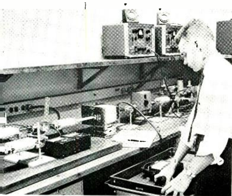
A. R. Johnson shown adjusting a complete 1A Isolator. Alternating current is used to stabilize the magnets to the operating values so that the magnets will remain permanent during years of use.
