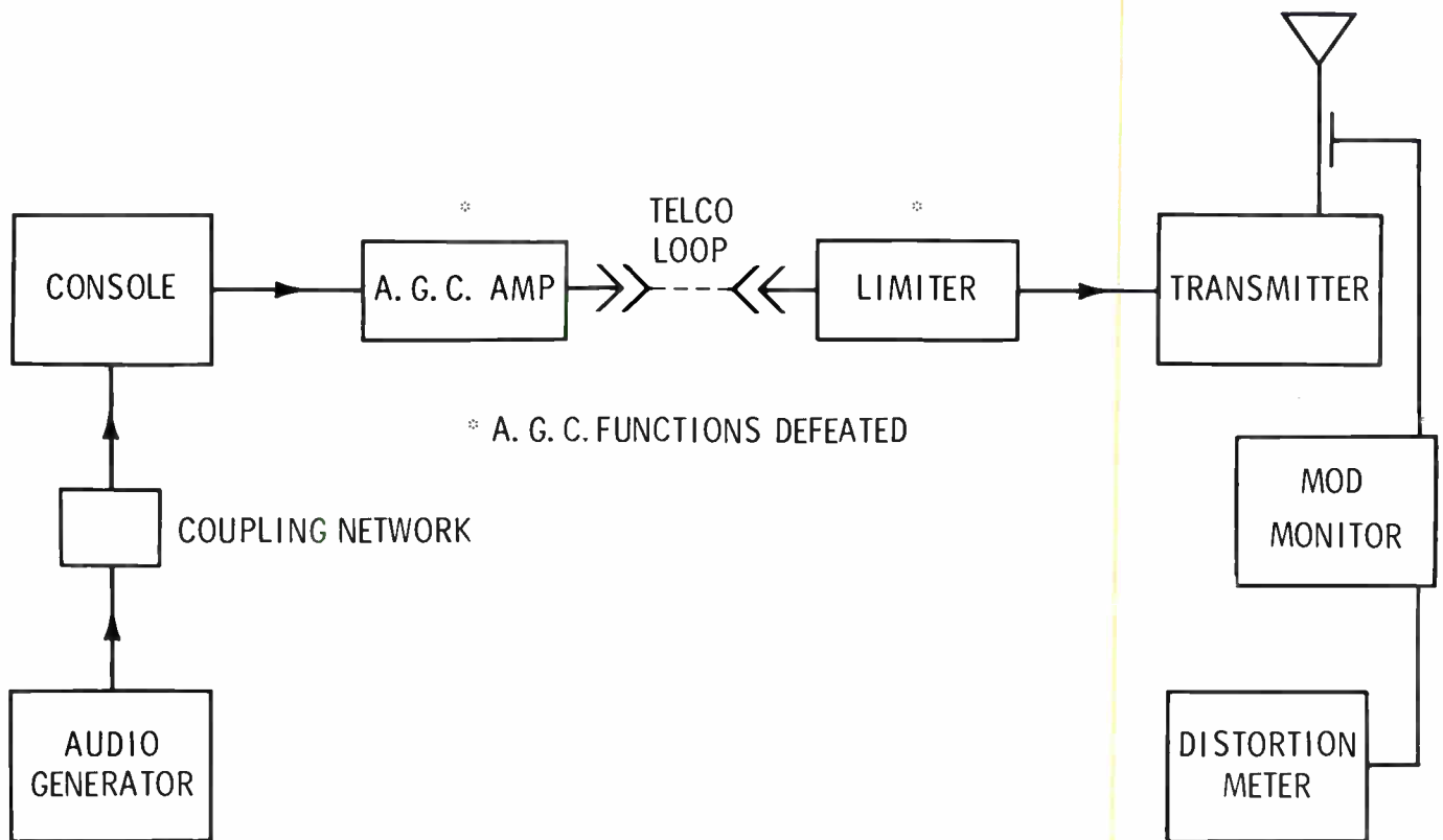
Figure 3a. Sample test equipment connection diagram.
