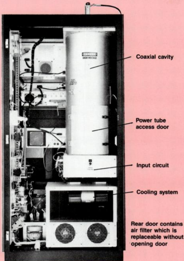
Rear view FM-5A Transmitter shows accessibility and excellent mechanical arrangement.
