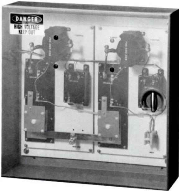
LEA Dynatech Heavy Duty Surge Eliminator
