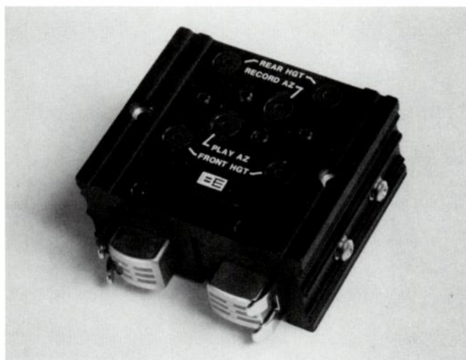
Phase Lok V Head Block
