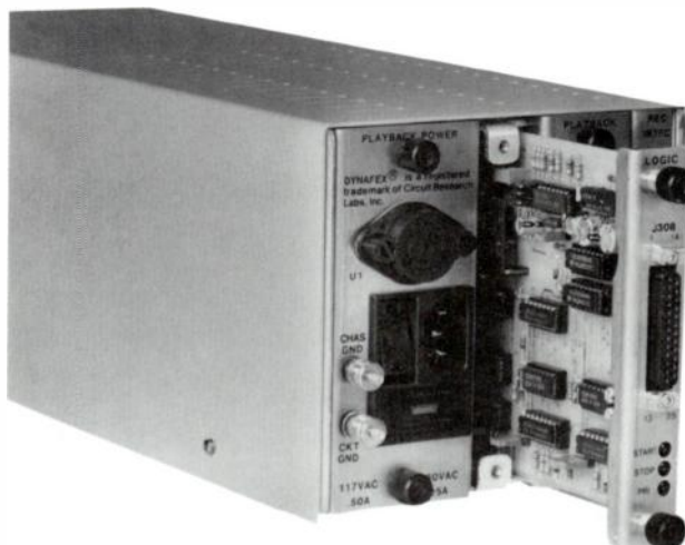
PHASE TRAK 90 PLAYBACK Modular Construction
