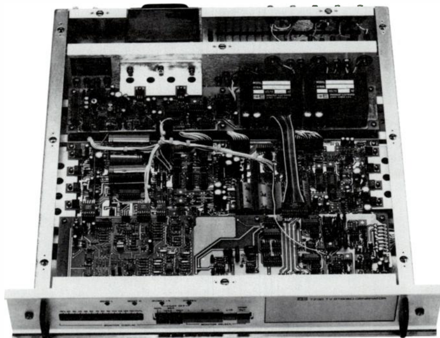
TZ-30 Internal View
