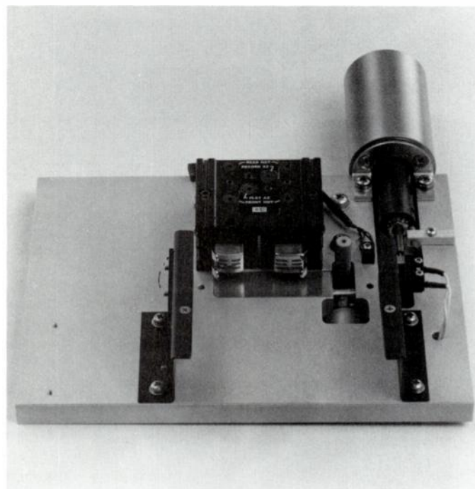
5300C Deck Assembly
