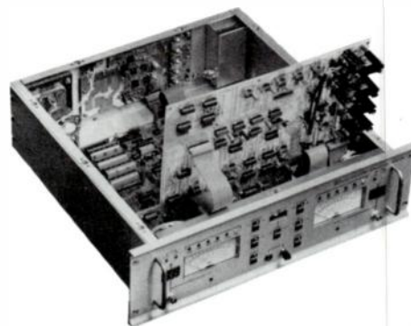
AS-10 Internal View
