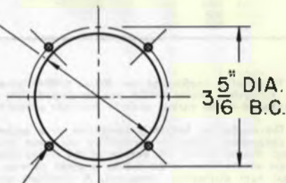
CHASSIS DRILLING
