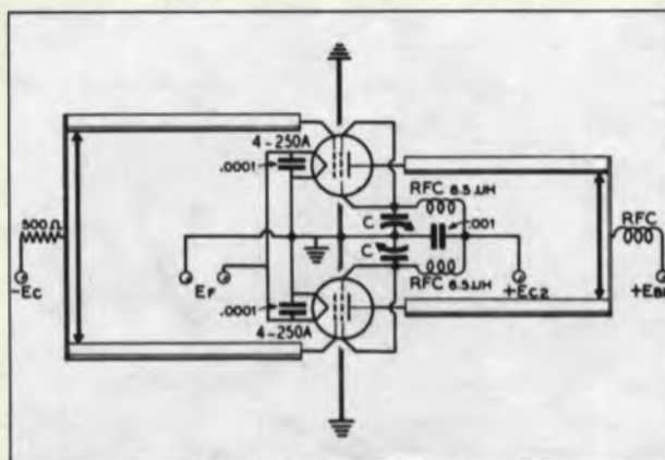
Screen-tuning neutralization circuit for use above 45 Mc. C — Approximately 100 \mu fd. per section, maximum.
