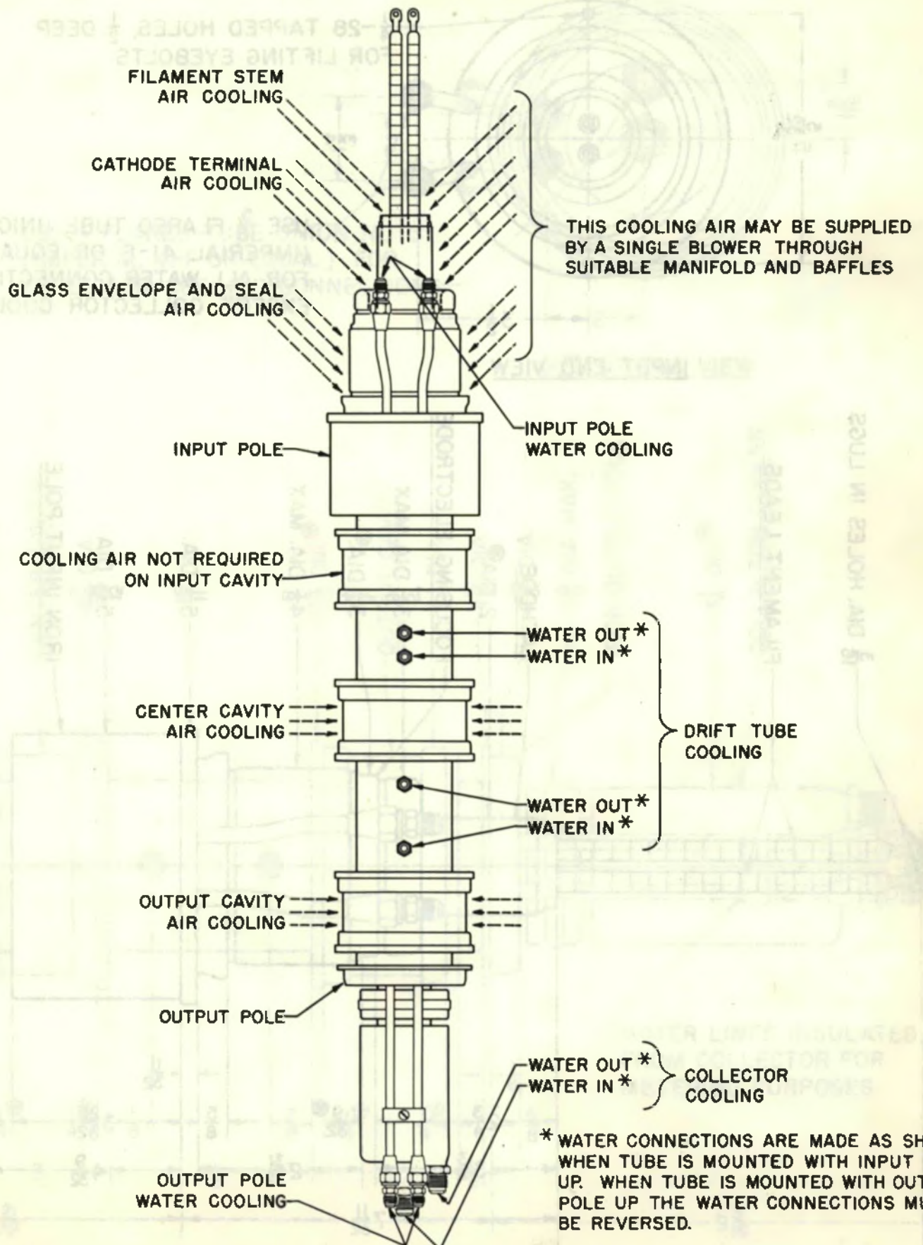
COOLING DIAGRAM
