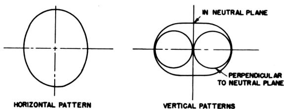
Fig. 4. Horizontal and vertical radiation patterns of simple loop antenna
