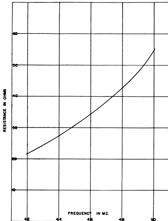
Fig. 10. Resonant resistance of circular antenna over the FM range when mounted on a 4-in. steel pole. (Includes leads and transmission-line insulators)
