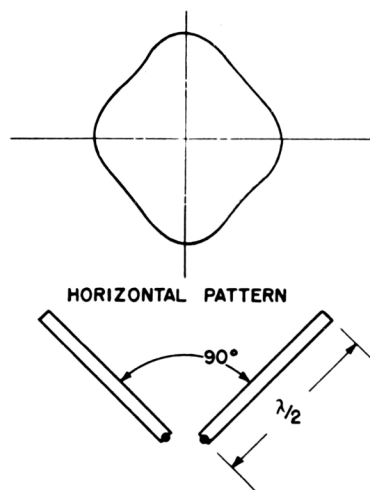
Fig. 2. The 90-deg "V" antenna and its horizontal radiation pattern
