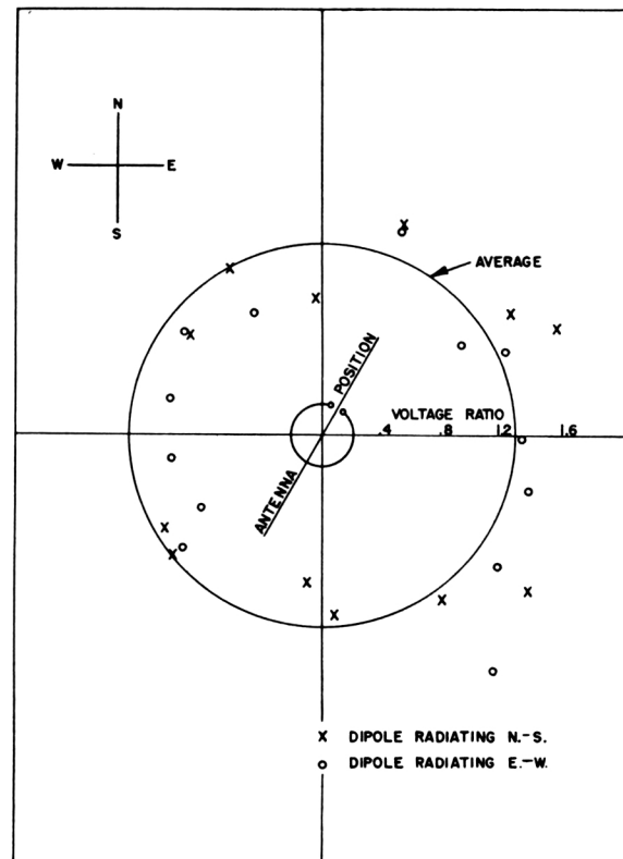
Fig. 14. Field measurements on a 2-bay FM circular antenna at 46.7 megacycles. (Compared with a dipole)
