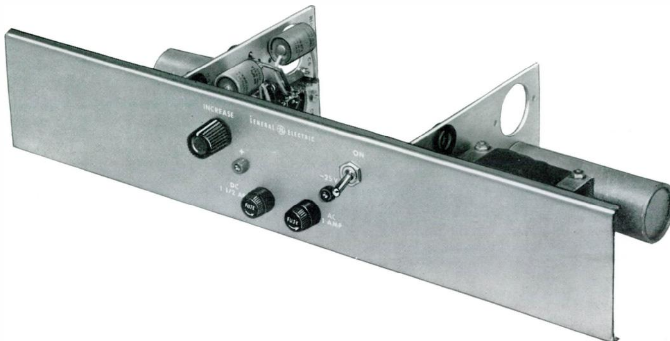
Type BP-20-A 25-Volt Transistor Power Supply (Regulated)
