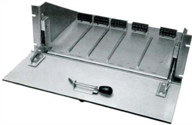
Front view of FA-23-B Shelf, with front panel open.
