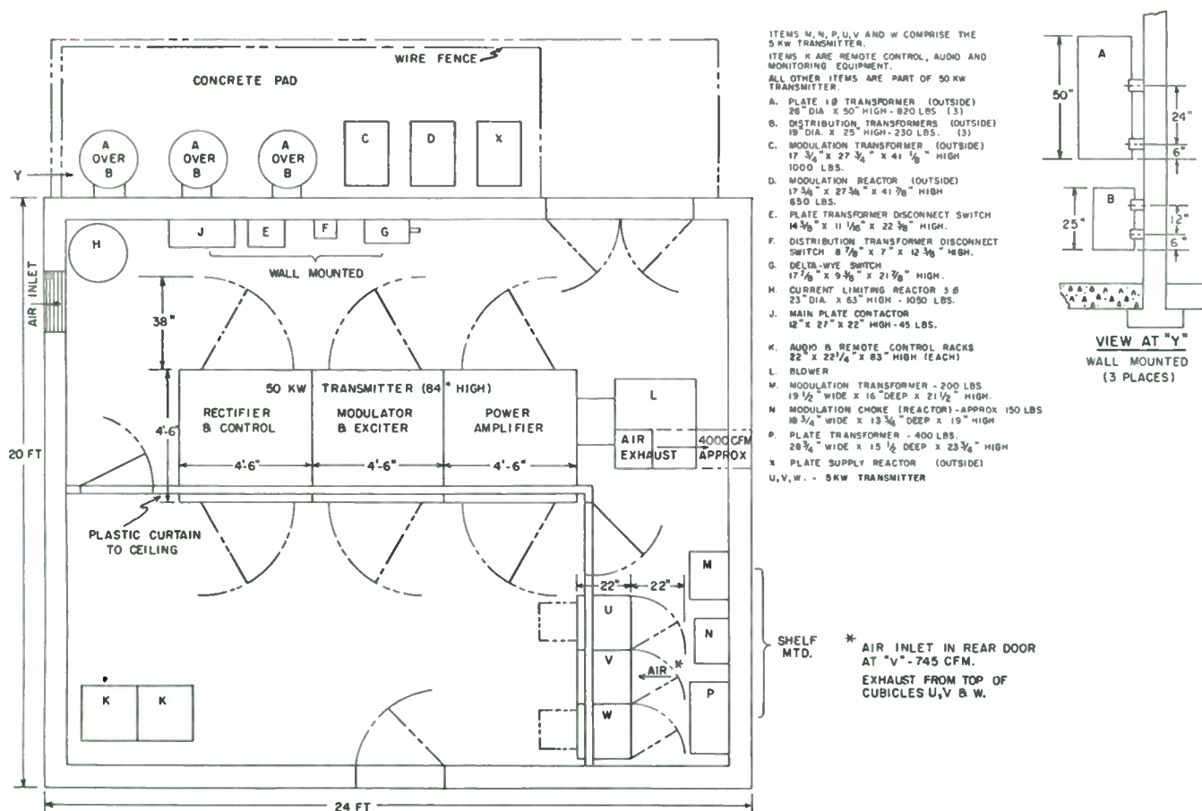
Typical Station Layout 50 KW AM Broadcast Transmitter with 5 KW Standby and Conelrad Transmitter
