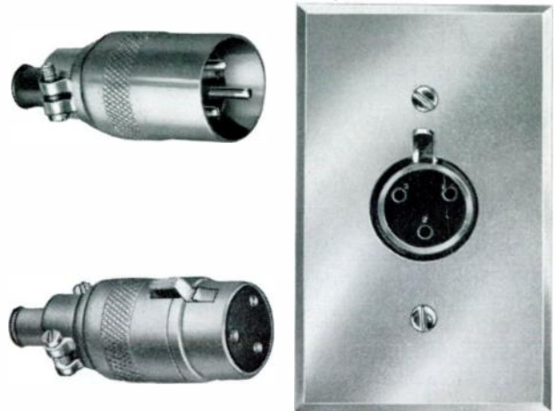
Type FA-16-A Male Microphone Plug, Type FA-16-B Female Microphone Plug, and Type FA-16-C Microphone Wall Receptacle
