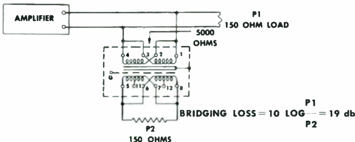
Installation Drawing for FA-41-C Transformer
