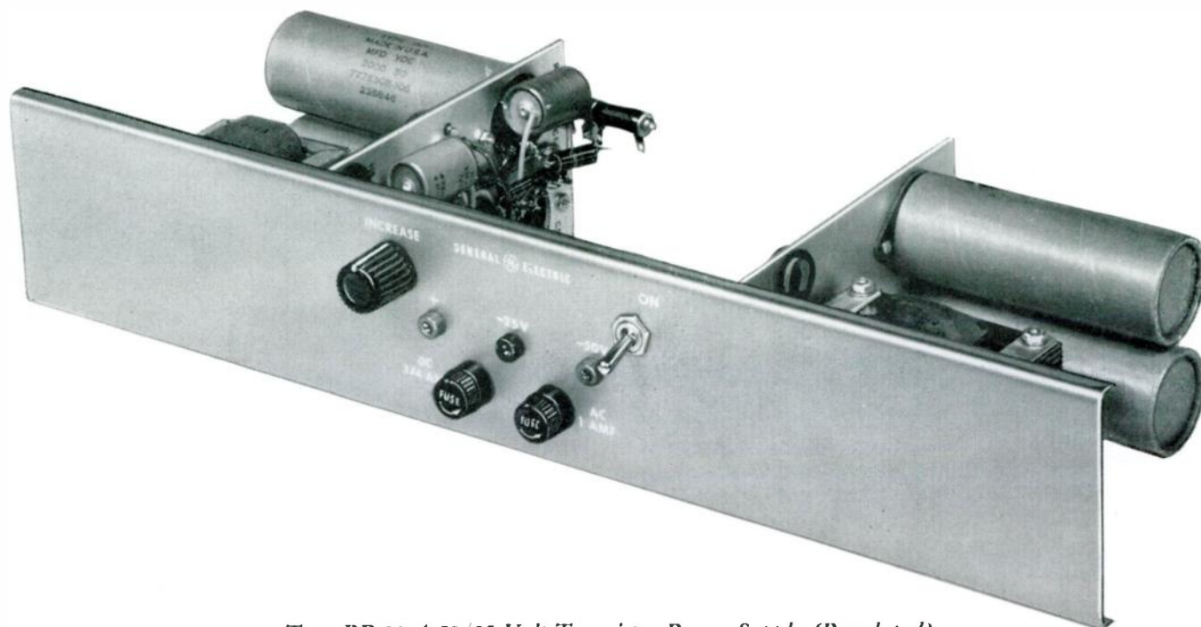
Type BP-21-A 50/25-Volt Transistor Power Supply (Regulated)
