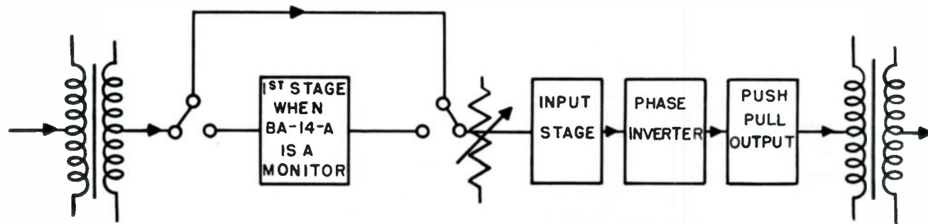
Block diagram of BA-14-A Program/Monitor Amplifier, shown connected as a program amplifier.
