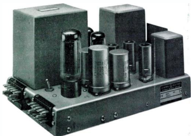
Rear view of BA-14-A Amplifier, showing plug-in construction.
