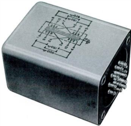
G-E Line-To-Line Transformer, Type FA-40-B
