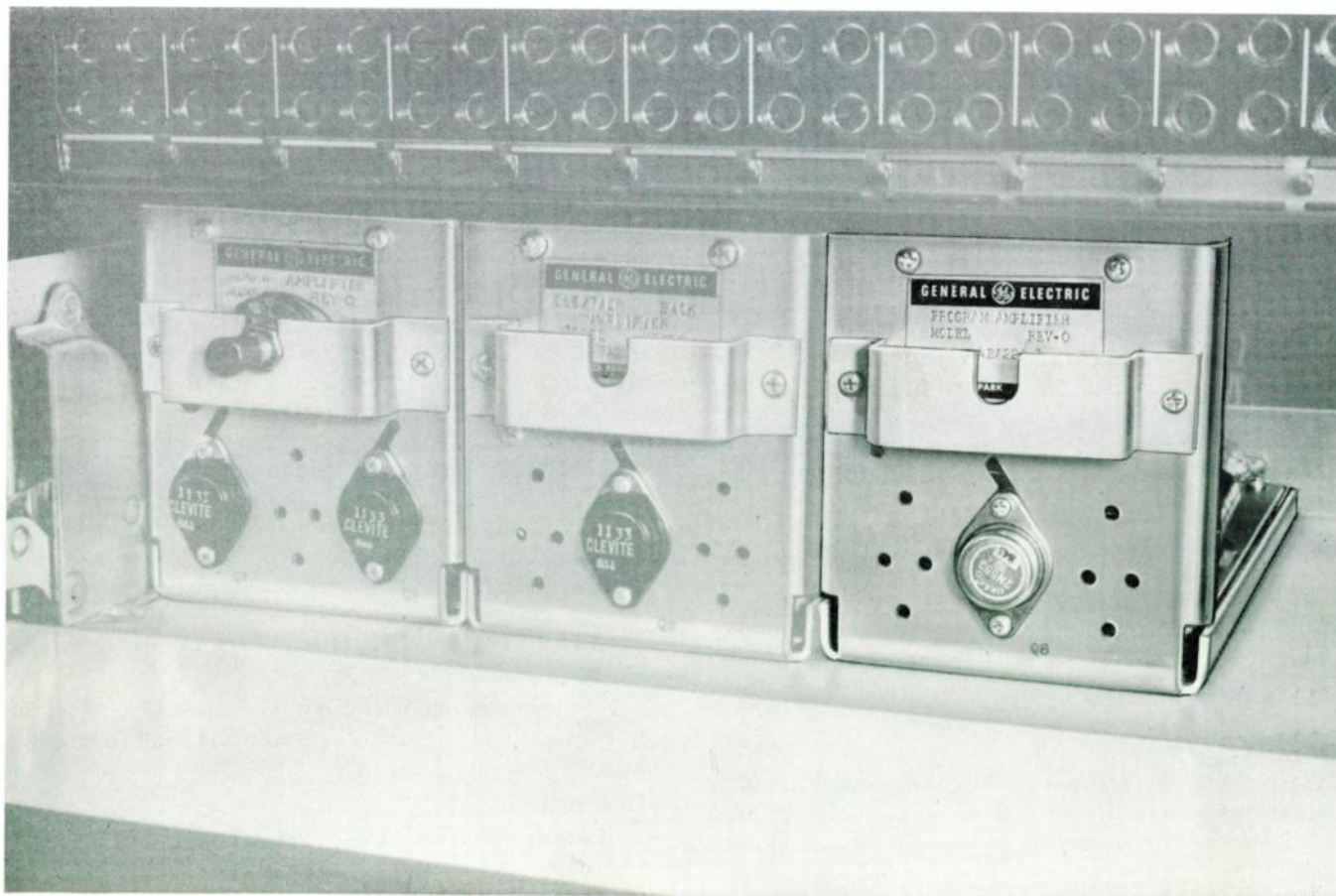
Type BA-22-A Program Amplifier installed in a Type FA-48-A Equipment Shelf.
