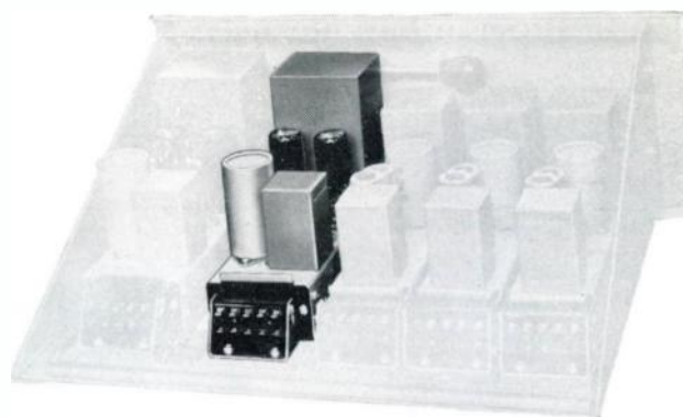
Plug-In Program/Monitoring Amplifiers, Type BA-12-C and Trays, Type FA-22-E; plus Plug-In Pre-Amplifiers, Type BA-1-F mounted in Broadcast Shelf, Type FA-23-A.
