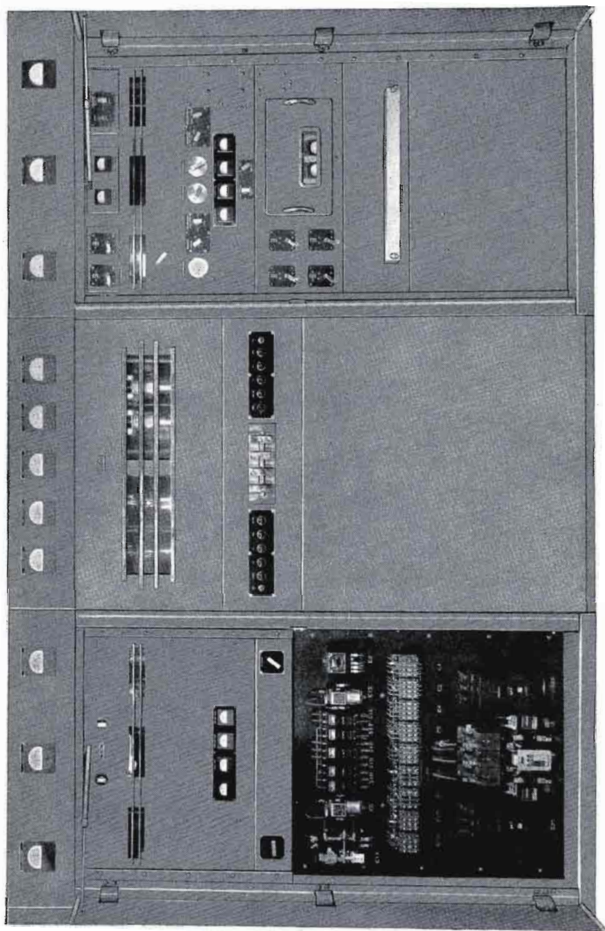
Front view (doors open) of Gates 5000 and 10,000 watt high frequency transmitters, Models HF5 and HF10.
