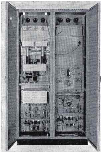
Rear BT100A view. Left cabinet contains visual and aural power amplifiers, visual exciter, modulator and power supplies. Right cabinet, demodulator, aural exciter, control and protective panel and power supplies.
