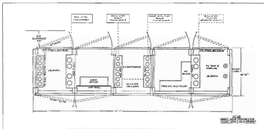
Floor plan of 20KW medium or short wave models.
