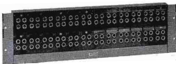
Left, one C-1500 jack panel mounted on PD1 jack mat. Has 48 jacks (24 pairs). Panel size: 3 1/2"x19".
