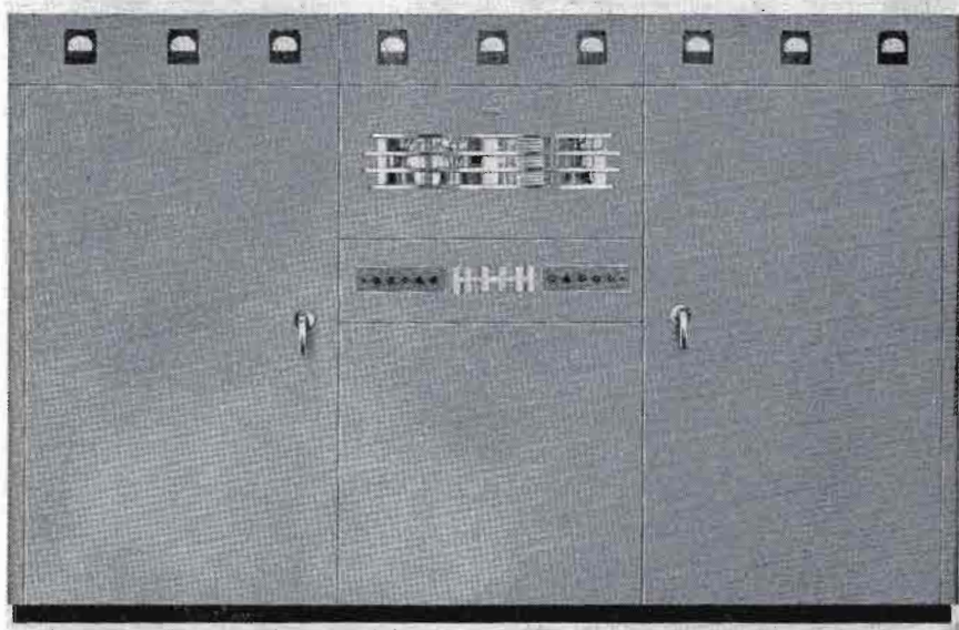
With front doors closed, all tuning controls are fully protected. Dead front design permits opening doors at any time for touch-up tuning and checking.
