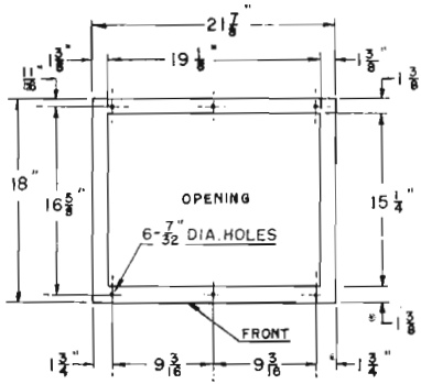
BASE DIMENSIONS, RAK-1 RACK
