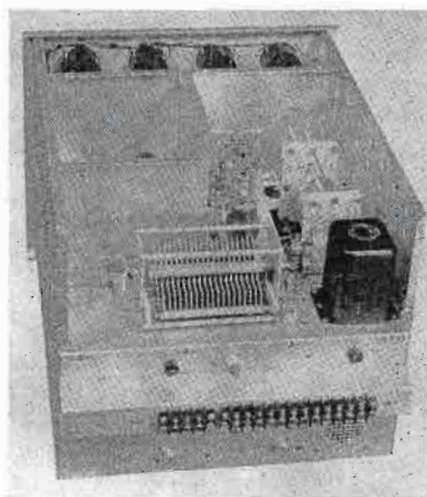
Above: Radio frequency chassis (top deck) with cover removed.
