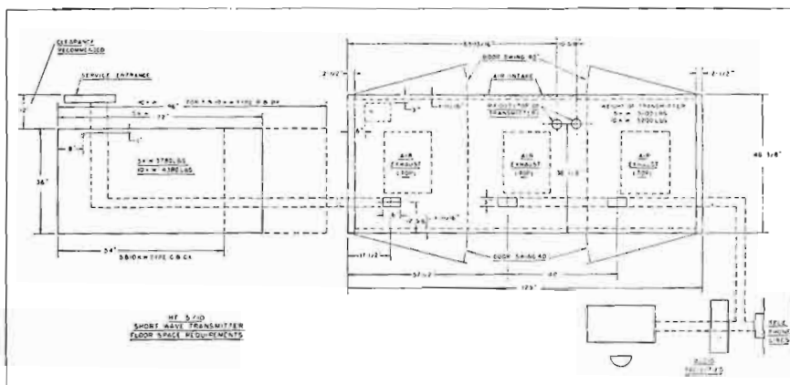
Floor plan shows location and size of transmitter and external modulator/power components. External components may also be mounted in basement or in out-building if desired.
