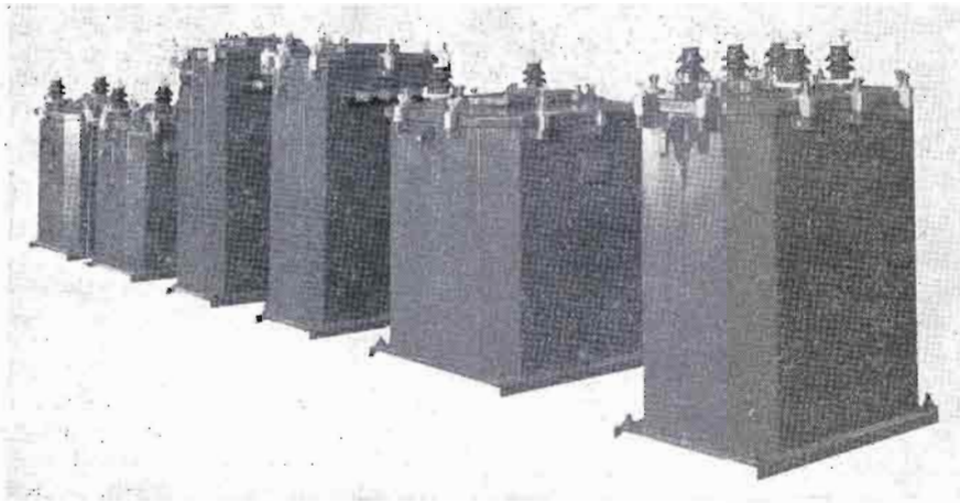
Heavy oil filled power-modulation components provide dual power supplies for both power amplifier and modulator.
