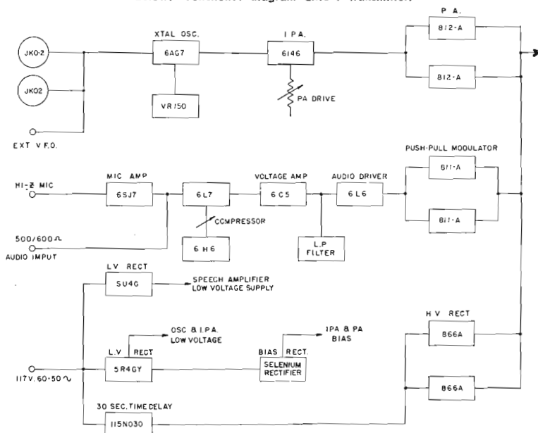
Below: Functional diagram CMG-1 transmitter.
