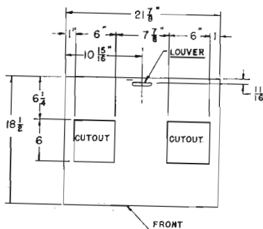
BASE DIMENSIONS, RAK2 RACK
