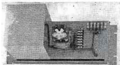
Rear of M-5295 rack mount motor driven variable transformer unit. M-5314, 2 KVA model is identical. Rack space is only 7"x19" or total for M-5294 electronic regulator and 1 or 2 KVA variable transformer unit is only 12¼" x 19" of rack space.
