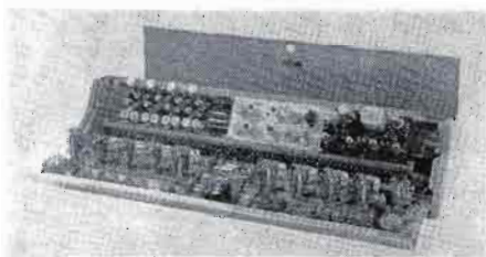
Right: Adding to serviceability, the entire amplifier framework hinges up. In this way, every under chassis connection may be instantly reached. Easily kept clean too.
