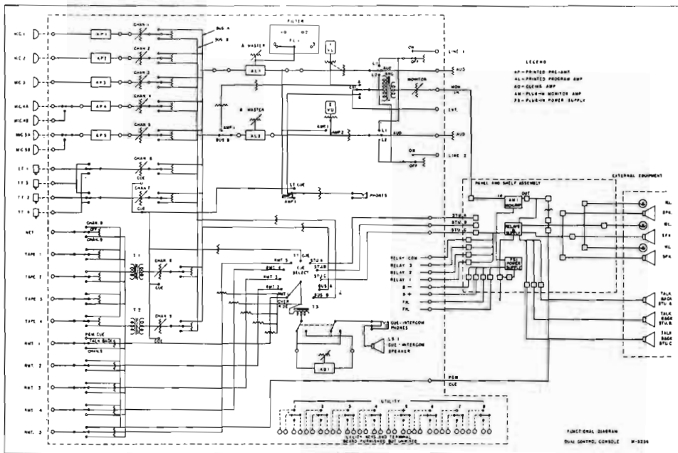
Functional Diagram M-5236 Dualux Speech Input Console.
