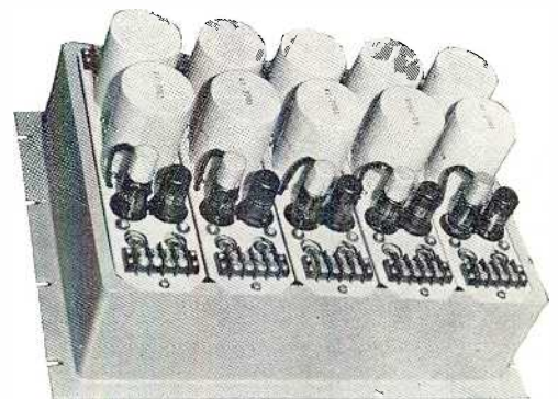
Figure E—Illustrates mounting five SA-70 preamplifiers on an SA-800 housing. This is the space saving and efficient way to mount Gates SA preamplifiers.
