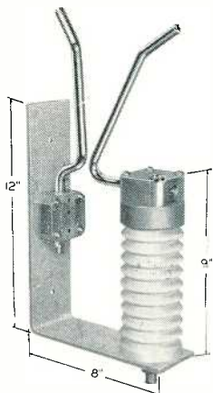
Horn gap assembly. Cat. M-3322
