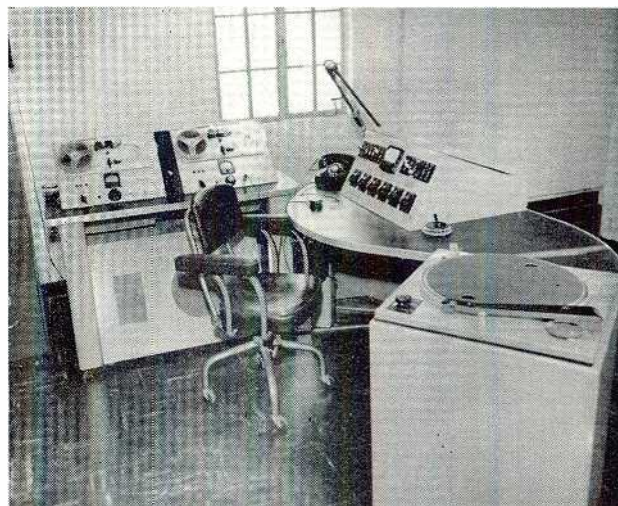
Below, to the left, 52-CS studioette in mobile radio studio supplied to the United States Government. Right, a typical studioette installation with tape recorders and turntables.
