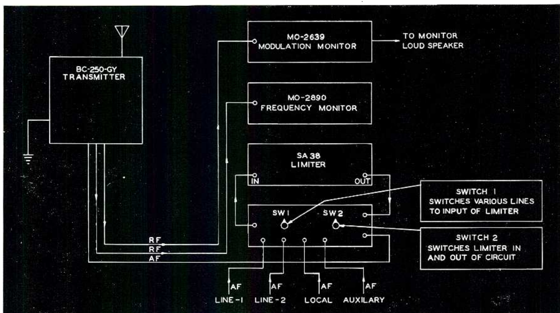
Block Diagram GY-48 Radio Station
