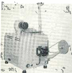
Complete projector, with 2" lens, lamps, tubes, one 1600' reel. Remote control unit for above. 3 point pedestal for floor mounting with 3" tilting adjustment. 2½" lens, speed F1.6. 3" lens, speed F1.6. 3½" lens, speed F1.6. 4" lens, speed F1.6. Shadow box for Image Orthicon (includes dual stand, image inverter).
