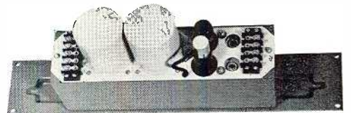
Figure D—Back view of SA-72 rack mount preamplifier. Note the shock mounting of tubes, test jacks for plate current, metering and isolation of input and output terminations.
