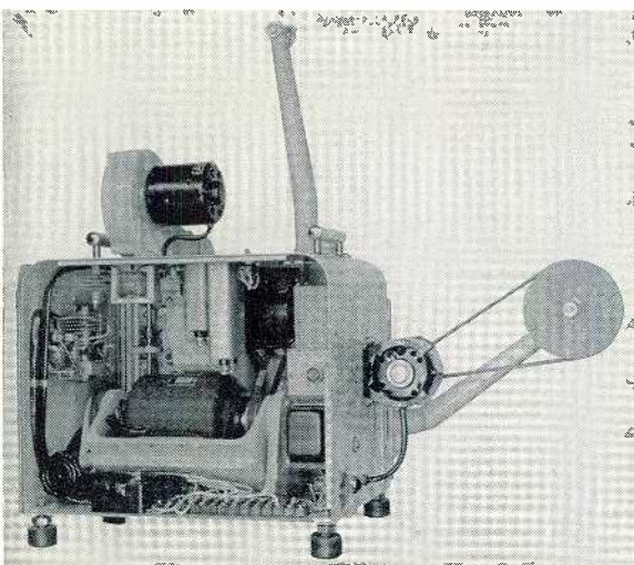
Dual stand with image inverter for Iconoscope projection. 4000' empty reel.
