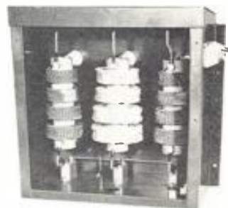
Below, the 24B Tower Choke assembly. Model 24A is identical, only having 2 section filter.
