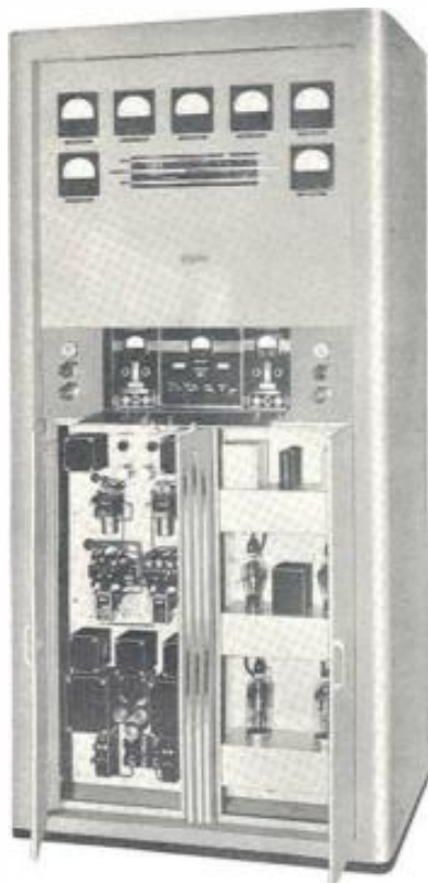
Above is the "Customaire" showing front doors open and wide accessibility to tubes and relays. At the right is a close-up of the frequency control unit section. On the center panel are the tuning controls for the entire transmitter.
