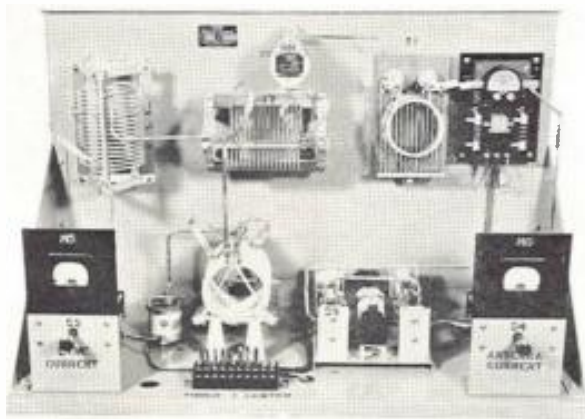
Indoor Shelf Type Coupler
