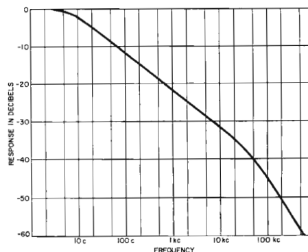
Response-frequency characteristic of the pink-noise filter.
