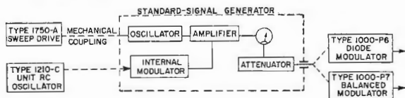
Figure 2. Modulation methods.
