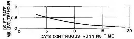
Typical drift after tubes are changed.
