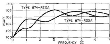
Average VSWR of Types 874-R20A and -R22A.
