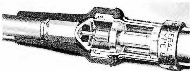
Basic Type 874 Connector (right) mated with Type 874 Cable Connector.
