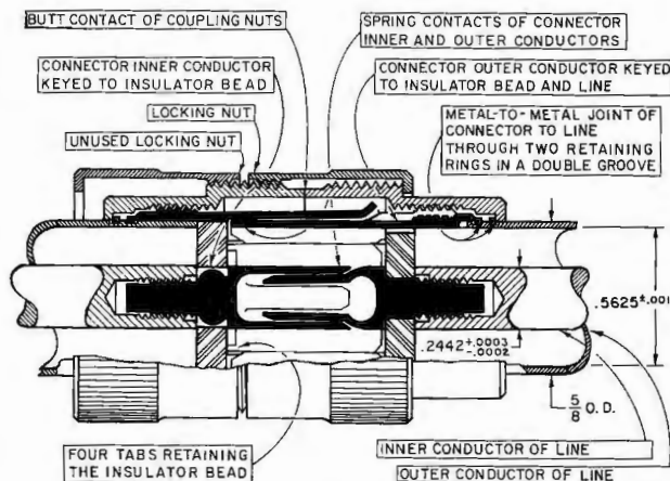
Section view of Type 874 locking connectors.
