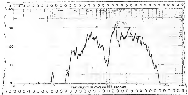
Plot of frequency response of a public-address system made on the graphic level recorder driving the frequency dial of the beat-frequency audio generator.
