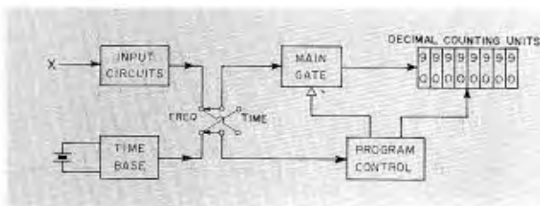
Figure 5. Elementary block diagram of a digital frequency meter (counter).
