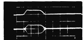
(Left) Amplitude-modulation characteristic at 900 Mc. Peak rf output is 10 millivolts; rf input, 50 millivolts. (Right) Oscilloscope showing modulation pulse and rf output pulse. Pulse duration is 0.25 \mu sec with 0.05- \mu sec rise time. Carrier frequency is 60 Mc. Scale is 0.1 \mu sec per horizontal division.
