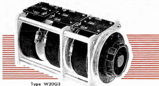
Type W20G3 (uncased) 3-gang model.
