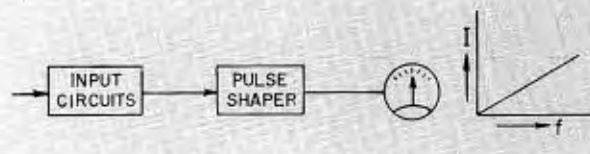
Figure 4. Elementary block diagram of an analog frequency meter.
