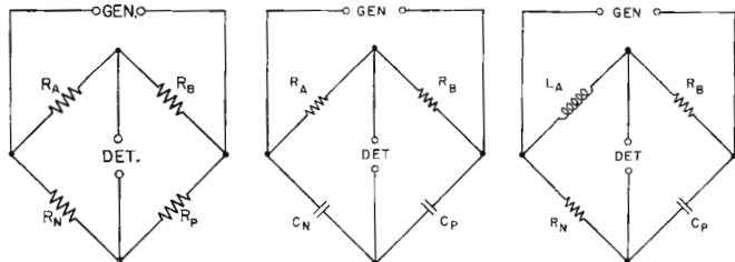
Figure 1. The general Wheatstone bridge circuit.
