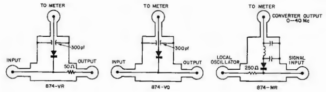
Schematic diagram of Types 874-VR, 874-VQ, and 874-MR.
