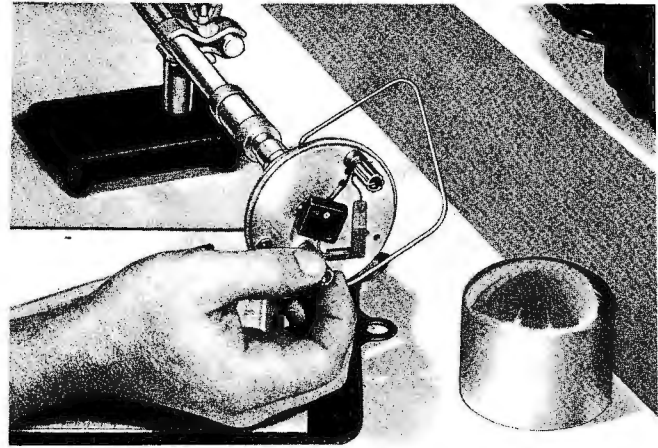
The Type 874-ML Component Mount is shown here attached to the Type 874-LK20L Constant-Impedance Adjustable Line. These useful accessories plug easily into the Admittance Meter. Also shown is the Type 874-Z Stand, which provides support.
