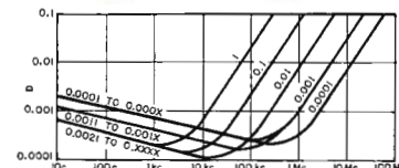
(Left) Change in capacitance as a function of frequency. These changes are referred to the values which the capacitors would have if there were neither interfacial polarization nor series inductance. The 1-kc value on the plot should be used as a basis of reference in estimating frequency errors. (Right) Dissipation factor as a function of frequency.
