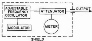
Figure 1. Elements of a standard-signal generator.
