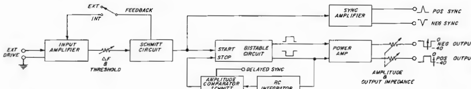
Block diagram of the circuit system.
