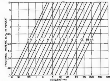
Figure 2. Percent increase in inductance versus frequency.
