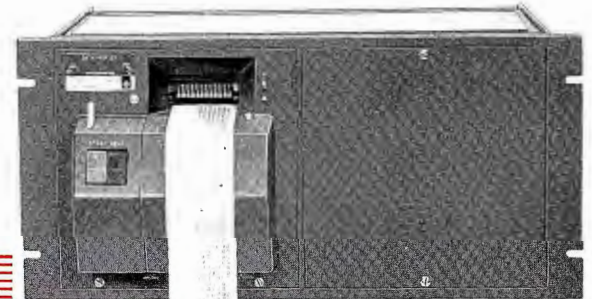
Type 1137-A Data Printer, Rack Mounted
