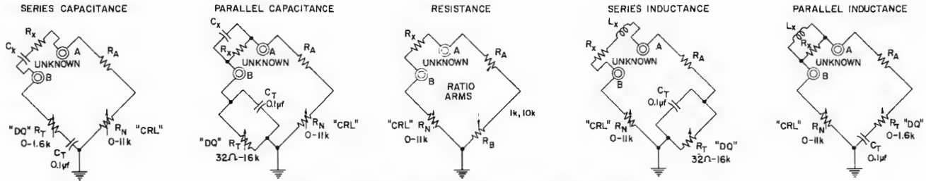
Schematic diagrams of the five circuits used in the bridge.
