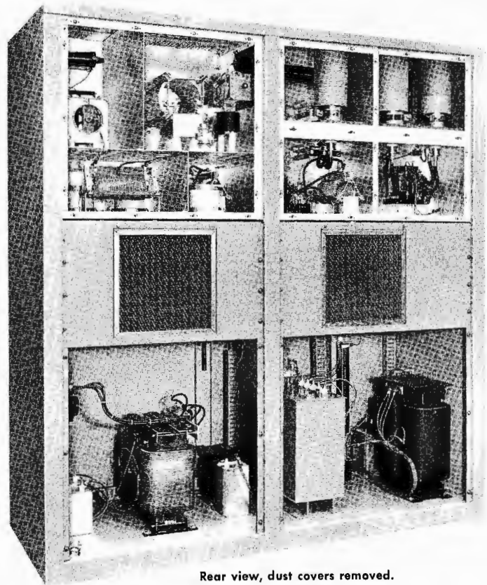
Rear view, dust covers removed.
