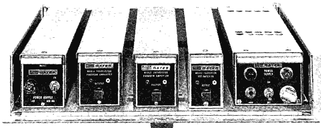
Above: M-6689 panel and shelf assembly, showing several "6300" series Solid-Statesman units. This assembly requires only 3½" x 19" of rack space.
