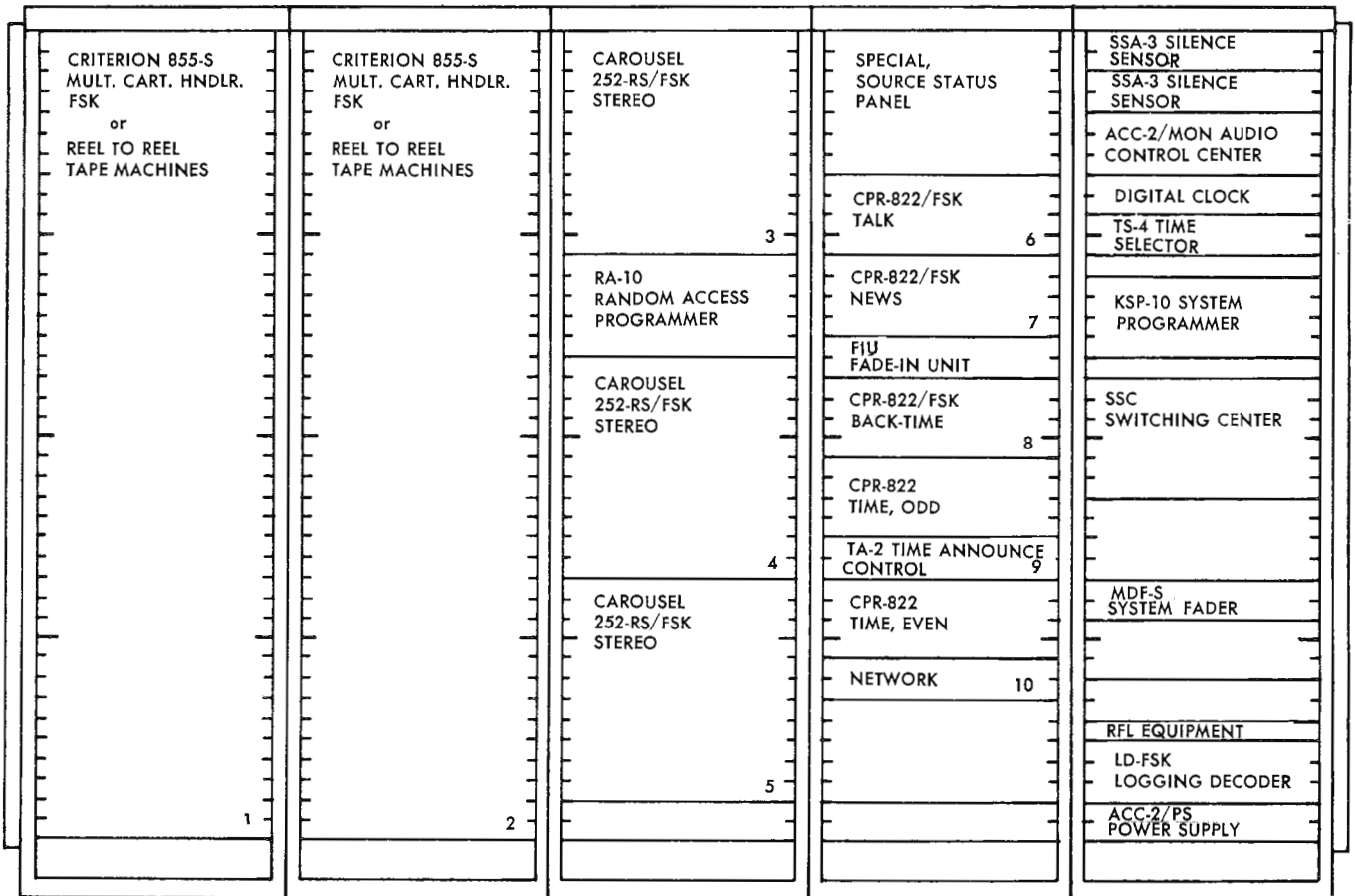
RACK LAYOUT
