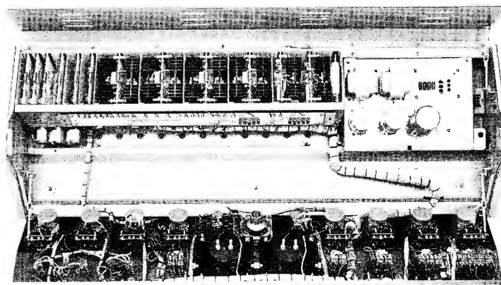
Hinged cabinet cover and front panel provide full accessibility to all components of the Dualux 80.
