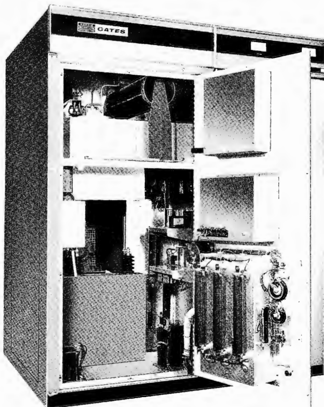
Modulator cubicle, showing modulator, modulator driver, 70 kHz filter, power supplies and control.
