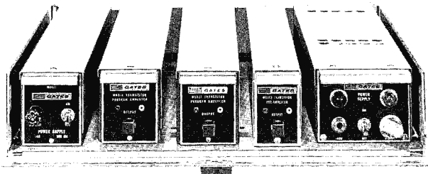
Above: M-6689 panel and shelf assembly, showing several "6300" series Solid-Statemans units. This assembly requires only 3½" x 19" of rack space.
