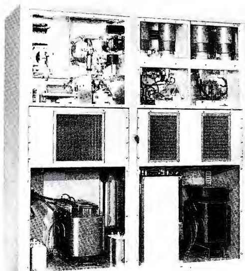
Rear view, interior.
