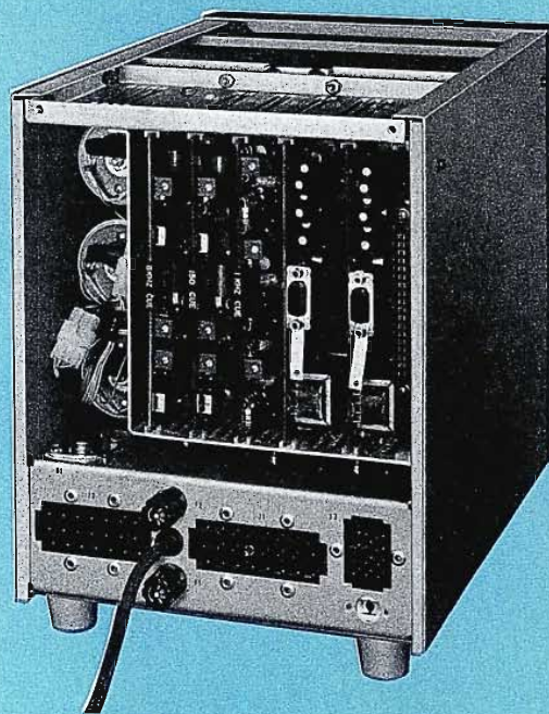
Two Criterion 90-3's may be mounted side by side in a standard rack to provide six playback units in a rack space that will hold only two regular size playbacks.
