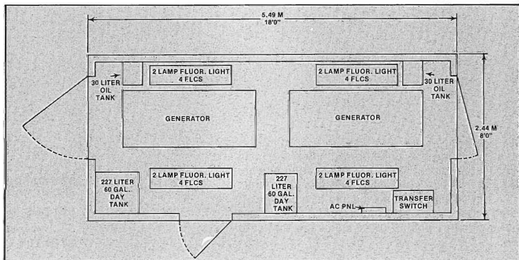
Generator shelter (optional)
