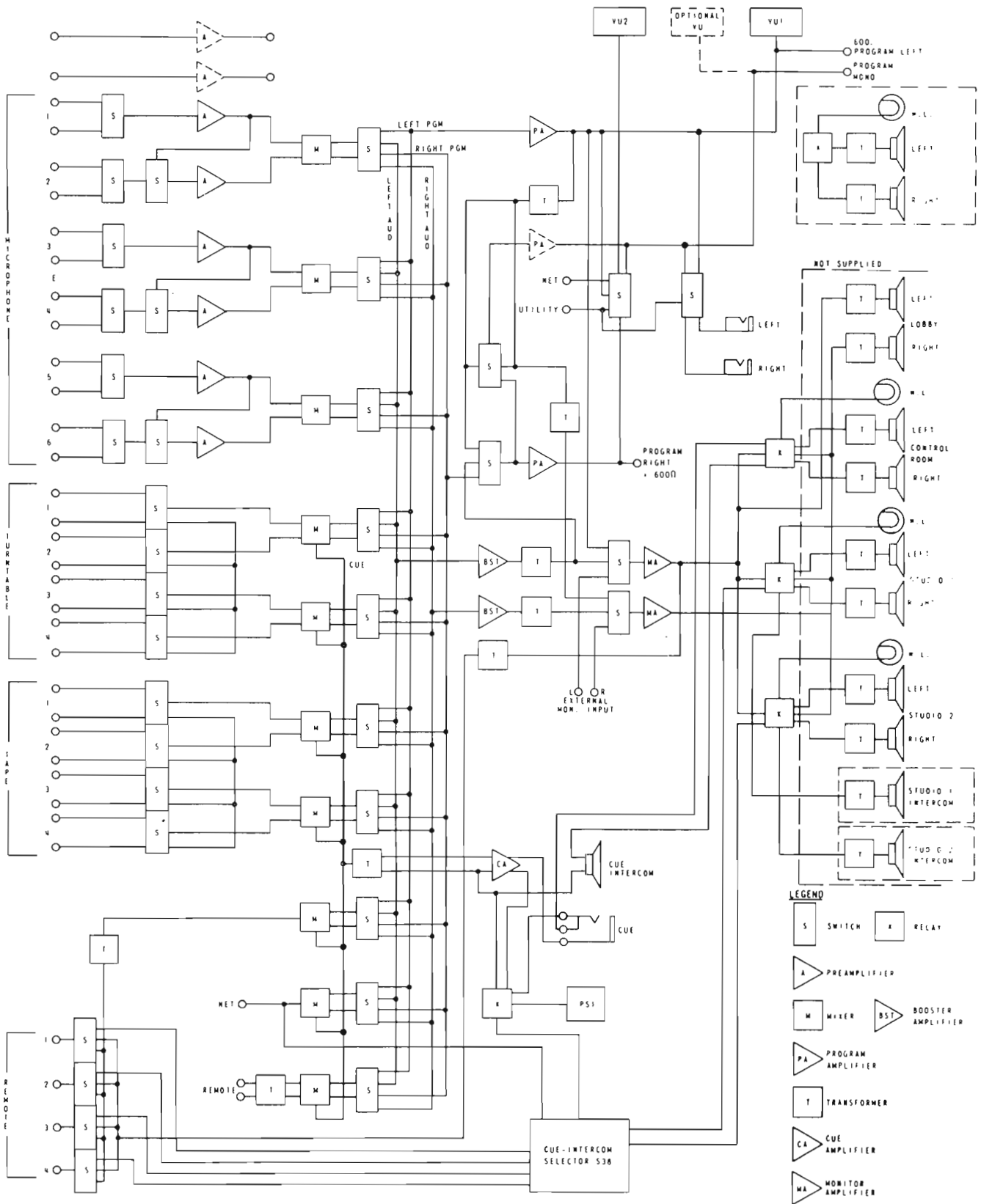
BLOCK DIAGRAM
