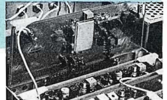
The MCP-1U visual exciter/modulator (above) is a solid-state, independent self-contained "on-channel" signal source. Harris' advanced TSB filter (right) is mounted on a PC board in the visual exciter, and measures only 1½ inches square.
