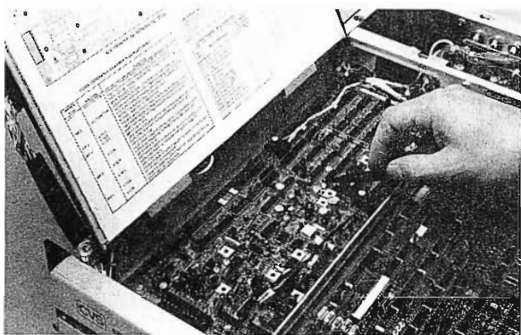
The unique "flat-pack" design of the CVS-517 makes all components easily accessible for fast, easy maintenance, testing and troubleshooting.
