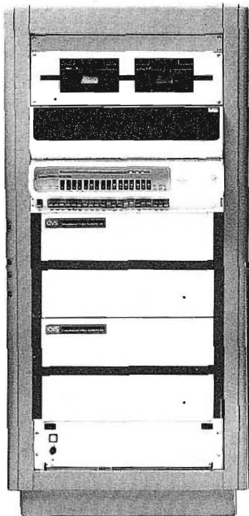
Figure 4: All EPIC components, except the compact keyboard, can be housed in a single 19" rack.
