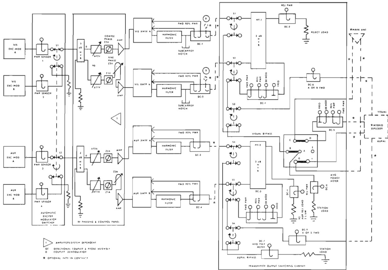
RF FLOW BTD-36L2 WITH HYBRID DIPLEXER
