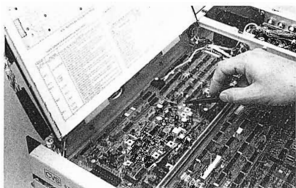
The unique "flat-pack" design of the CVS 516 makes all components easily accessible for fast, easy maintenance, testing and troubleshooting.
