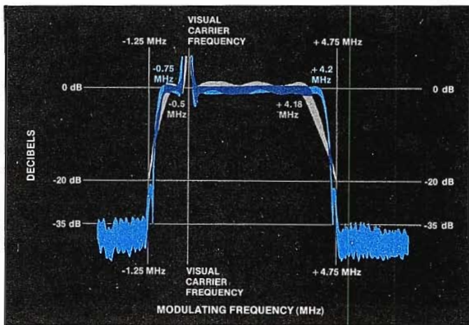
Sideband response of MCP-1U exciter (in blue) showing improvement over typical response of older exciters (shown in gray).
