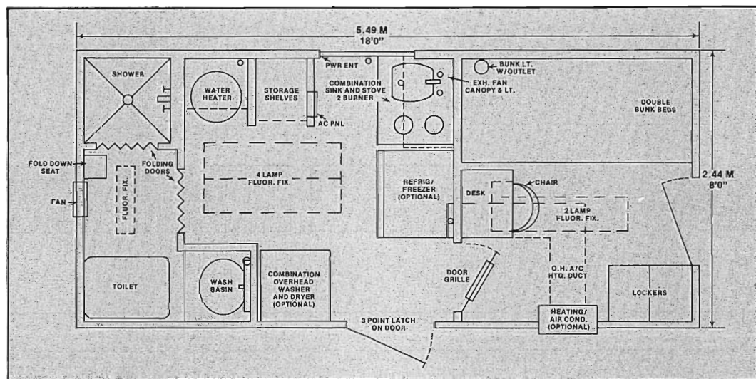
Living shelter (optional)
