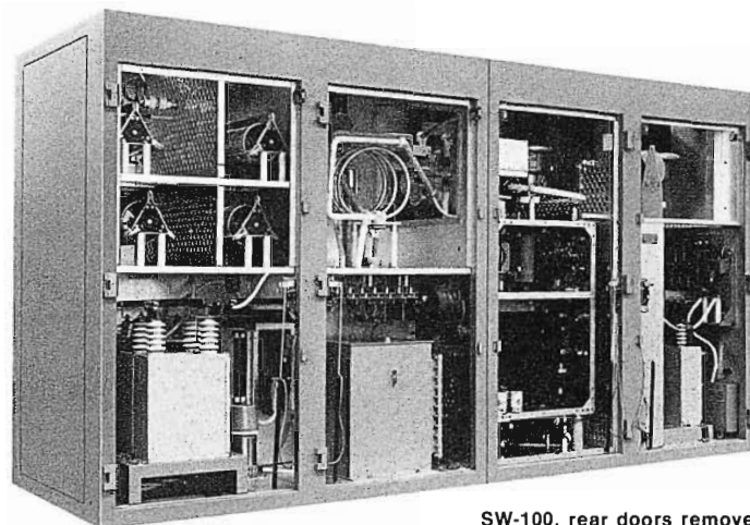
SW-100, rear doors removed (Heat exchanger not shown)
