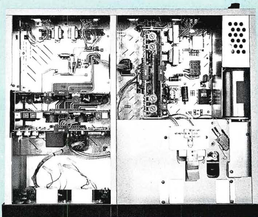
Criterion 90-2 record/playback, top view, cover off, showing modular construction and easy component access.
