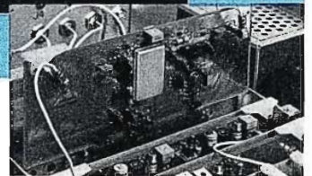
The MCP-1V visual exciter/modulator (above) is a solid-state, independent, self-contained "on-channel" signal source. Harris' advanced TSB filter (right) is mounted on a PC board in the visual exciter, and measures only 1½ square inches.
