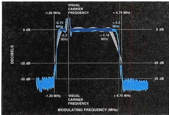
Sideband response of MCP-1V exciter (in blue) showing improvement over typical response of older exciters (shown in gray).
