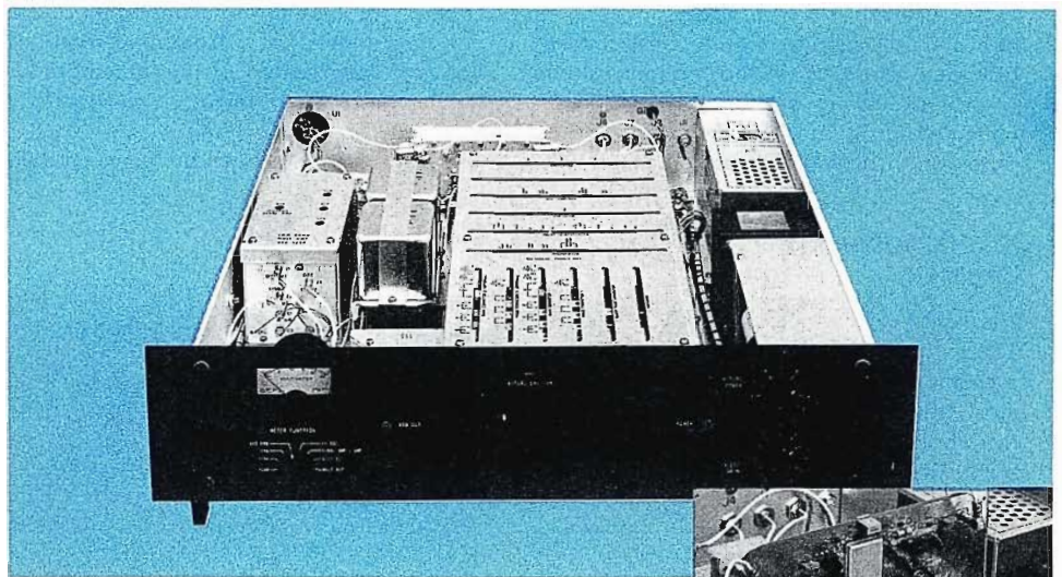
The MCP-1V visual exciter/modulator (above) is a solid-state, independent, self-contained "on-channel" signal source. Harris' advanced TSB filter (right) is mounted on a PC board in the visual exciter, and measures only 1½ square inches.
