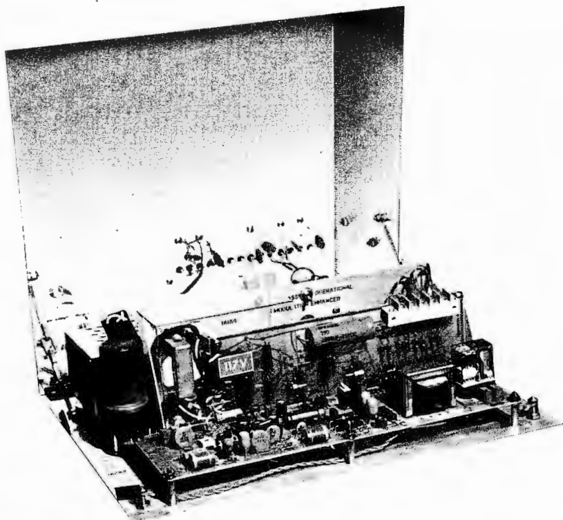
Low level Pulse Duration Modulator chassis, showing power control and audio input/control.
