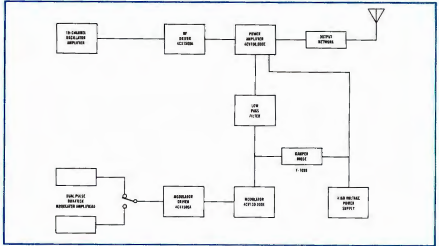
SW-100A BLOCK DIAGRAM
