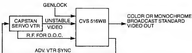
Capstan servo VTR operation.
