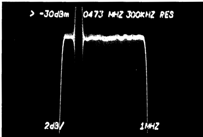
Sideband response of MCP-2U exciter showing passband (2 dB/cm) frequency response.
