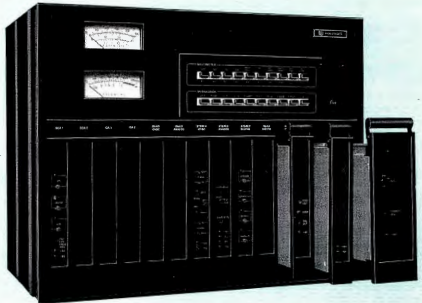
The high-performance MS-15 Exciter, above, and the FM-100K Amplifier utilize modular construction throughout for ease of service
