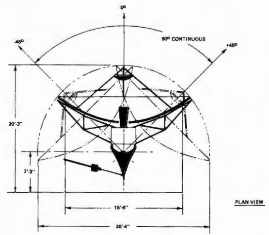
6.1-Meter Antenna with Kingpost Pedestal
