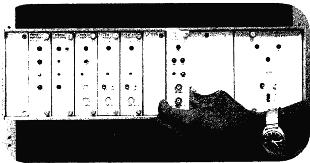
FIGURE 2. FV40 Receive Equipment Shelf equipped with (left to right): blank covering one unoccupied space, Video/Subcarrier Separator (one space), System Monitor for pilot and noise (one space), Clamper Amplifier (one space), two FM Channel Receiver units (one space each), blank covering one unoccupied space, one AM Channel Receiver unit (one space), blank covering two unoccupied spaces, and a DC -48/-21V Converter unit (three spaces).
