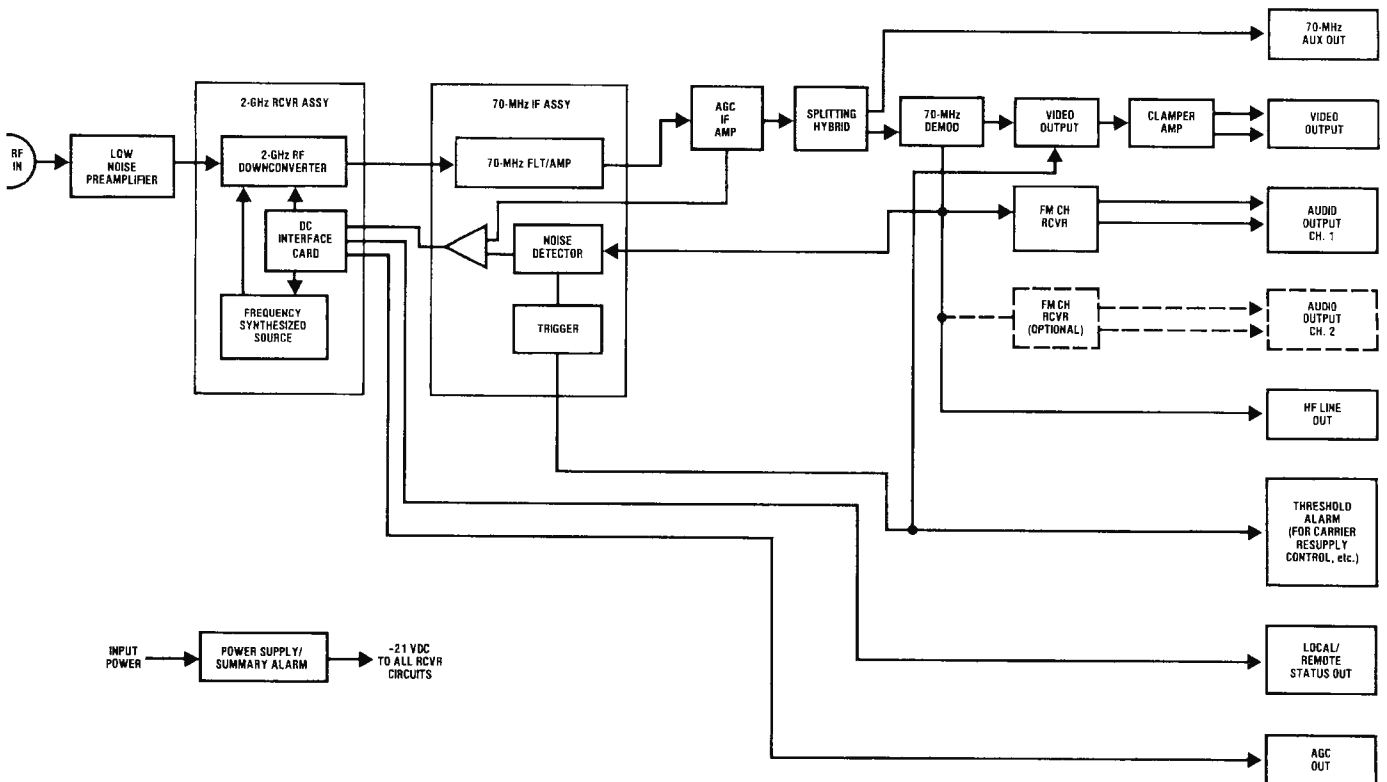
Simplified Block Diagram of Typical FV2CR Receiver Circuitry
