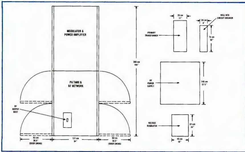
SW-100A FLOOR PLAN
