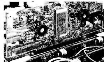
The MCP-2U visual exciter (above) is a solid-state, independent, self-contained "on-channel" signal source. Harris' advanced VIDEO SAW filter (right) is mounted on a PC board in the visual exciter, and measures only 2½ inches square.
