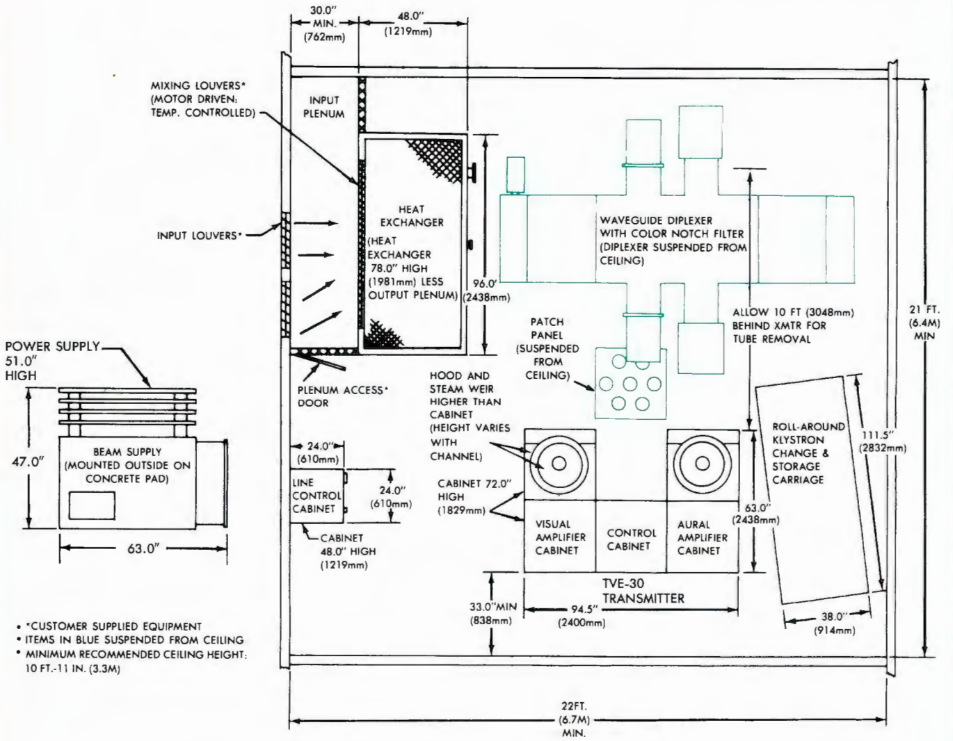
TYPICAL EQUIPMENT PLACEMENT TVE-30 TRANSMITTER
