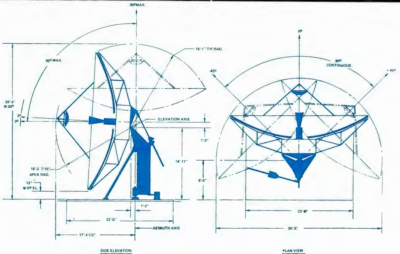
Harris 9-Meter Antenna Las Vegas, Nevada
