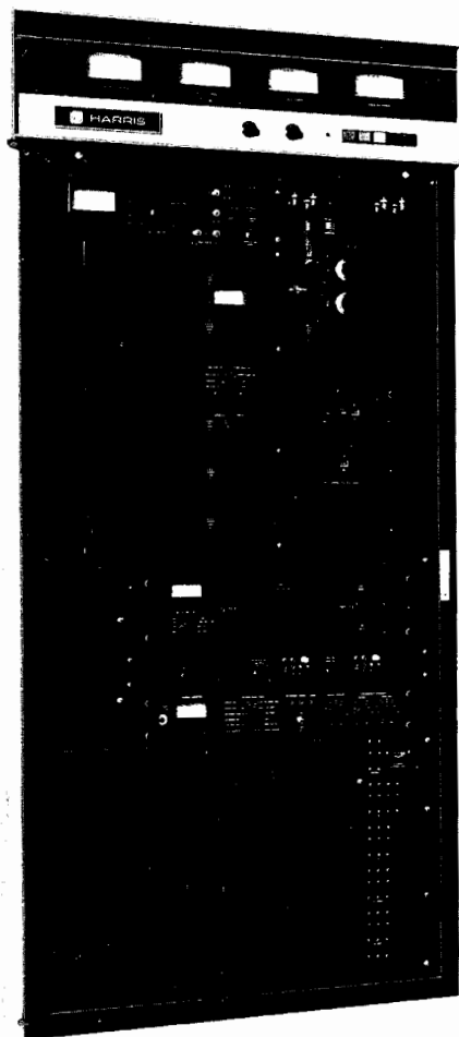
Ultra-linear driver cabinet with solid-state IPA
