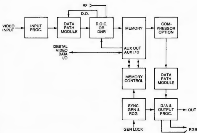
Figure 1: Basic Block Diagram HVS 630 Frame Synchronizer
