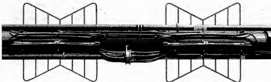
(Above) Channel 5, five-bay Batwing antenna. (At left) Batwing transmitting antenna junction box assembly.
