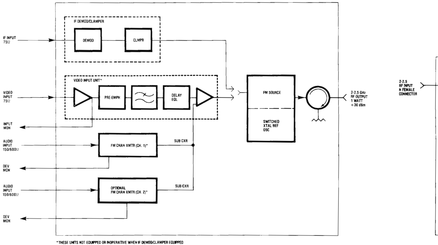
Simplified block diagram FV2/2.5MP transmitter
