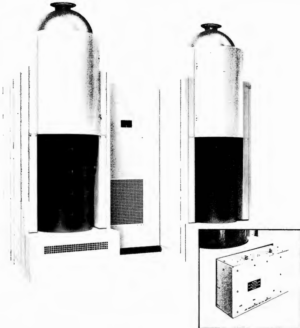
TVE-55, rear view. (Inset) Mod Anode Pulser.
