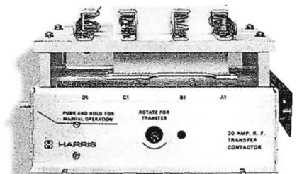
HS-4P 30 Amp RF Contactor
