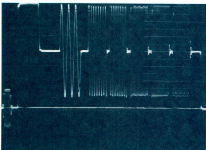
multiburst response
