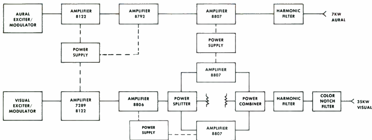
BT-35L2 BLOCK DIAGRAM
