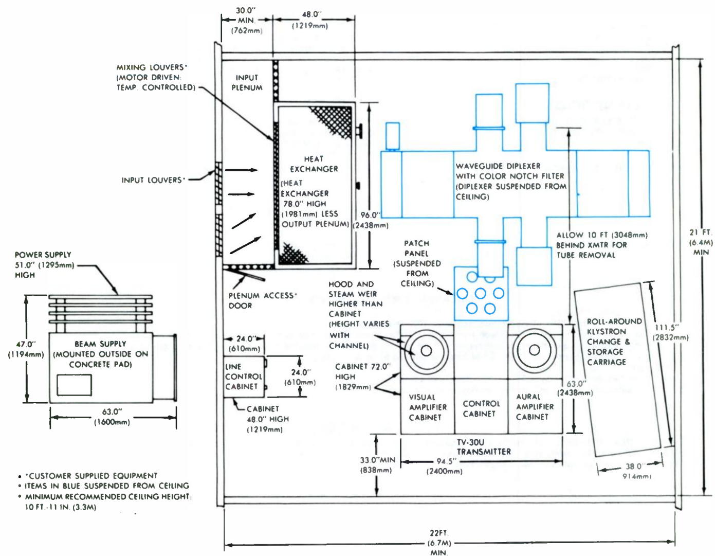
TYPICAL EQUIPMENT PLACEMENT TV-30U TRANSMITTER
