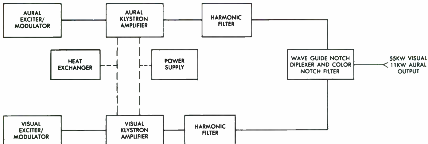
BLOCK DIAGRAM TV-55U
