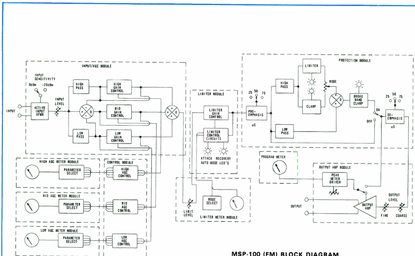
MSP-100 (FM) BLOCK DIAGRAM
