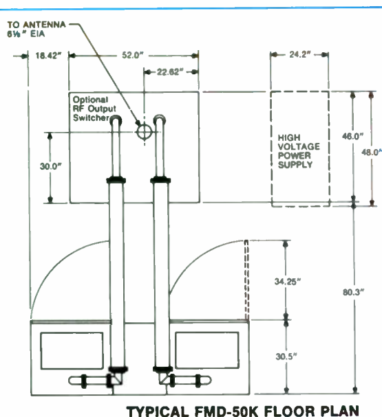
TYPICAL FMD-50K FLOOR PLAN
