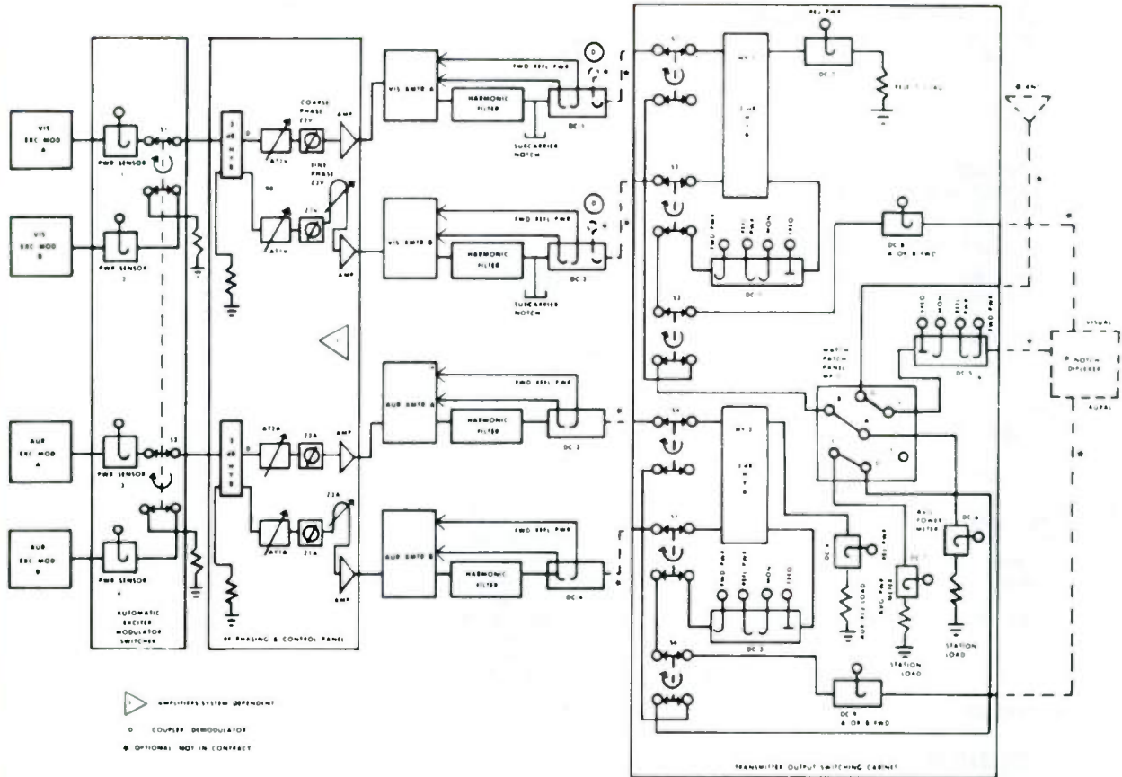
RF FLOW TVD-36H WITH NOTCH DIPLEXER
