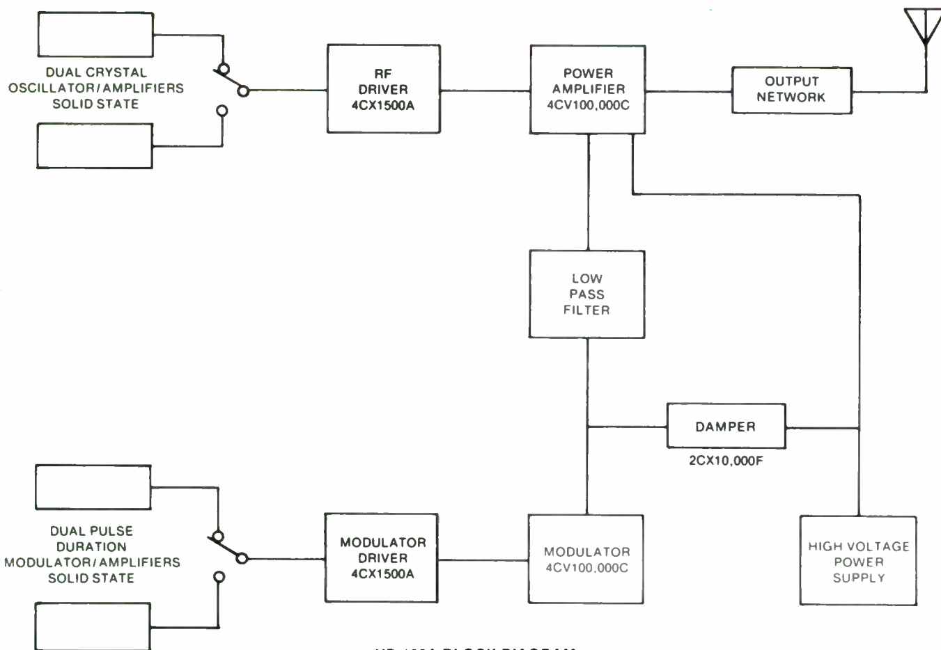
VP-100A BLOCK DIAGRAM
