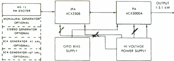
FM-5K BLOCK DIAGRAM
