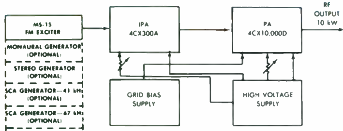
FM-10K BLOCK DIAGRAM
