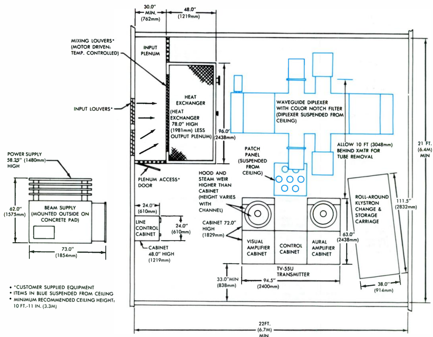
TYPICAL EQUIPMENT PLACEMENT TV-55U TRANSMITTER
