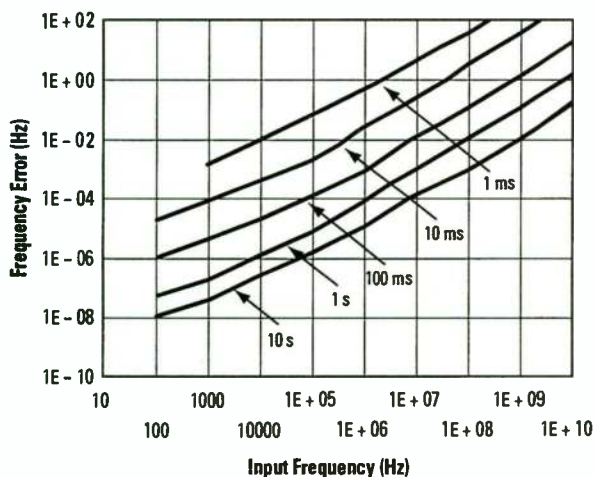
HP 53131A and 53181A – Worst Case RMS Resolution (Time or Digits Arming)
