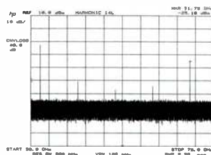
50 to 75 GHz Sweep Using HP 11974 Series Mixer
