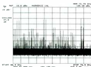
50 to 75 GHz Sweep Without Preselection
