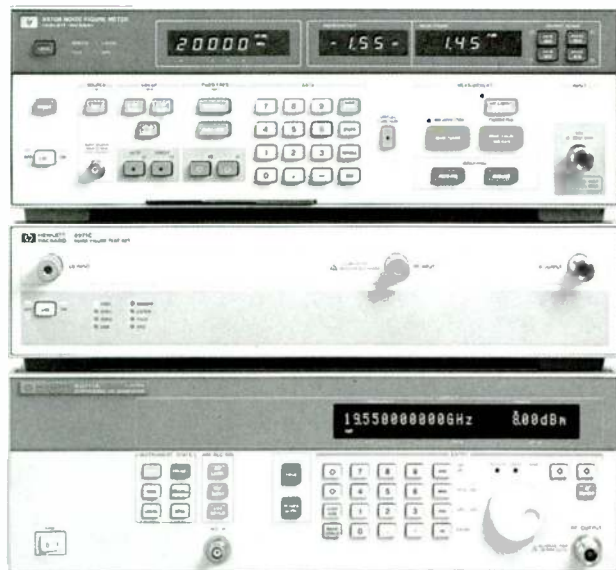
HP 8970S/V
