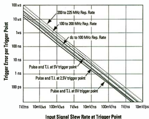
Trigger Level Timing Error (Level Setting Error and Input Hysteresis)
