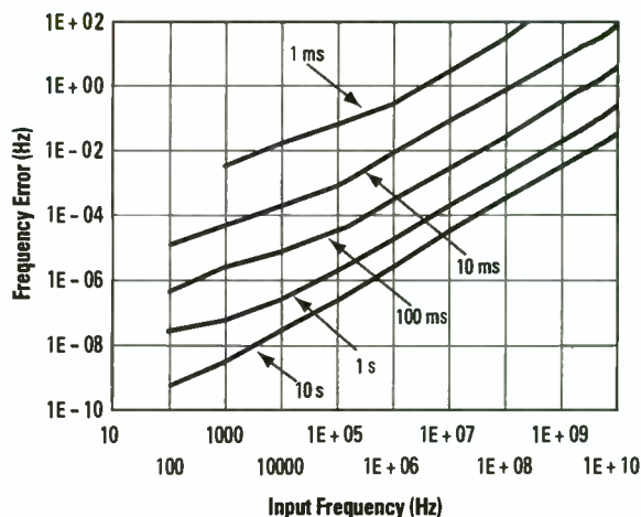
HP 53132A – Worst Case RMS Resolution (Time or Digits Arming)
