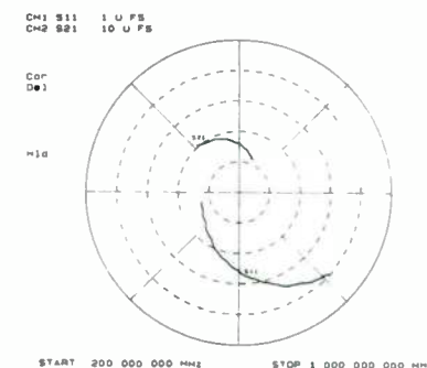
Simultaneous measurement of transistor S-parameters.
