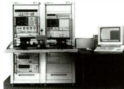
Customized system for cellular base station amplifier testing
