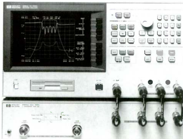
HP 8751A with HP 87511A
