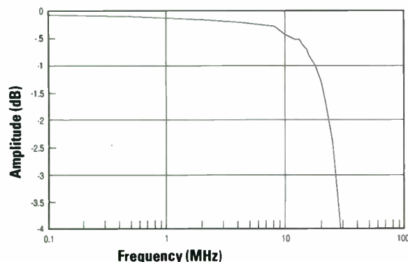
I/Q Bandwidth
