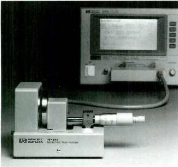
HP 16451B Dielectric Test Fixture
