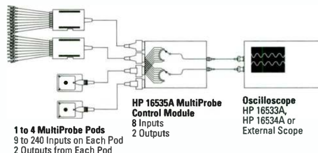
HP MultiProbe System block diagram
