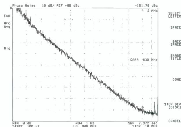
VCO phase noise measurement
