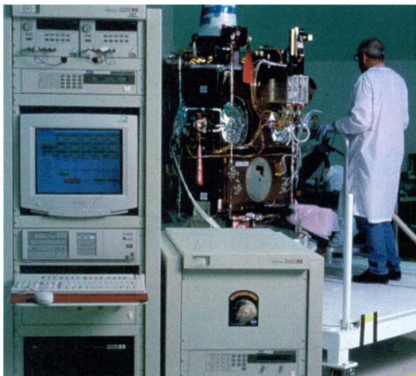
HP Lunar Prospector Electrical Test Set (LPETS) at Lockheed Martin site, performing test during Lunar Prospector manufacturing phase.
