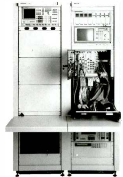
VXI-based manufacturing test system—racking and cabling to high-density, quick disconnect DUT fixture interface
