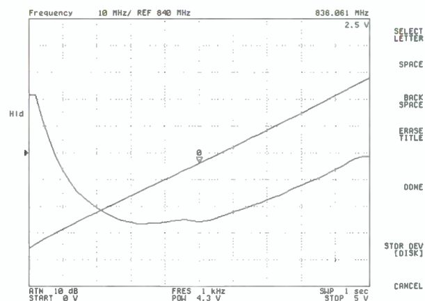
VCO tuning characteristics (frequency/tuning sensitivity)
