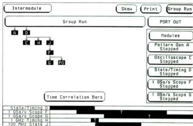
Powerful cross-domain triggering helps you pinpoint problems that display symptoms in one domain but are caused by activity from another domain.
