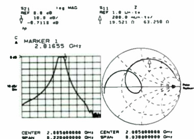
Simultaneous measurement of transmission response and passband reflection coefficient.
