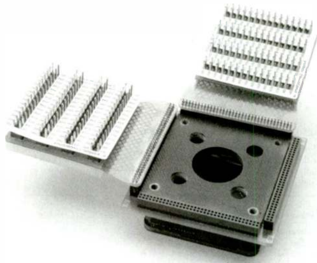
Locator base probing system with 1/4 flex adapters.
