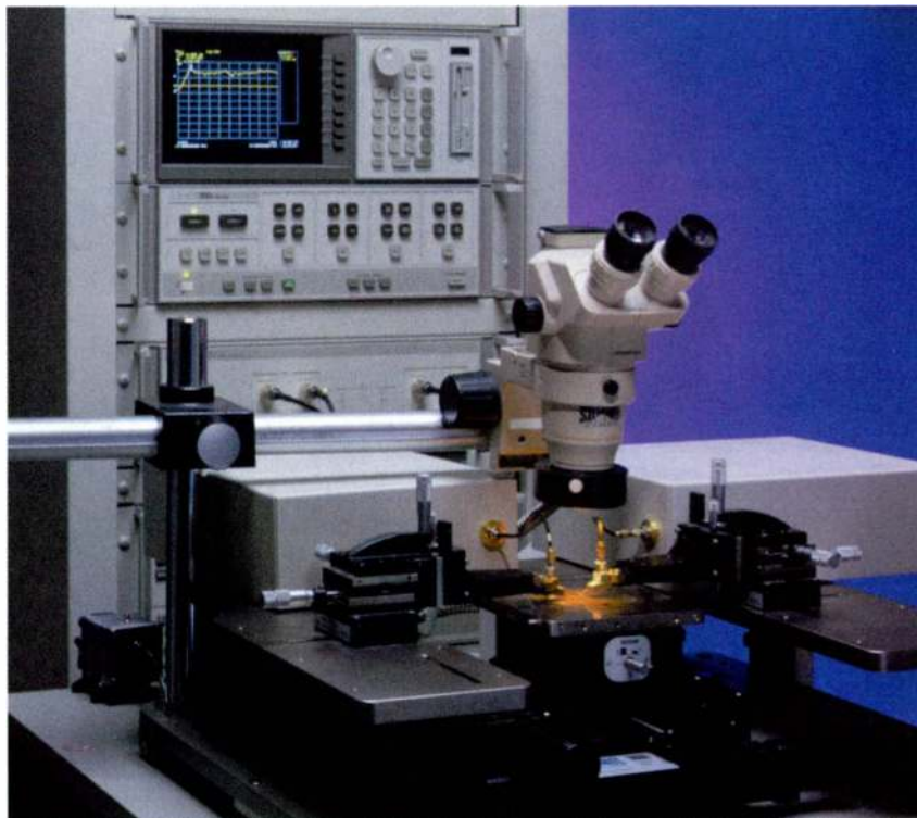
Convenient on-wafer measurements with the HP 8510XF using a Cascade Microtech wafer probing station and APC 110 probes.
