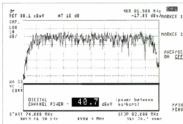
Digital Carrier Power Measurement on HP 8591C
