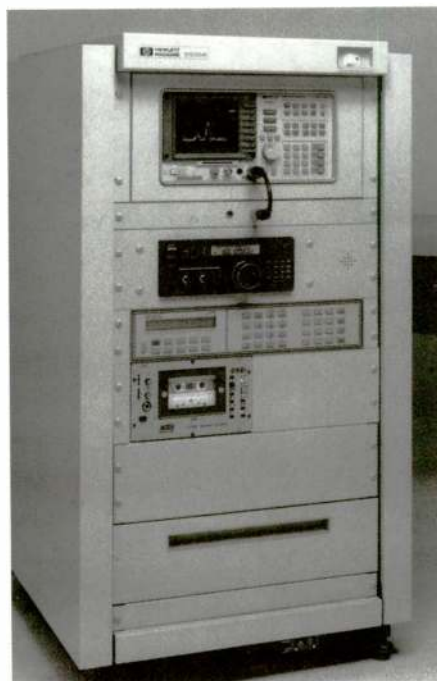
HP E4900B-003 System (pull-out tray with laptop PC included in rack)
