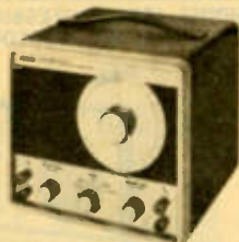
MODEL 379 SOLID-STATE SINE/SQ WAVE GENERATOR KIT
