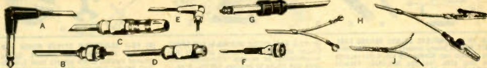
RCA TYPE PHONO PLUG TO VARIOUS CONNECTIONS All Cables shielded except unshielded parallel cable. Wt. 6 oz.
