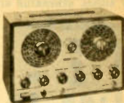
MODEL 369K TV-FM SWEEP MARKED GENERATOR KIT
