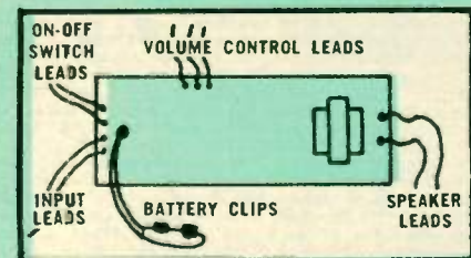
ON-OFF SWITCH LEADS VOLUME CONTROL LEADS INPUT LEADS BATTERY CLIPS SPEAKER LEADS
