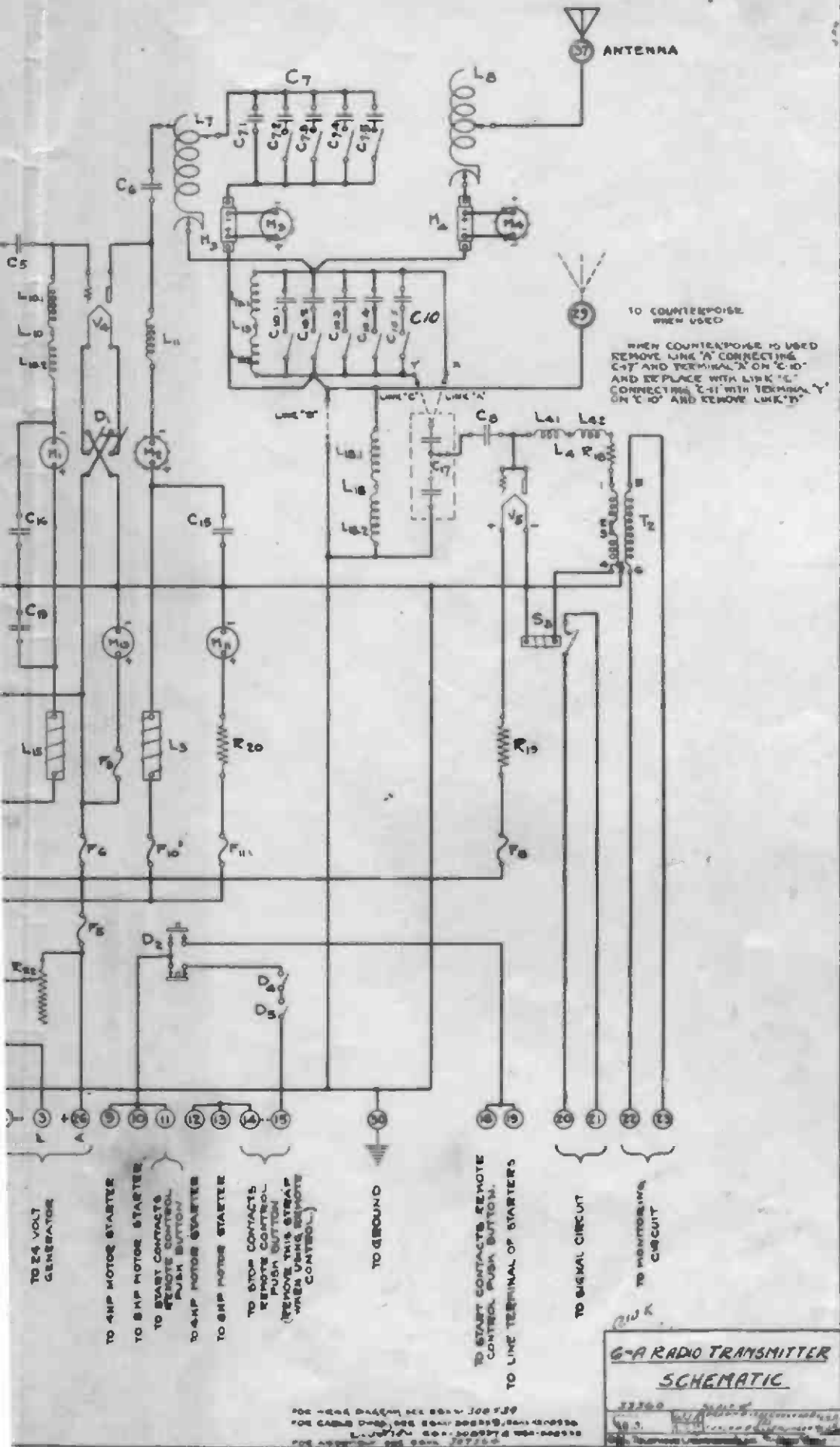
6-A RADIO TRANSMITTER SCHEMATIC ISSUE 7—ESR-307849
