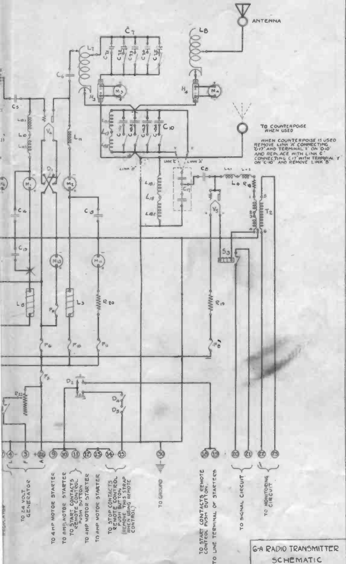
6-A RADIO TRANSMITTER SCHEMATIC ISSUE 4—ESR-308840
